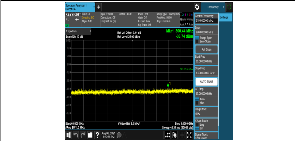
Band2-5MHz-QPSK-18900-6-0-Low-30-1000--33.74-PASS
