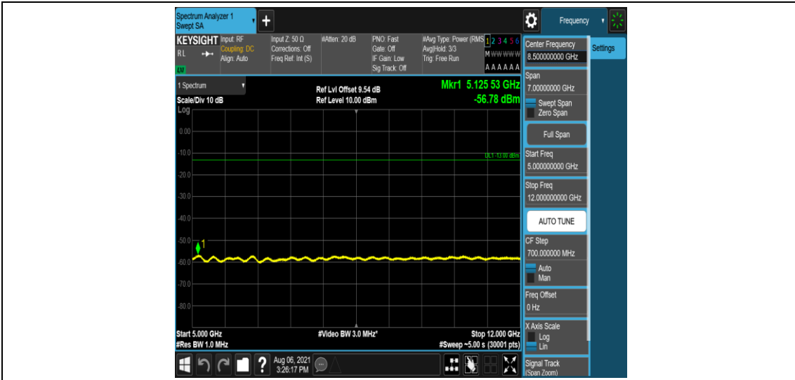
Band2-5MHz-QPSK-19175-1-5-Low-5000-12000--56.78-PASS
