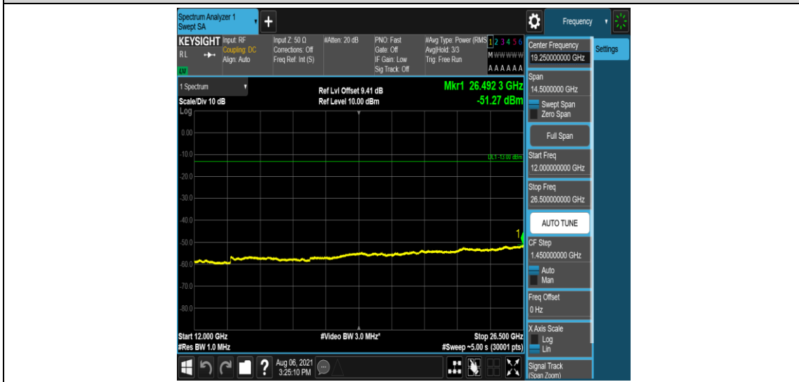
Band2-5MHz-16QAM-18900-6-0-Low-12000-26500--51.27-PASS
