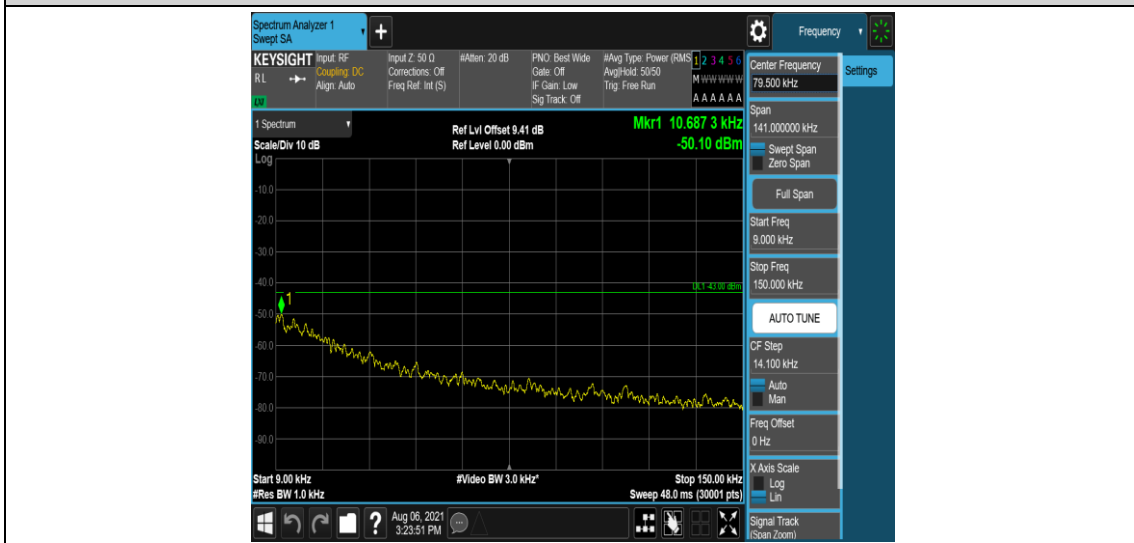
Band2-5MHz-16QAM-18900-6-0-Low-0.009-0.15--50.1-PASS
