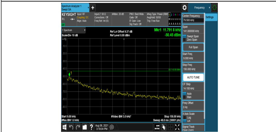
Band2-5MHz-16QAM-18625-6-0-Low-0.009-0.15--50.45-PASS
