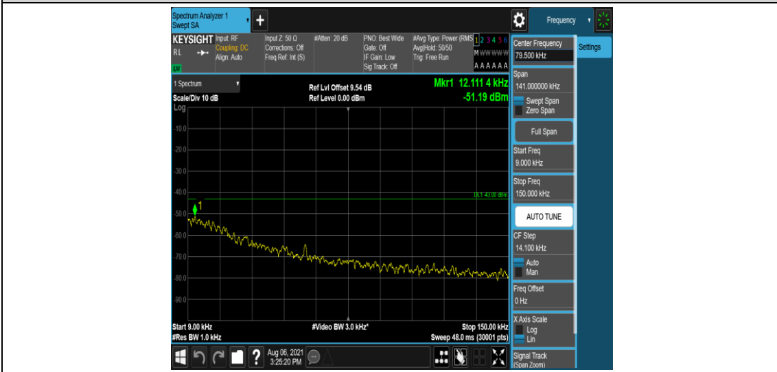
Band2-5MHz-QPSK-19175-1-5-Low-0.009-0.15--51.2-PASS
