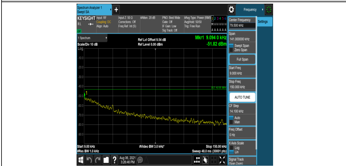
Band2-5MHz-16QAM-19175-1-5-Low-0.009-0.15--51.82-PASS
