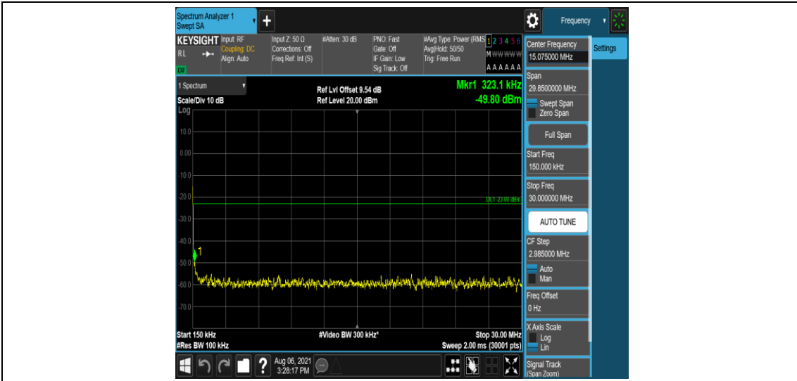
Band2-5MHz-QPSK-19175-6-0-Low-0.15-30--49.81-PASS
