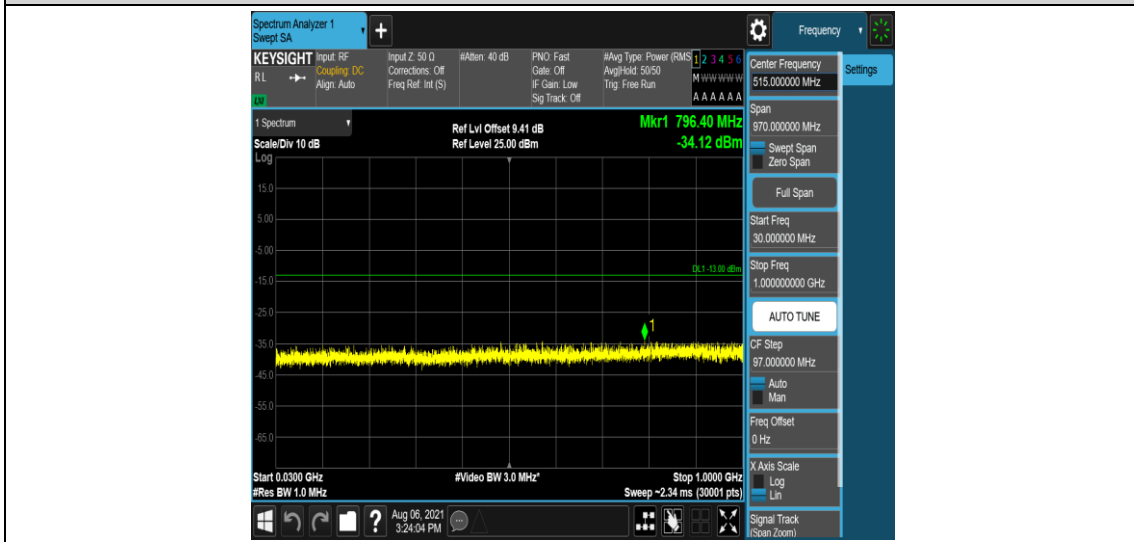
Band2-5MHz-16QAM-18900-6-0-Low-30-1000--34.12-PASS
