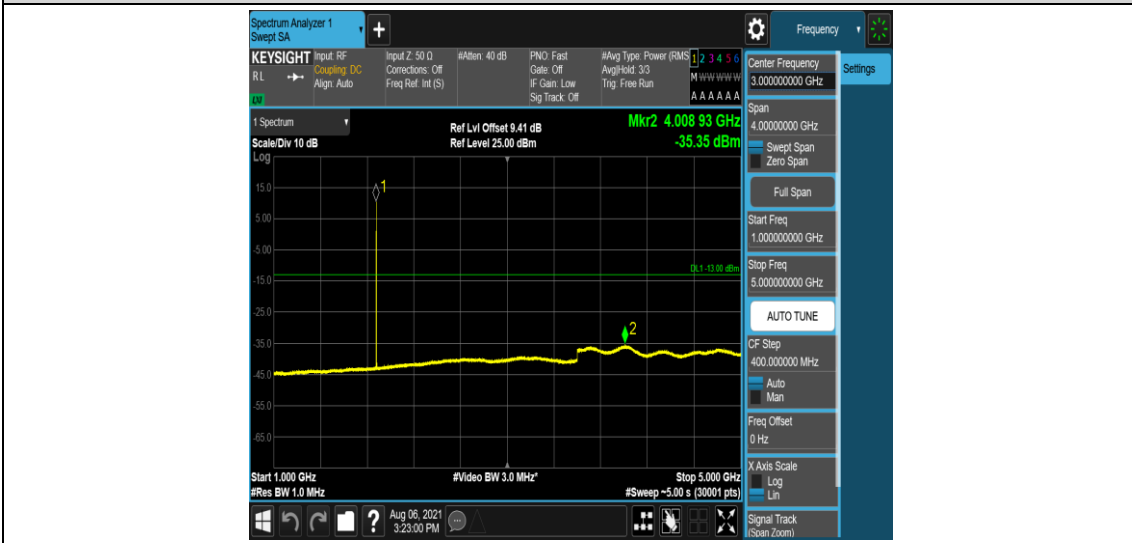
Band2-5MHz-QPSK-18900-6-0-Low-1000-5000--35.35-PASS
