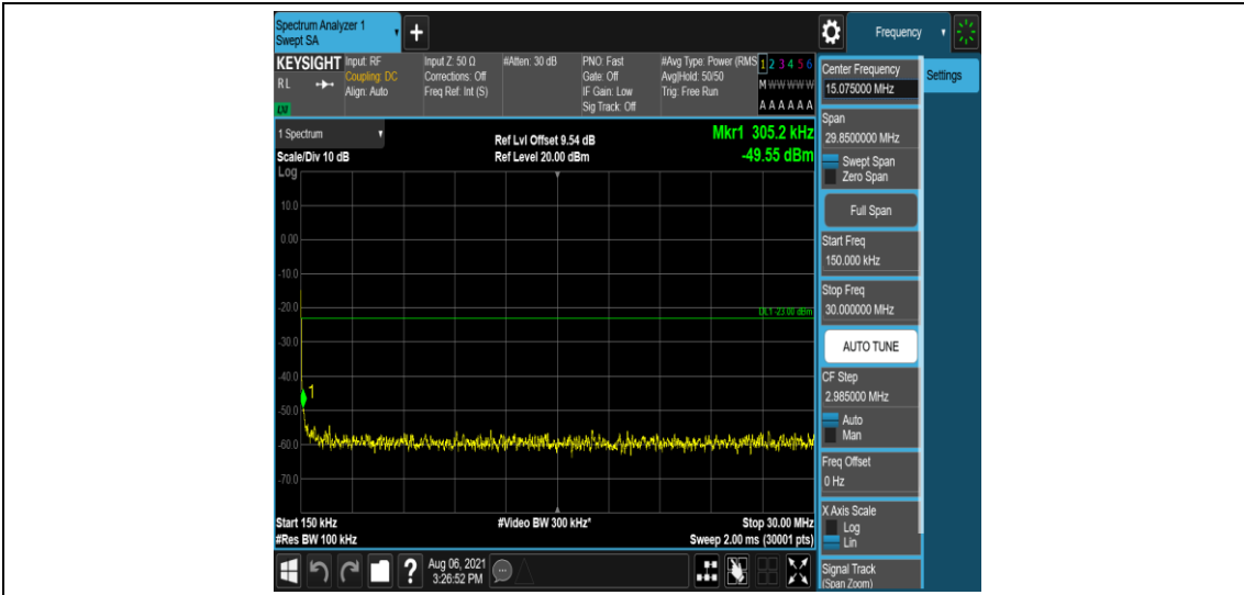
Band2-5MHz-16QAM-19175-1-5-Low-0.15-30--49.55-PASS
