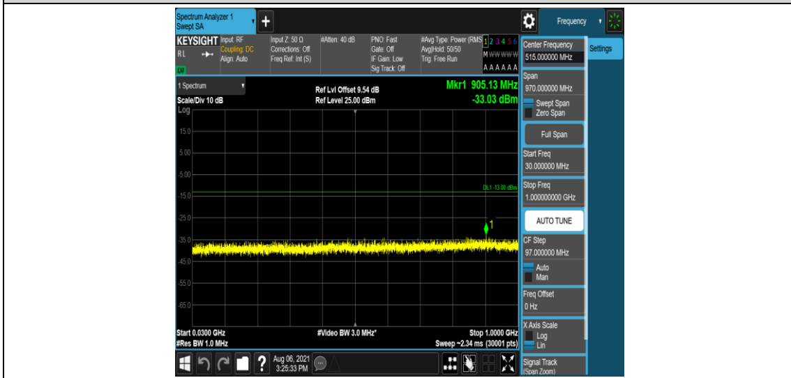
Band2-5MHz-QPSK-19175-1-5-Low-30-1000--33.03-PASS
