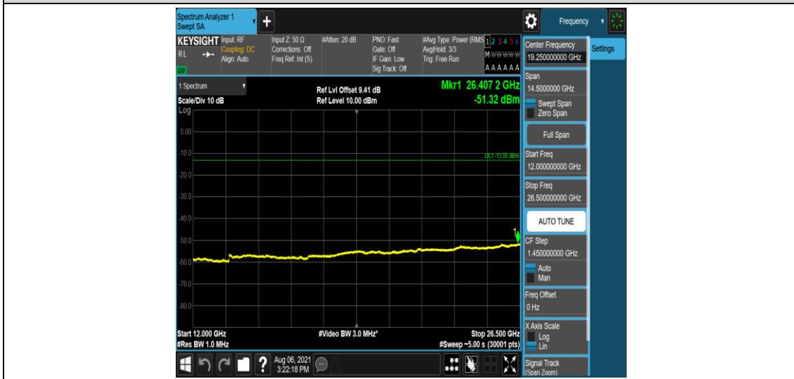
Band2-5MHz-16QAM-18900-1-0-Low-12000-26500--51.32-PASS
