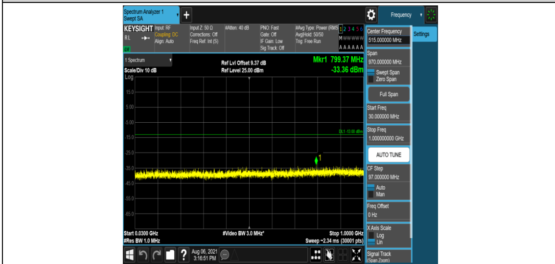
Band2-5MHz-QPSK-18625-6-0-Low-30-1000--33.36-PASS
