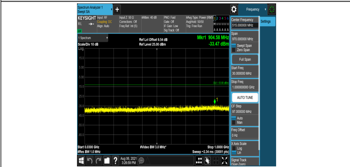
Band2-5MHz-16QAM-19175-1-5-Low-30-1000--33.47-PASS
