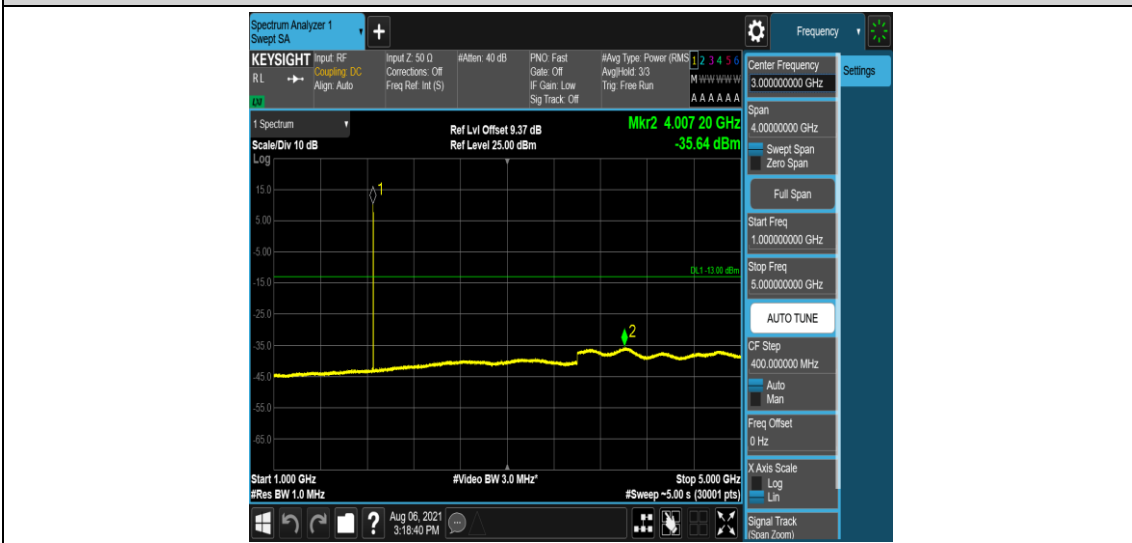
Band2-5MHz-16QAM-18625-6-0-Low-1000-5000--35.64-PASS
