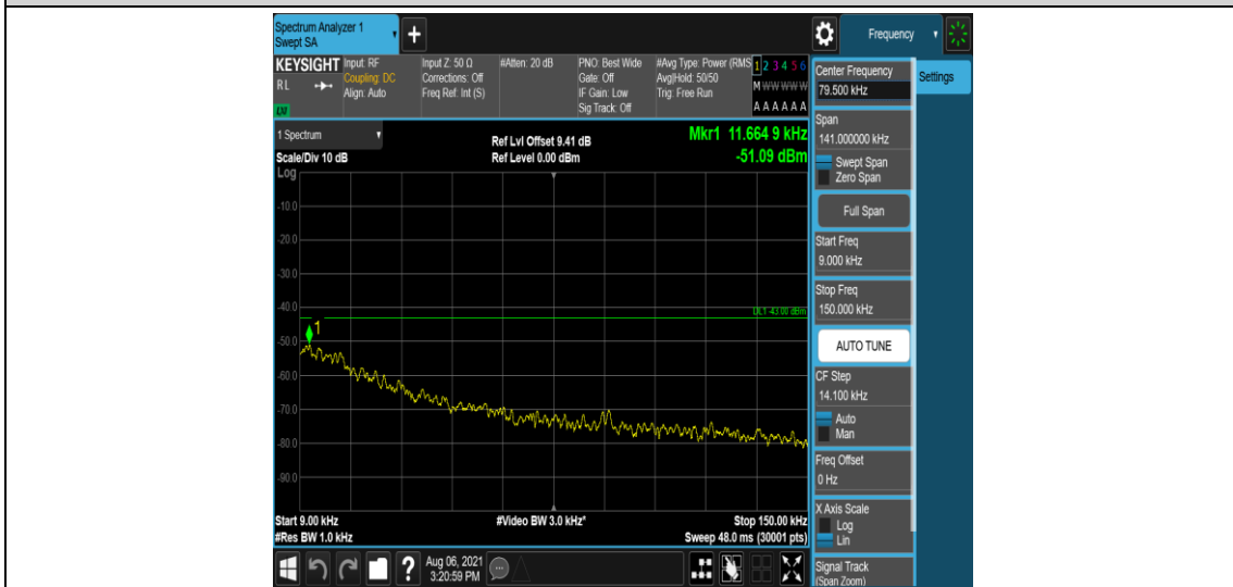
Band2-5MHz-16QAM-18900-1-0-Low-0.009-0.15--51.09-PASS
