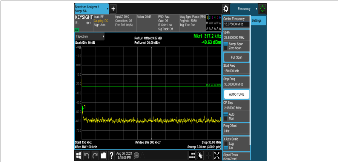
Band2-5MHz-16QAM-18625-6-0-Low-0.15-30--49.63-PASS
