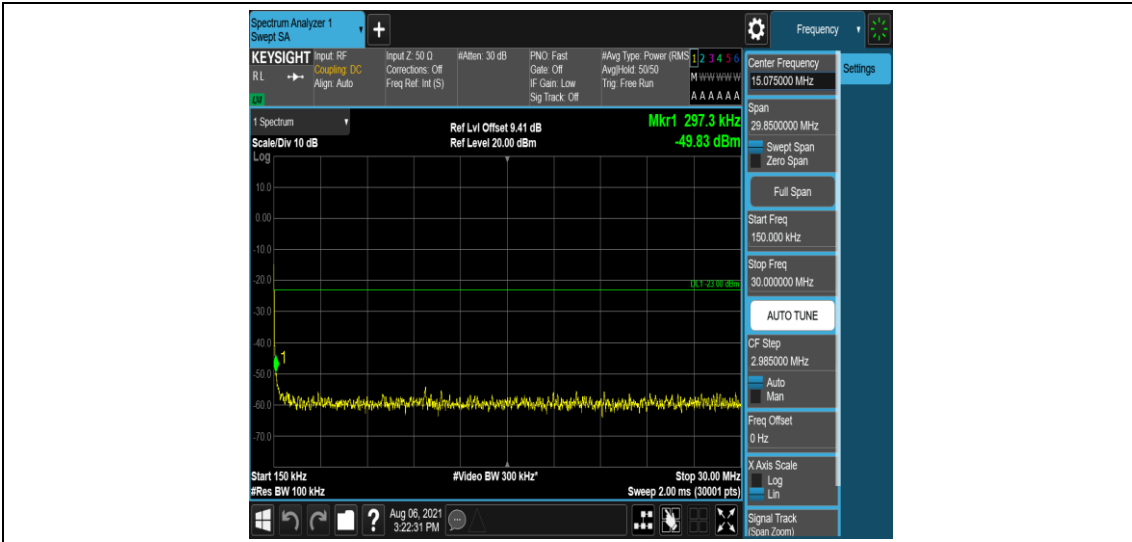
Band2-5MHz-QPSK-18900-6-0-Low-0.15-30--49.83-PASS
