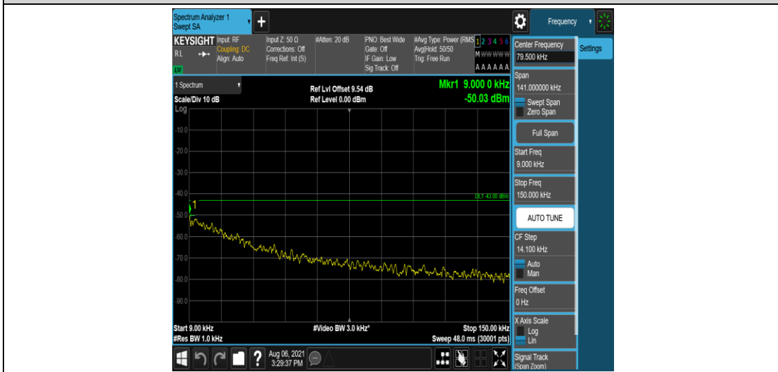
Band2-5MHz-16QAM-19175-6-0-Low-0.009-0.15--50.03-PASS
