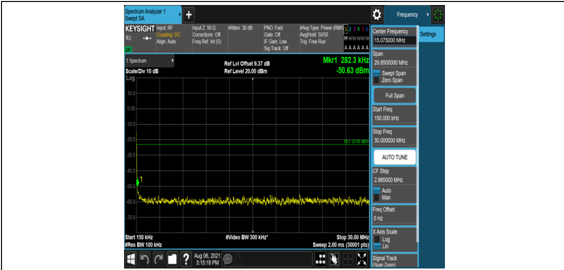
Band2-5MHz-16QAM-18625-1-0-Low-0.15-30--50.63-PASS
