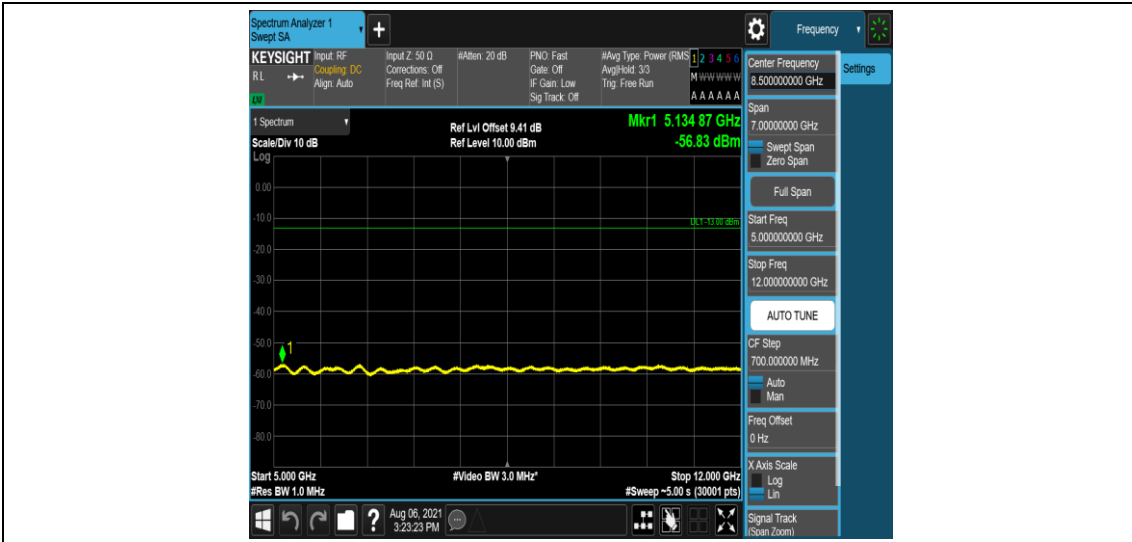
Band2-5MHz-QPSK-18900-6-0-Low-5000-12000--56.83-PASS
