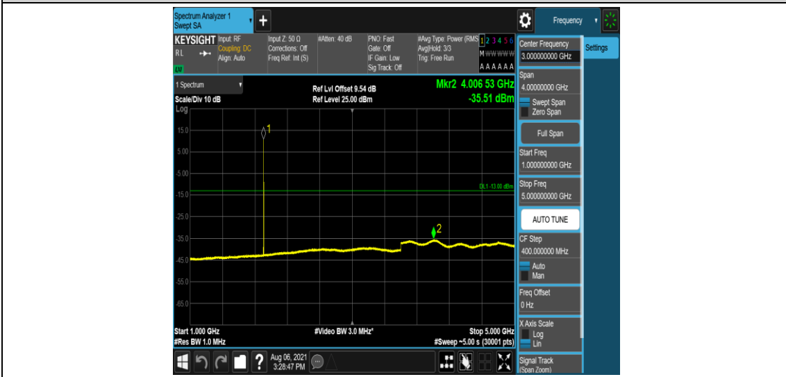
Band2-5MHz-QPSK-19175-6-0-Low-1000-5000--35.51-PASS
