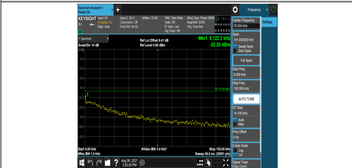
Band2-5MHz-QPSK-18900-6-0-Low-0.009-0.15--52.2-PASS
