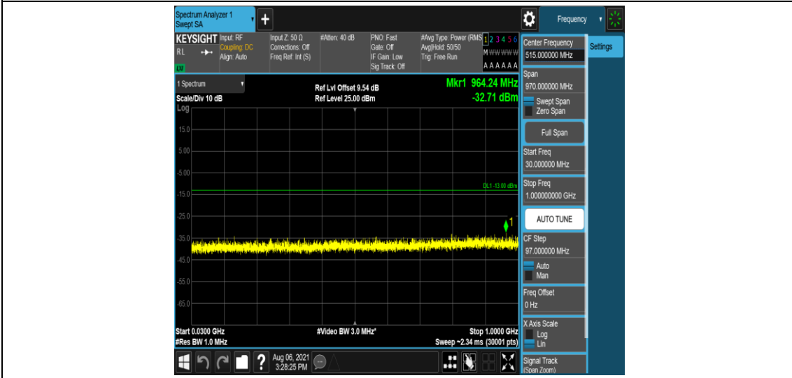
Band2-5MHz-QPSK-19175-6-0-Low-30-1000--32.71-PASS
