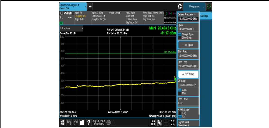
Band2-5MHz-QPSK-19175-1-5-Low-12000-26500--51.17-PASS
