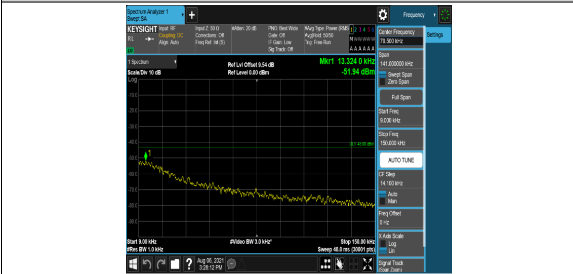
Band2-5MHz-QPSK-19175-6-0-Low-0.009-0.15--51.94-PASS
