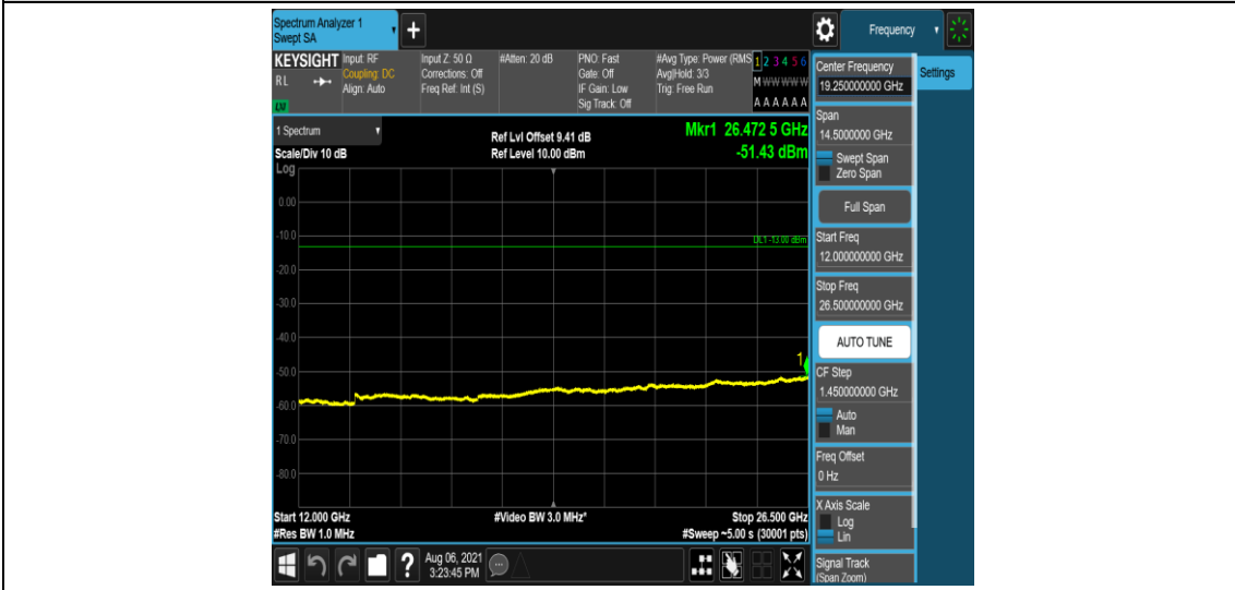
Band2-5MHz-QPSK-18900-6-0-Low-12000-26500--51.43-PASS
