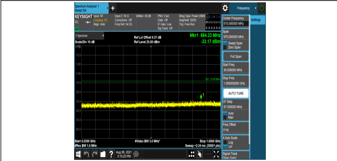
Band2-5MHz-16QAM-18625-1-0-Low-30-1000--33.17-PASS
