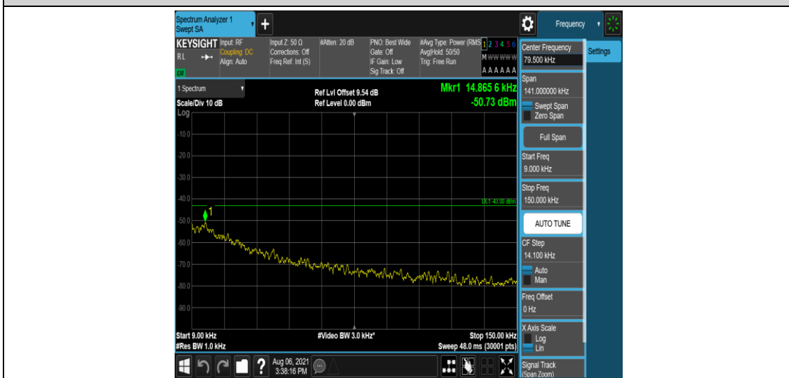
Band2-3MHz-16QAM-19185-1-5-Low-0.009-0.15--50.73-PASS
