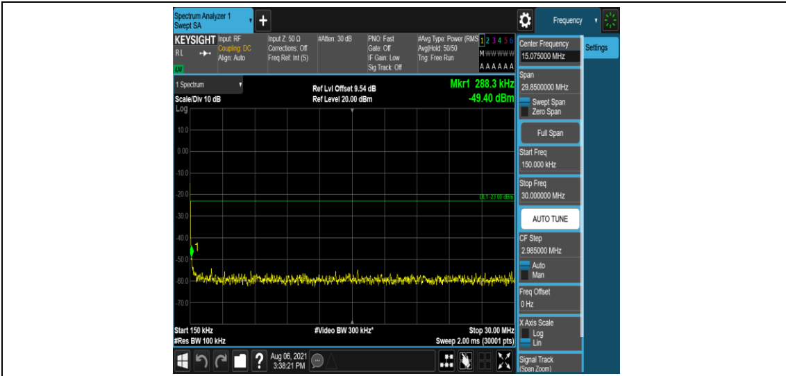
Band2-3MHz-16QAM-19185-1-5-Low-0.15-30--49.4-PASS
