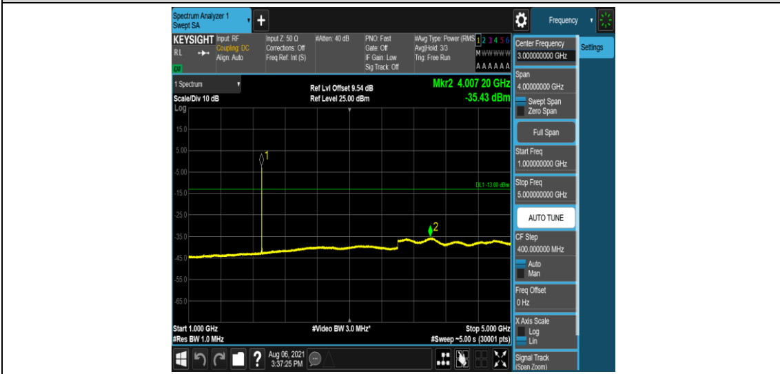
Band2-3MHz-QPSK-19185-1-5-Low-1000-5000--35.43-PASS
