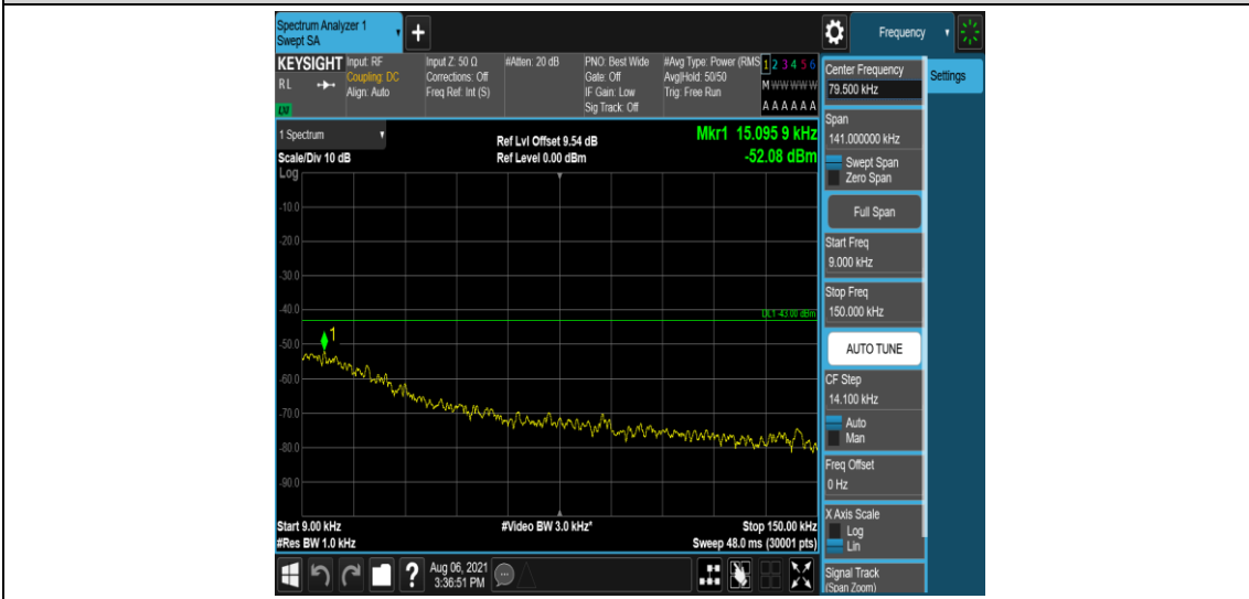
Band2-3MHz-QPSK-19185-1-5-Low-0.009-0.15--52.08-PASS
