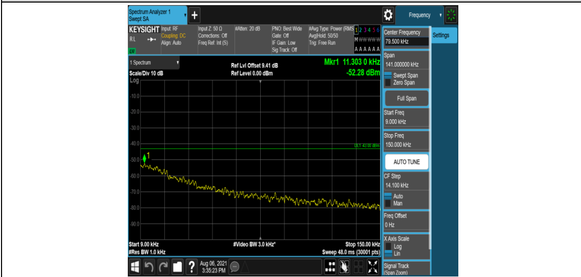
Band2-3MHz-16QAM-18900-6-0-Low-0.009-0.15--52.28-PASS
