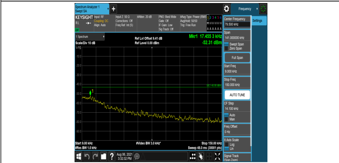
Band2-3MHz-16QAM-18900-1-0-Low-0.009-0.15--52.31-PASS
