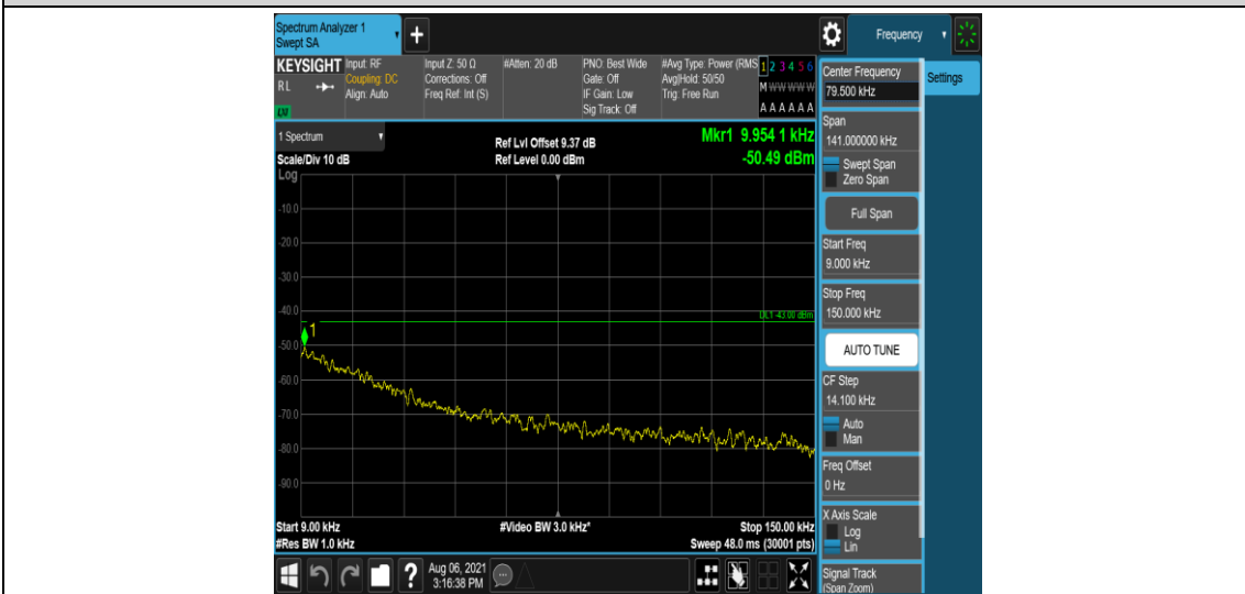
Band2-5MHz-QPSK-18625-6-0-Low-0.009-0.15--50.49-PASS
