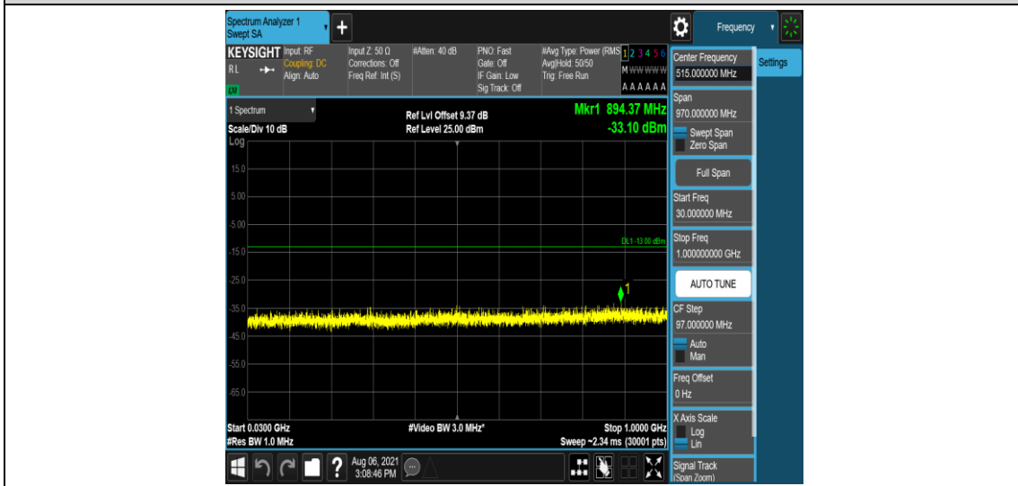
Band2-3MHz-16QAM-18615-1-0-Low-30-1000--33.1-PASS
