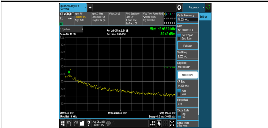
Band2-3MHz-QPSK-19185-6-0-Low-0.009-0.15--50.42-PASS
