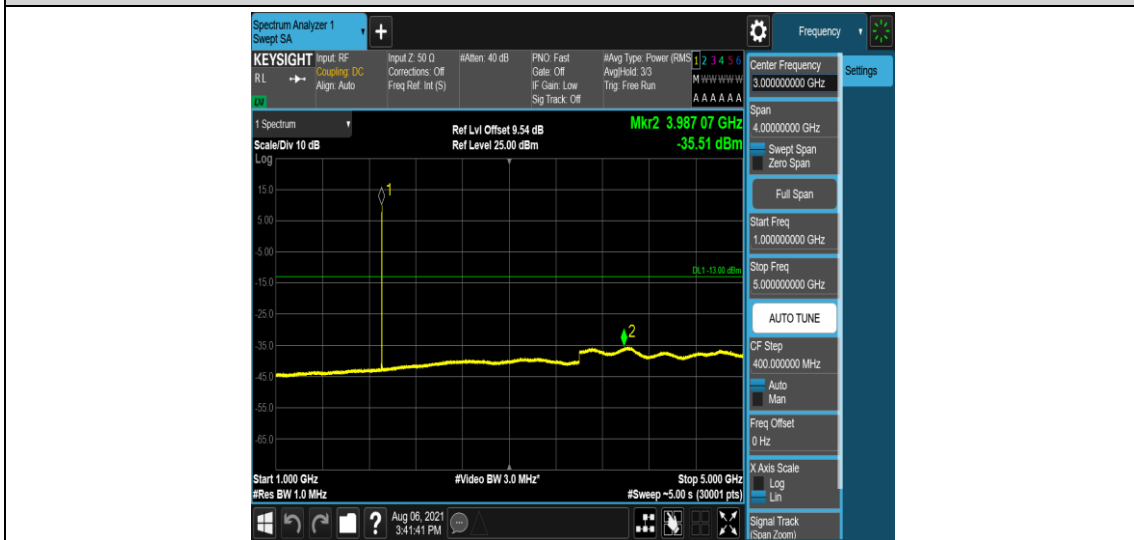
Band2-3MHz-16QAM-19185-6-0-Low-1000-5000--35.51-PASS
