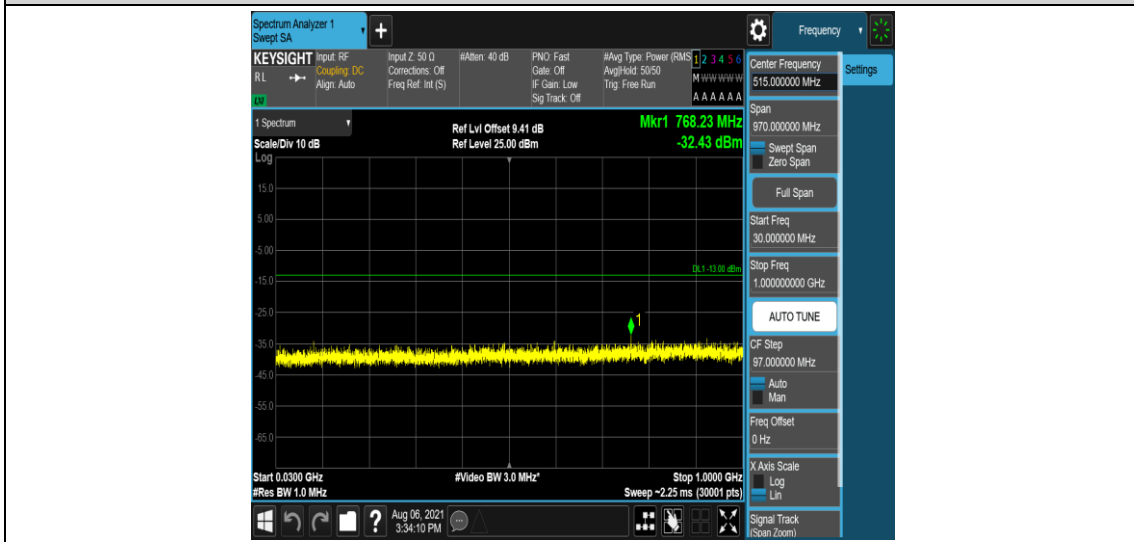
Band2-3MHz-QPSK-18900-6-0-Low-30-1000--32.43-PASS
