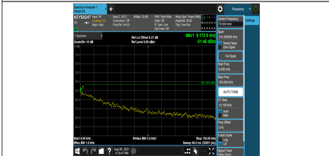
Band2-5MHz-QPSK-18625-1-0-Low-0.009-0.15--51.46-PASS
