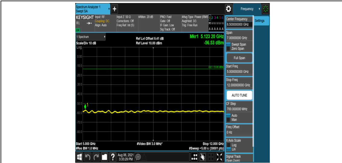
Band2-3MHz-16QAM-18900-1-0-Low-5000-12000--56.53-PASS
