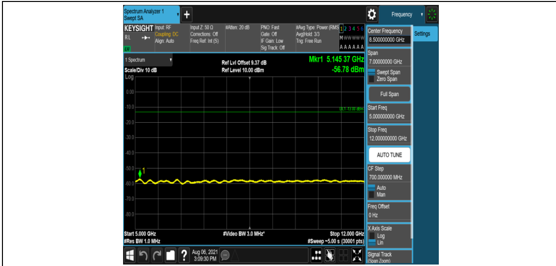
Band2-3MHz-16QAM-18615-1-0-Low-5000-12000--56.78-PASS
