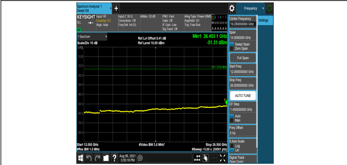
Band2-3MHz-QPSK-18900-6-0-Low-12000-26500--51.31-PASS
