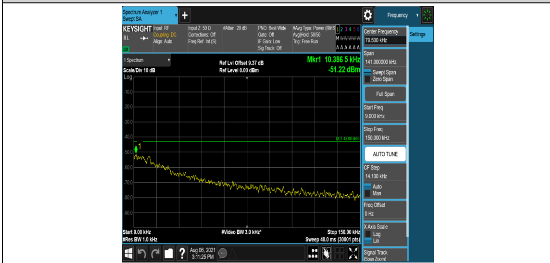
Band2-3MHz-16QAM-18615-6-0-Low-0.009-0.15--51.22-PASS
