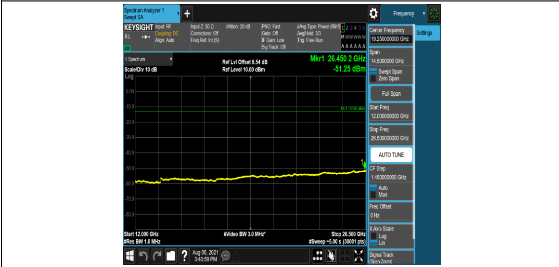
Band2-3MHz-QPSK-19185-6-0-Low-12000-26500--51.25-PASS
