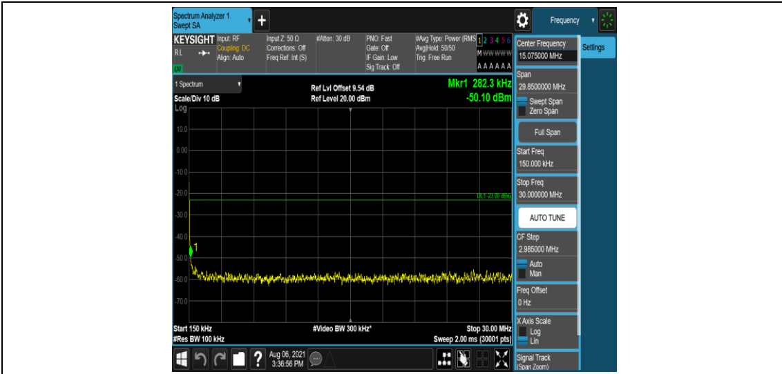
Band2-3MHz-QPSK-19185-1-5-Low-0.15-30--50.1-PASS
