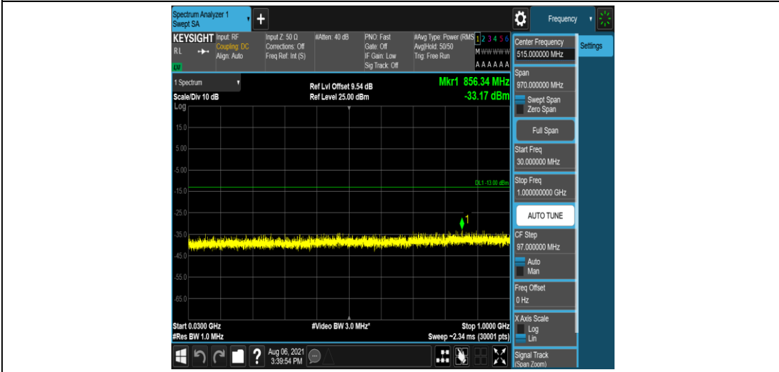
Band2-3MHz-QPSK-19185-6-0-Low-30-1000--33.17-PASS
