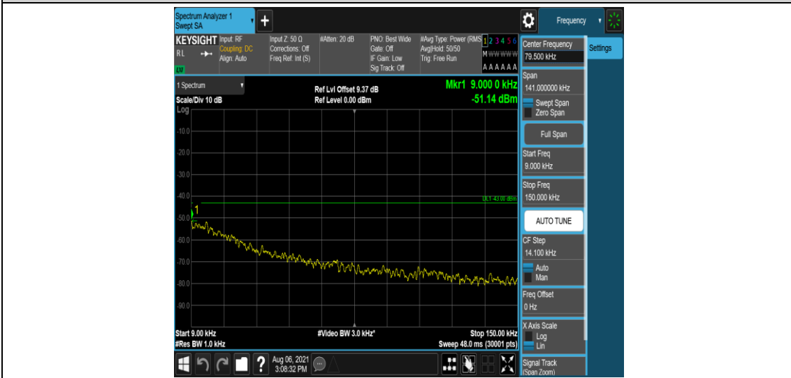
Band2-3MHz-16QAM-18615-1-0-Low-0.009-0.15--51.14-PASS
