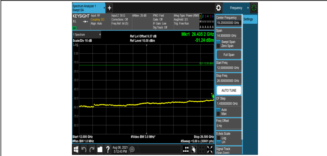
Band2-3MHz-16QAM-18615-6-0-Low-12000-26500--51.24-PASS
