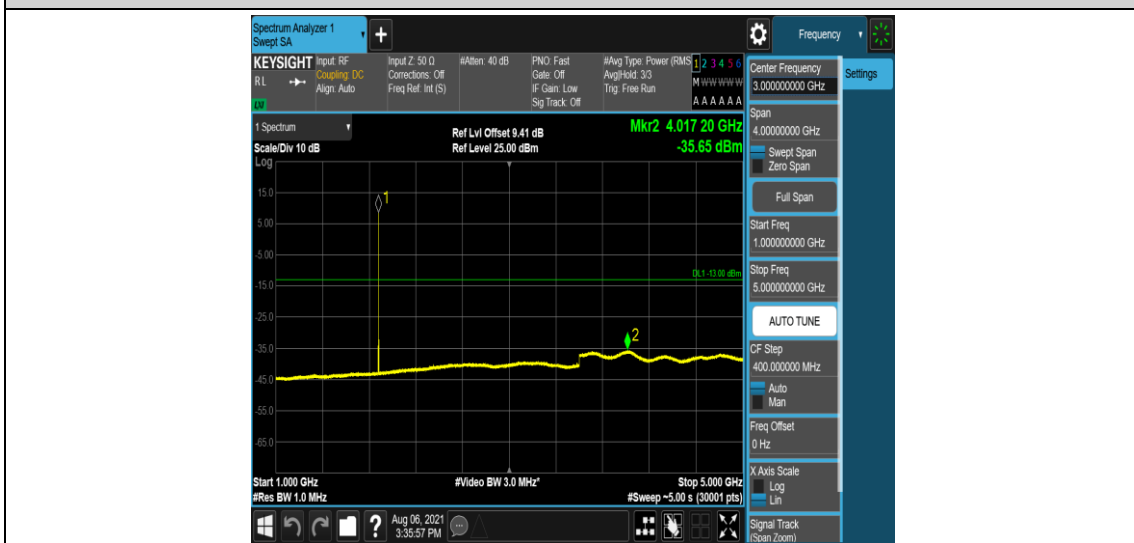
Band2-3MHz-16QAM-18900-6-0-Low-1000-5000--35.65-PASS
