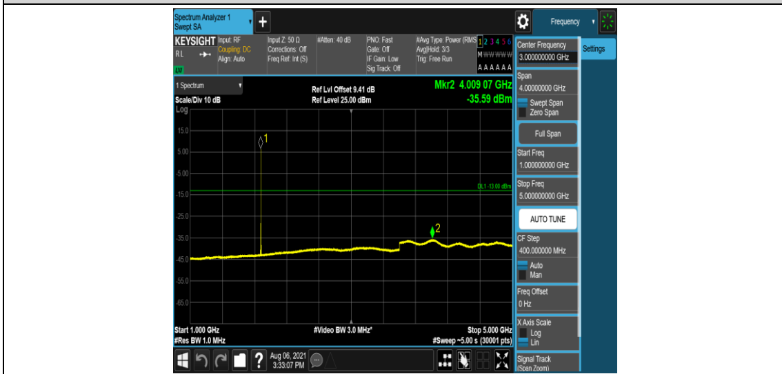
Band2-3MHz-16QAM-18900-1-0-Low-1000-5000--35.59-PASS
