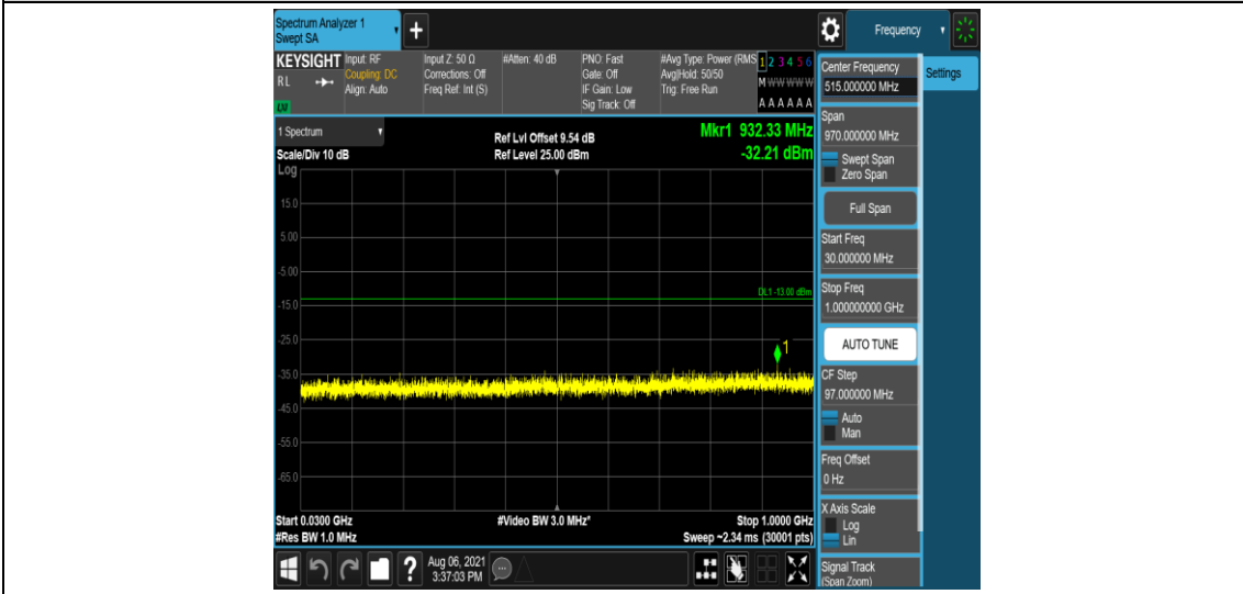
Band2-3MHz-QPSK-19185-1-5-Low-30-1000--32.21-PASS
