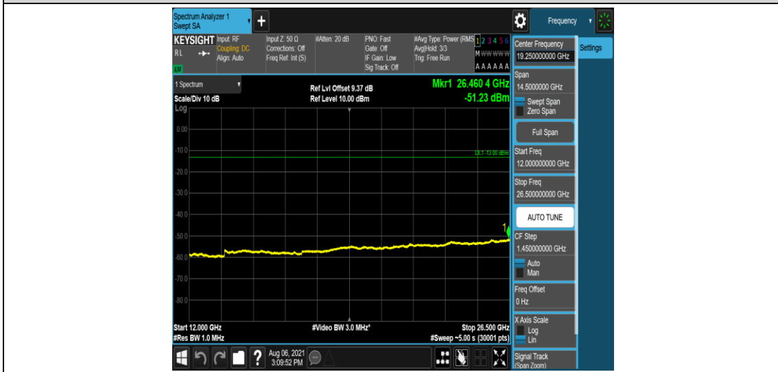
Band2-3MHz-16QAM-18615-1-0-Low-12000-26500--51.23-PASS
