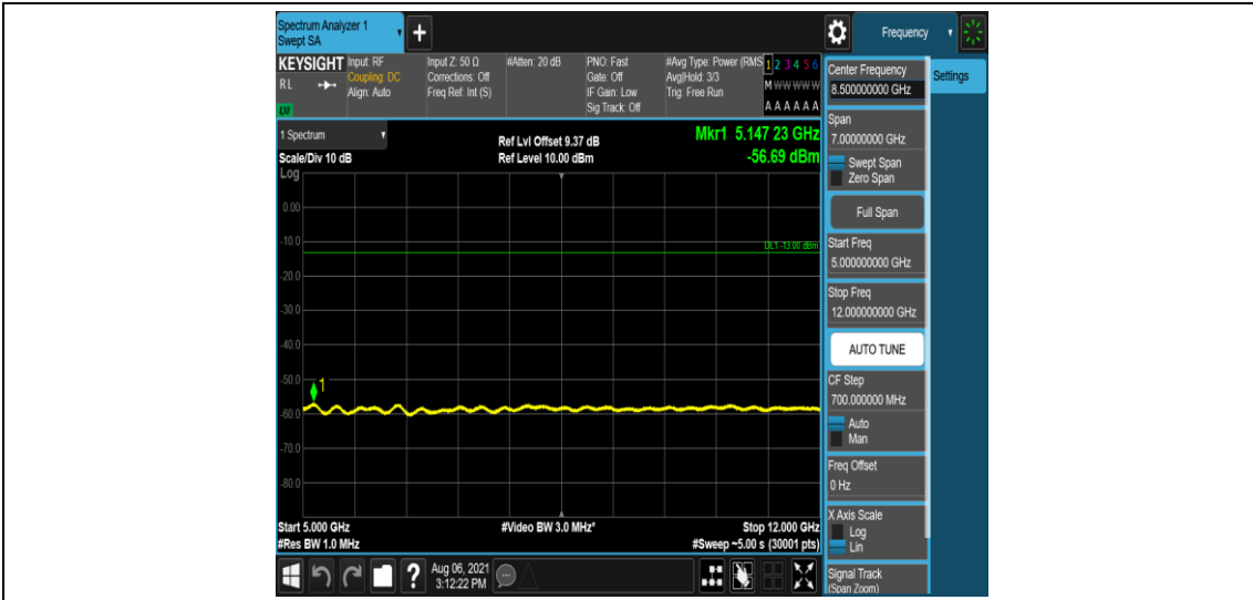
Band2-3MHz-16QAM-18615-6-0-Low-5000-12000--56.69-PASS
