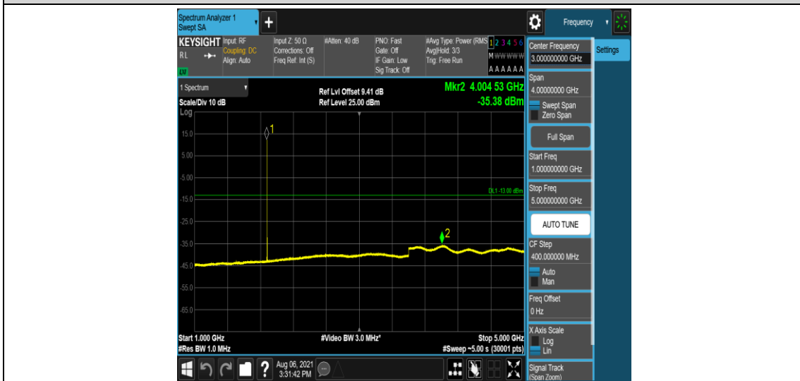
Band2-3MHz-QPSK-18900-1-0-Low-1000-5000--35.38-PASS
