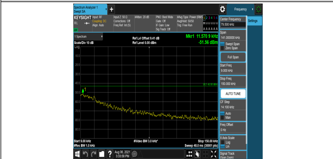
Band2-3MHz-QPSK-18900-6-0-Low-0.009-0.15--51.56-PASS
