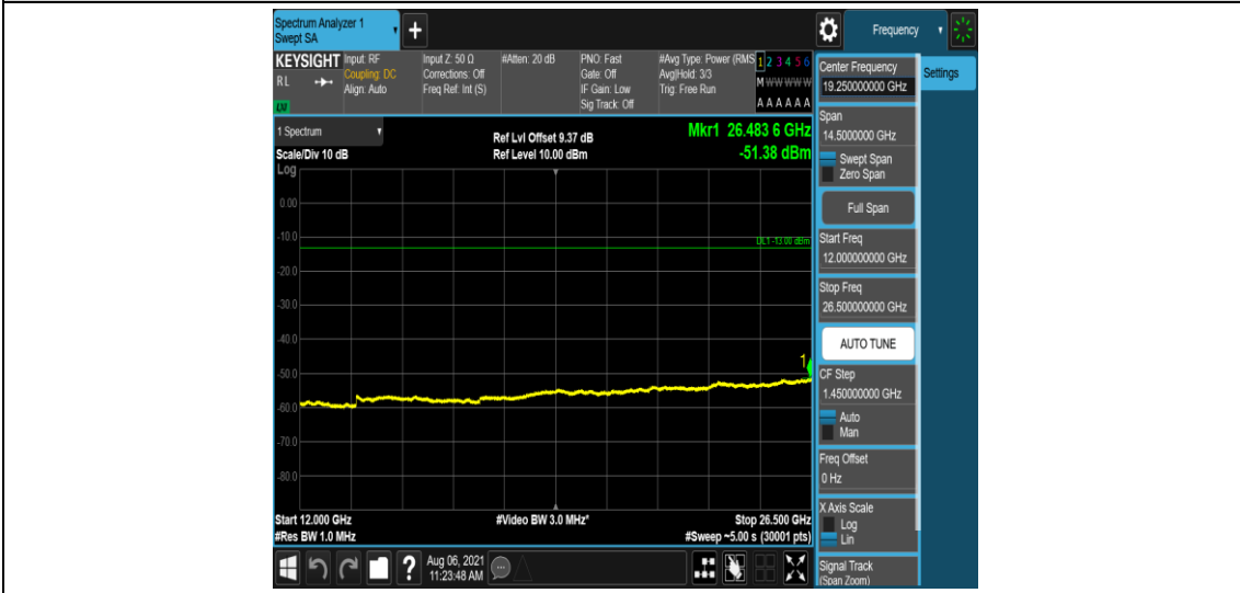
Band2-1.4MHz-16QAM-18607-6-0-Low-12000-26500--51.38-PASS
