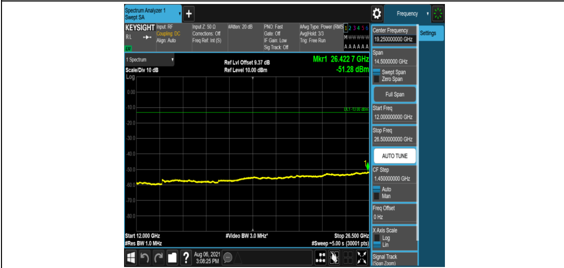
Band2-3MHz-QPSK-18615-1-0-Low-12000-26500--51.28-PASS
