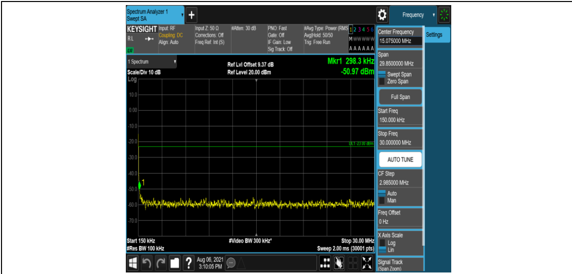
Band2-3MHz-QPSK-18615-6-0-Low-0.15-30--50.97-PASS
