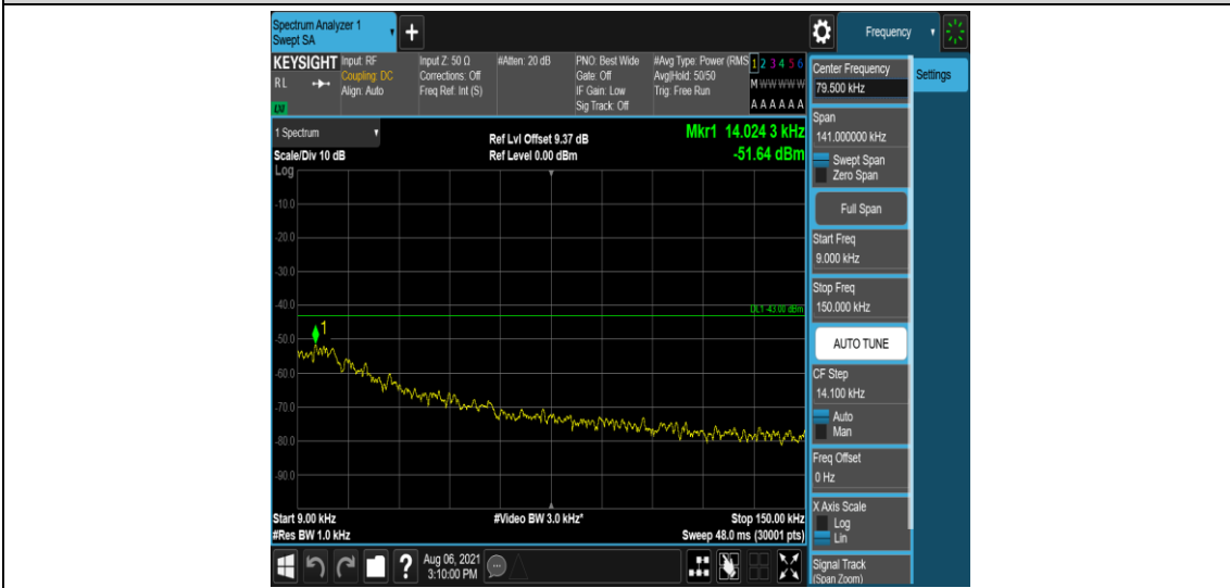
Band2-3MHz-QPSK-18615-6-0-Low-0.009-0.15--51.64-PASS
