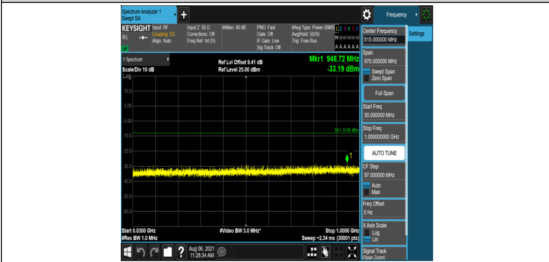
Band2-1.4MHz-16QAM-18900-6-0-Low-30-1000--33.19-PASS
