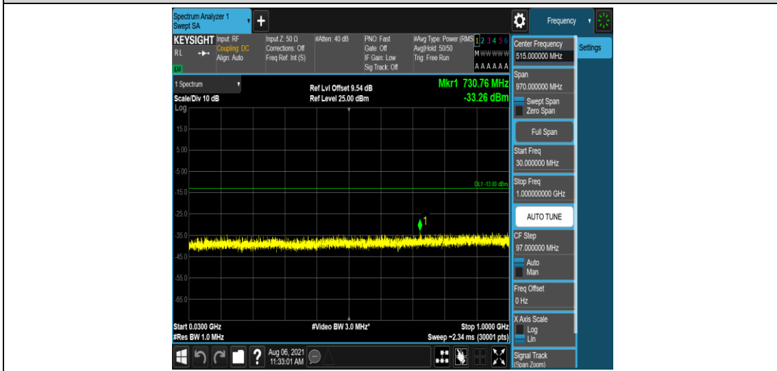
Band2-1.4MHz-QPSK-19193-6-0-Low-30-1000--33.26-PASS
