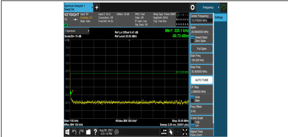
Band2-3MHz-QPSK-18900-1-0-Low-0.15-30--50.73-PASS
