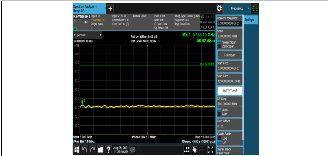
Band2-1.4MHz-16QAM-18900-6-0-Low-5000-12000--56.92-PASS
