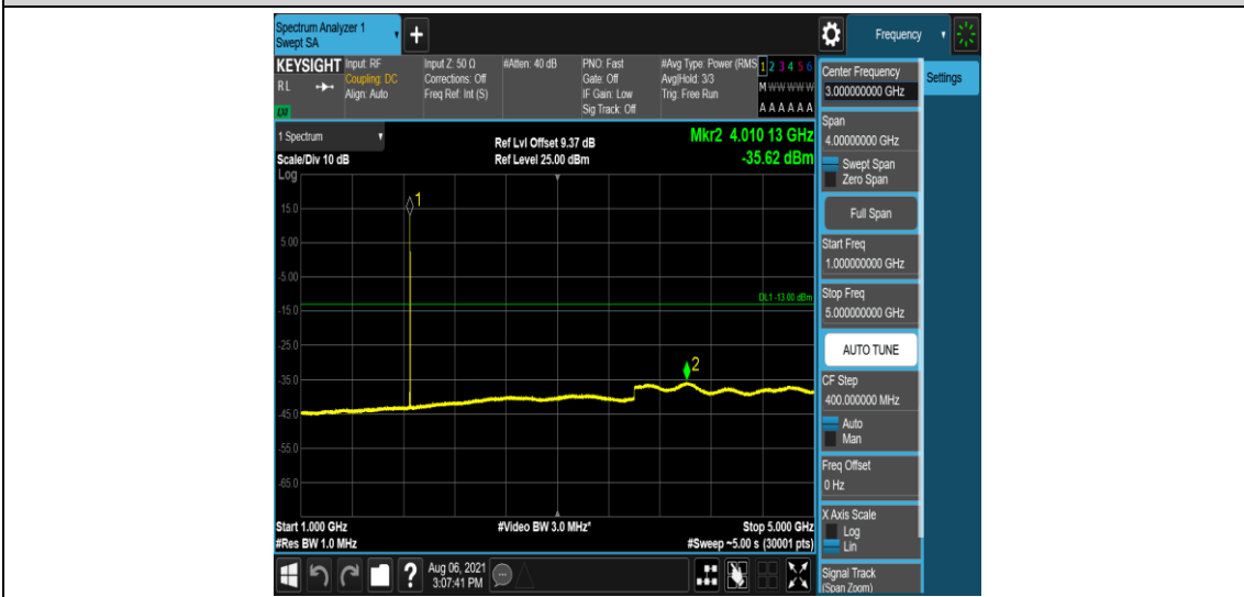
Band2-3MHz-QPSK-18615-1-0-Low-1000-5000--35.62-PASS
