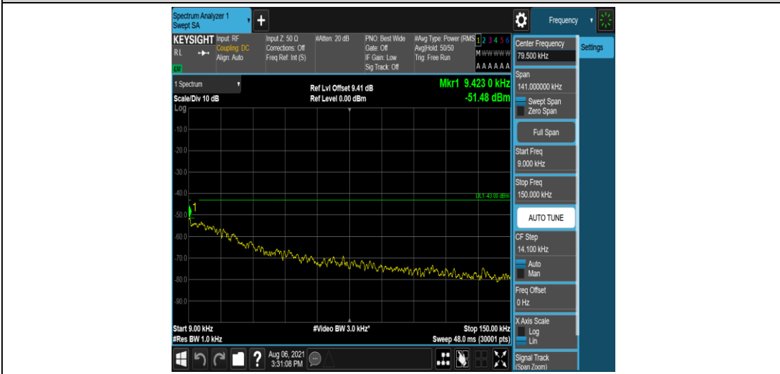
Band2-3MHz-QPSK-18900-1-0-Low-0.009-0.15--51.48-PASS
