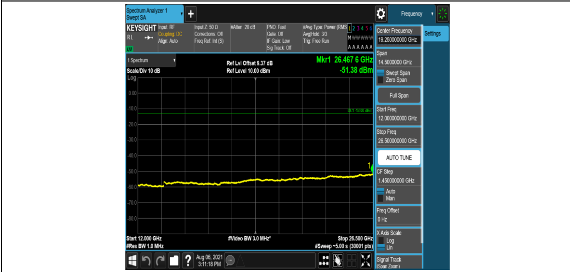
Band2-3MHz-QPSK-18615-6-0-Low-12000-26500--51.38-PASS
