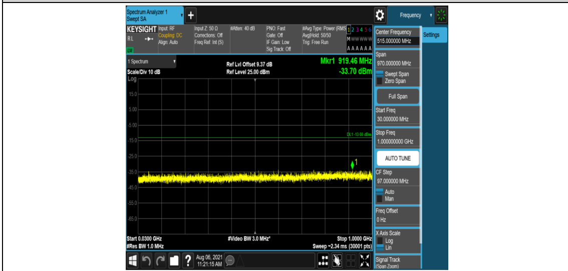
Band2-1.4MHz-QPSK-18607-6-0-Low-30-1000--33.7-PASS
