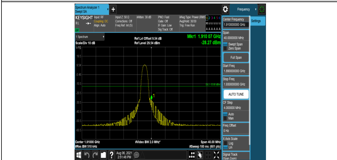
Band2-20MHz-QPSK-19100-6-0-High--28.27-PASS
