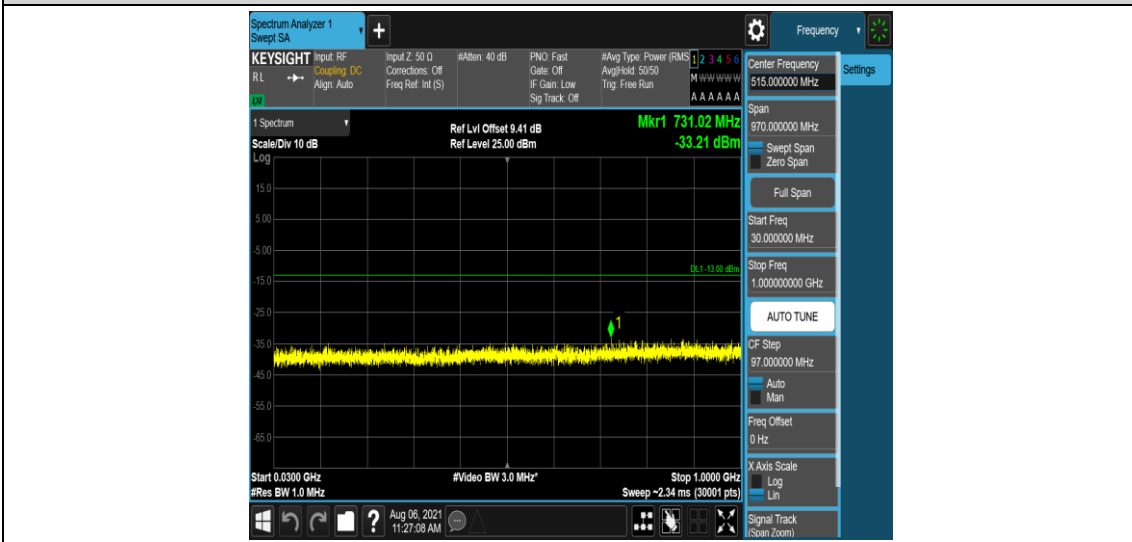
Band2-1.4MHz-QPSK-18900-6-0-Low-30-1000--33.21-PASS
