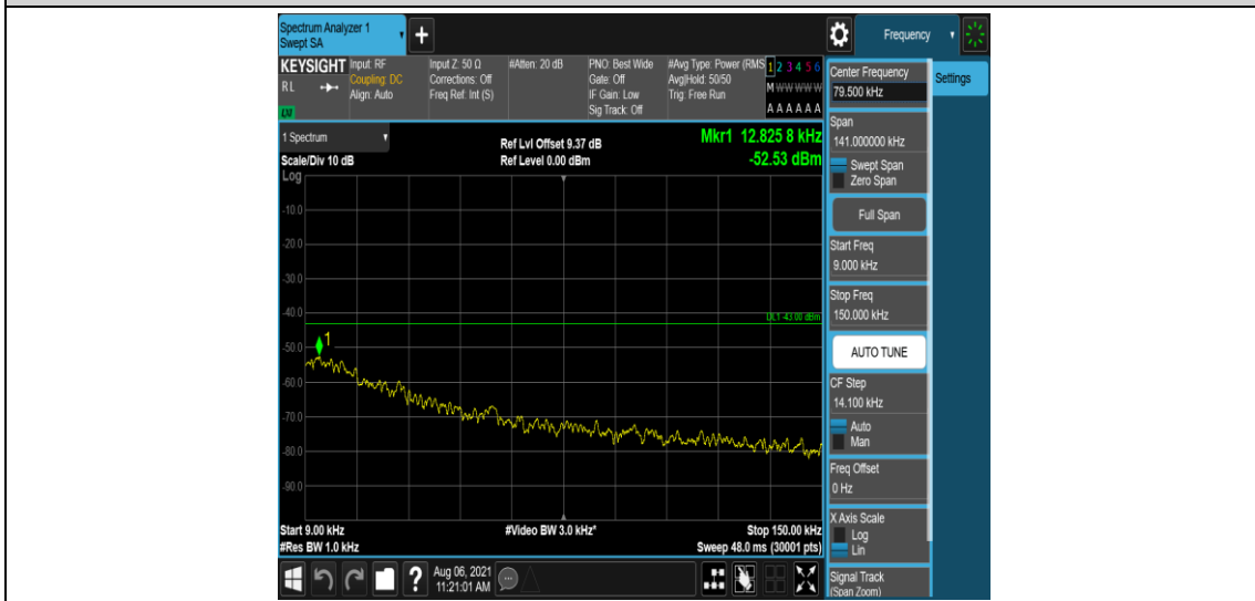
Band2-1.4MHz-QPSK-18607-6-0-Low-0.009-0.15--52.53-PASS
