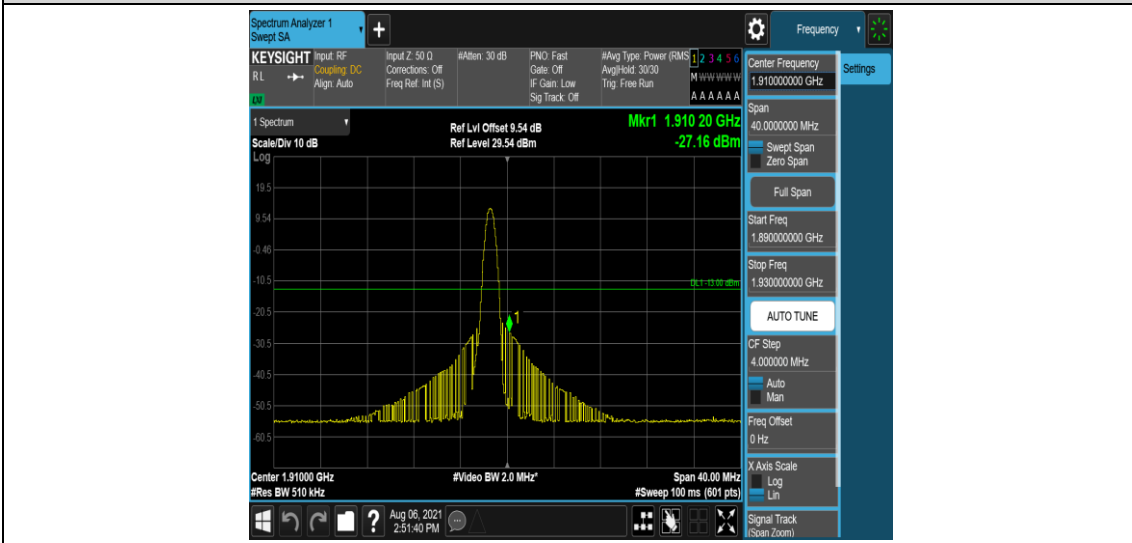
Band2-20MHz-16QAM-19100-1-5-High--27.16-PASS
