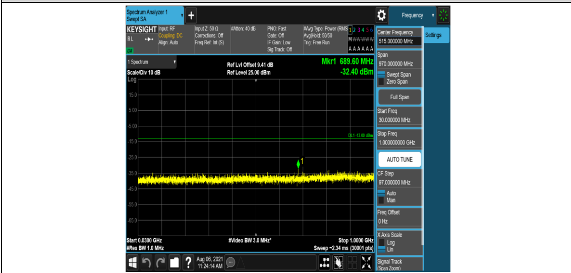
Band2-1.4MHz-QPSK-18900-1-0-Low-30-1000--32.4-PASS
