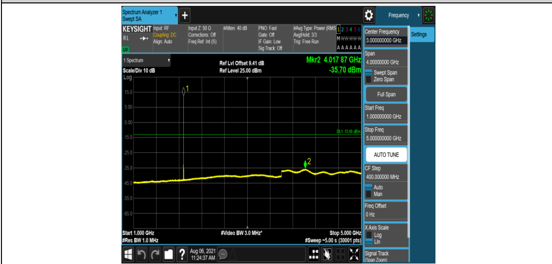
Band2-1.4MHz-QPSK-18900-1-0-Low-1000-5000--35.7-PASS
