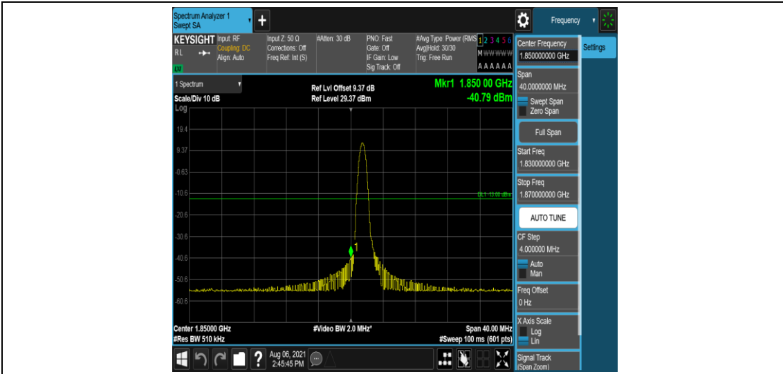
Band2-20MHz-16QAM-18700-1-0-Low--40.79-PASS
