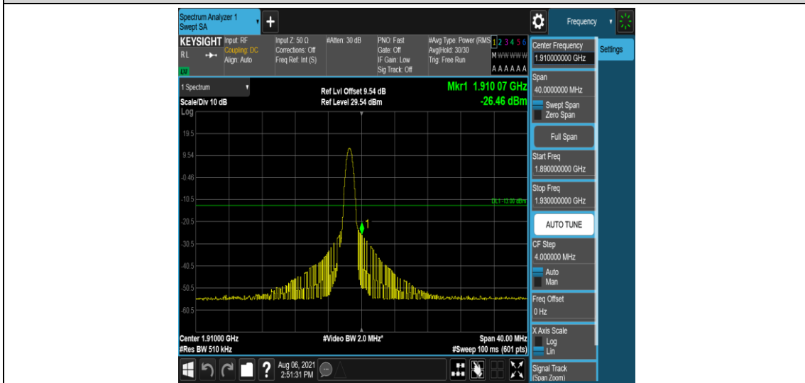
Band2-20MHz-QPSK-19100-1-5-High--26.46-PASS
