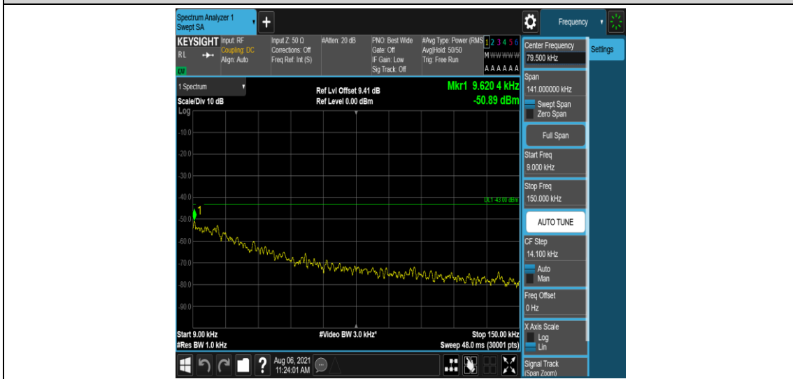
Band2-1.4MHz-QPSK-18900-1-0-Low-0.009-0.15--50.89-PASS
