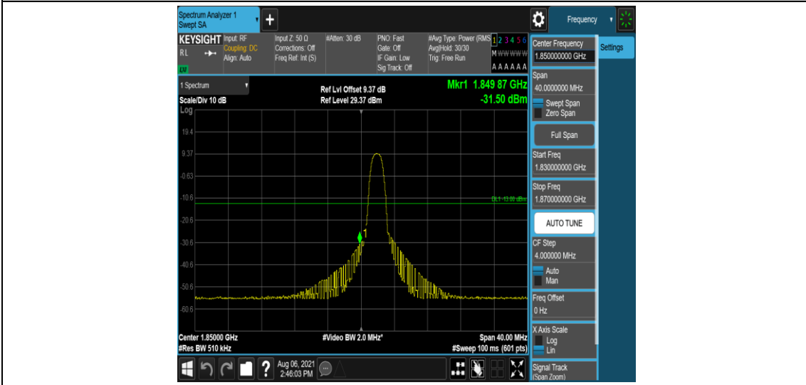
Band2-20MHz-16QAM-18700-6-0-Low--31.50-PASS
