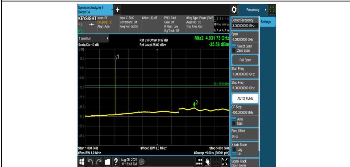
Band2-1.4MHz-QPSK-18607-1-0-Low-1000-5000--35.58-PASS
