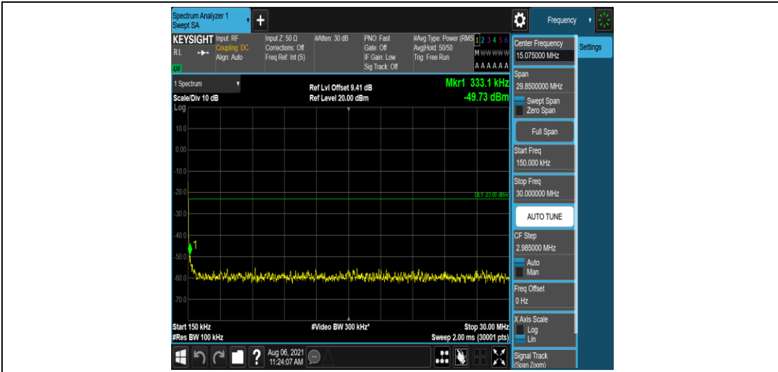
Band2-1.4MHz-QPSK-18900-1-0-Low-0.15-30--49.73-PASS
