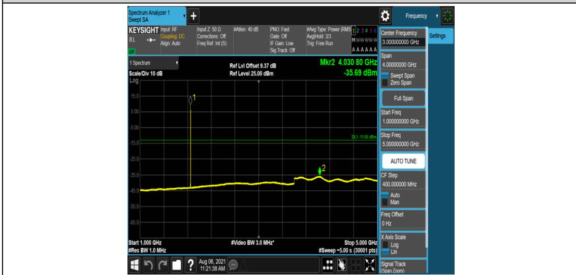
Band2-1.4MHz-QPSK-18607-6-0-Low-1000-5000--35.69-PASS
