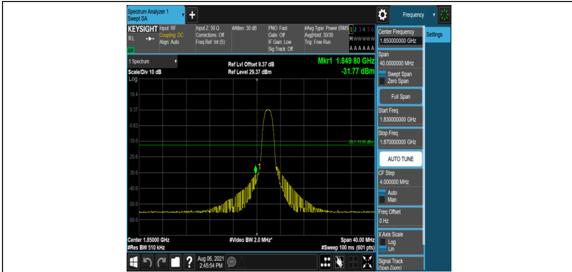
Band2-20MHz-QPSK-18700-6-0-Low--31.77-PASS
