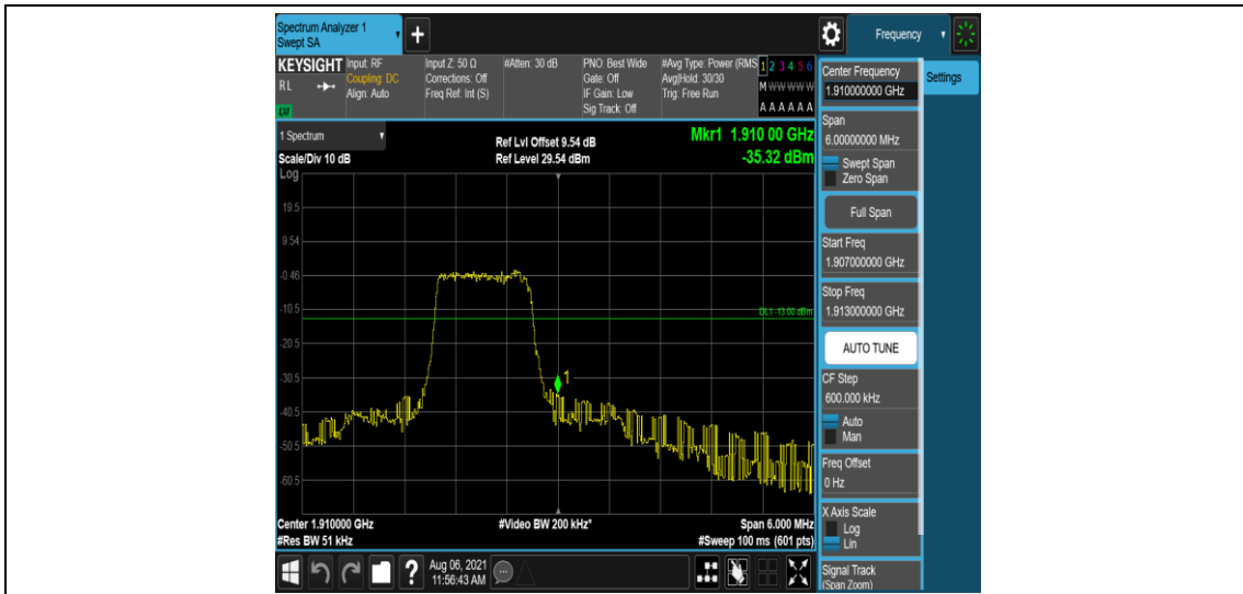
Band2-3MHz-QPSK-19185-6-0-High--35.32-PASS
