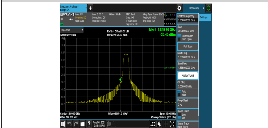
Band2-15MHz-16QAM-18675-6-0-Low--30.45-PASS
