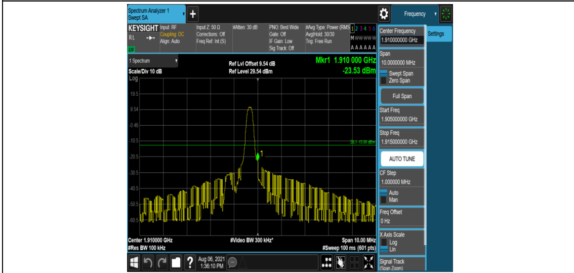
Band2-5MHz-QPSK-19175-1-5-High--23.53-PASS
