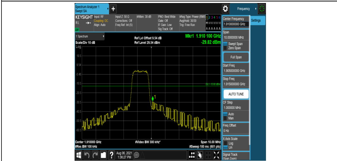
Band2-5MHz-QPSK-19175-6-0-High--29.82-PASS
