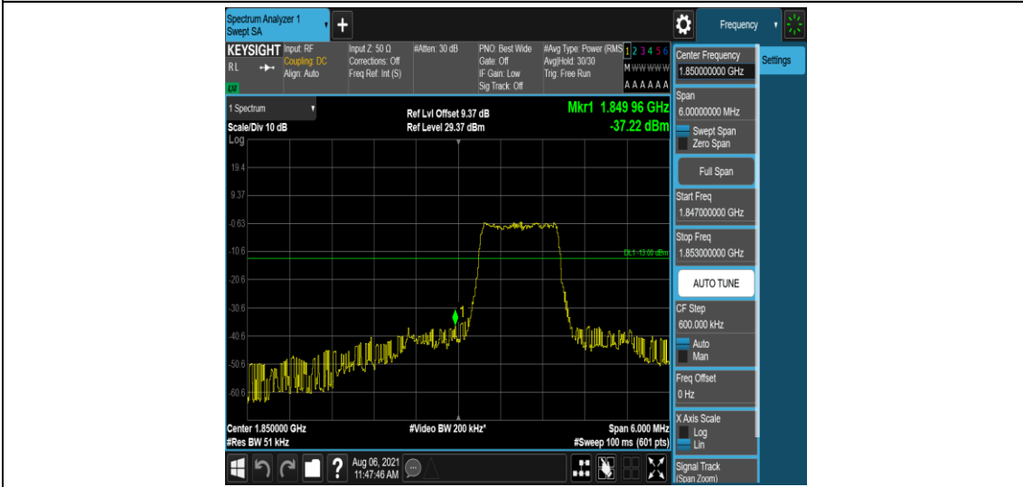
Band2-3MHz-QPSK-18615-6-0-Low--37.22-PASS
