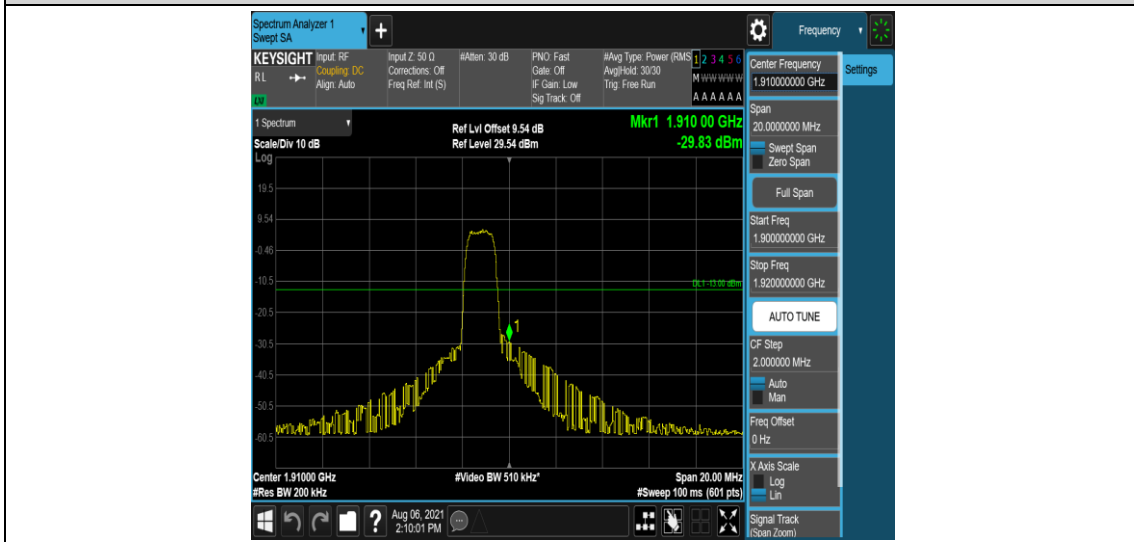
Band2-10MHz-QPSK-19150-6-0-High--29.83-PASS
