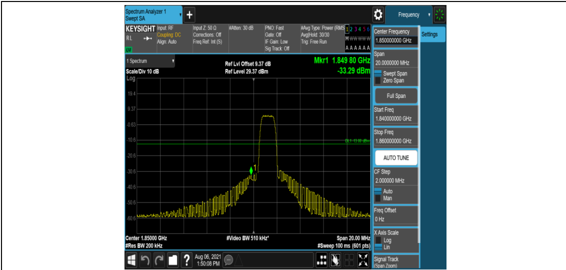
Band2-10MHz-16QAM-18650-6-0-Low--33.29-PASS
