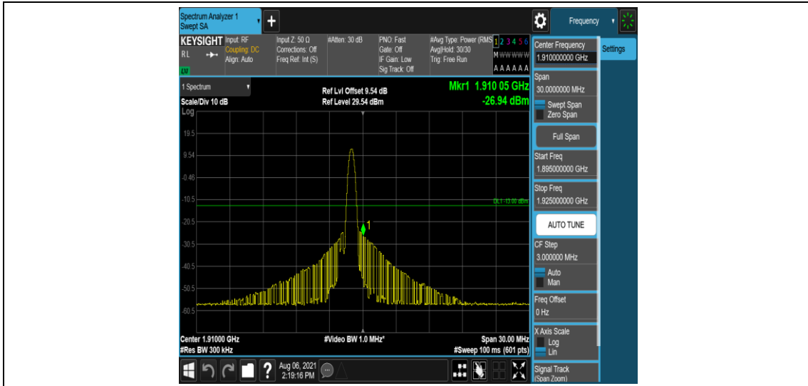
Band2-15MHz-16QAM-19125-1-5-High--26.94-PASS
