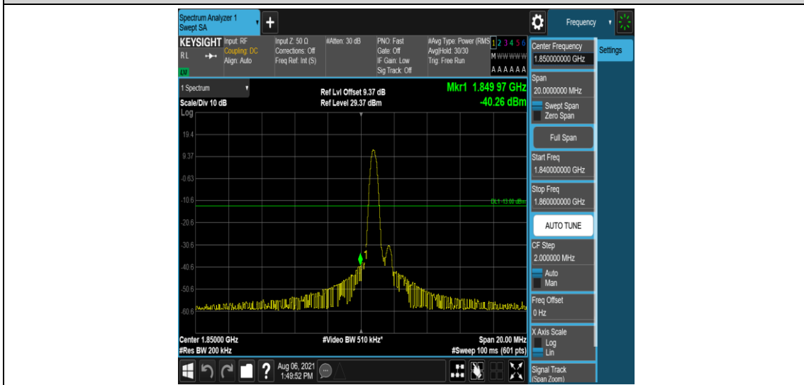
Band2-10MHz-16QAM-18650-1-0-Low--40.26-PASS
