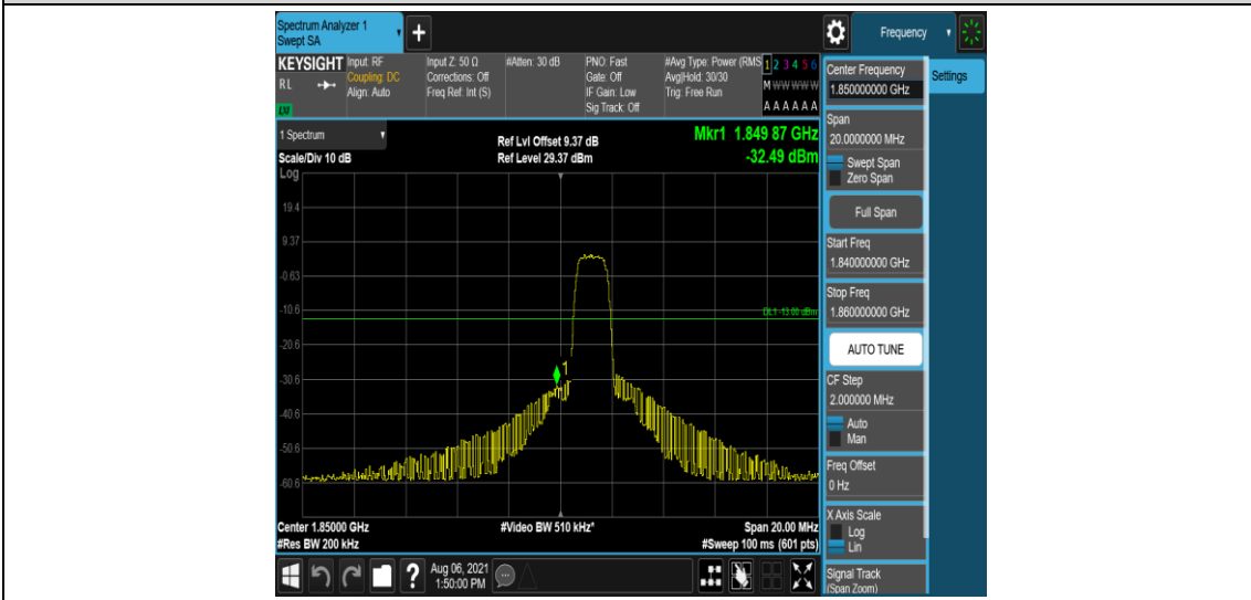
Band2-10MHz-QPSK-18650-6-0-Low--32.49-PASS
