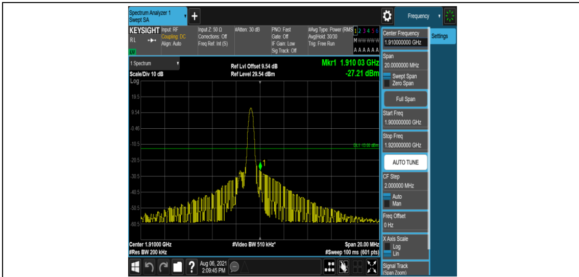
Band2-10MHz-QPSK-19150-1-5-High--27.21-PASS
