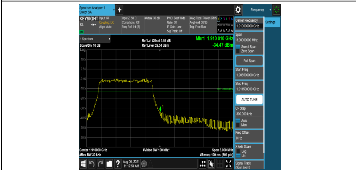
Band2-1.4MHz-16QAM-19193-6-0-High--34.47-PASS
