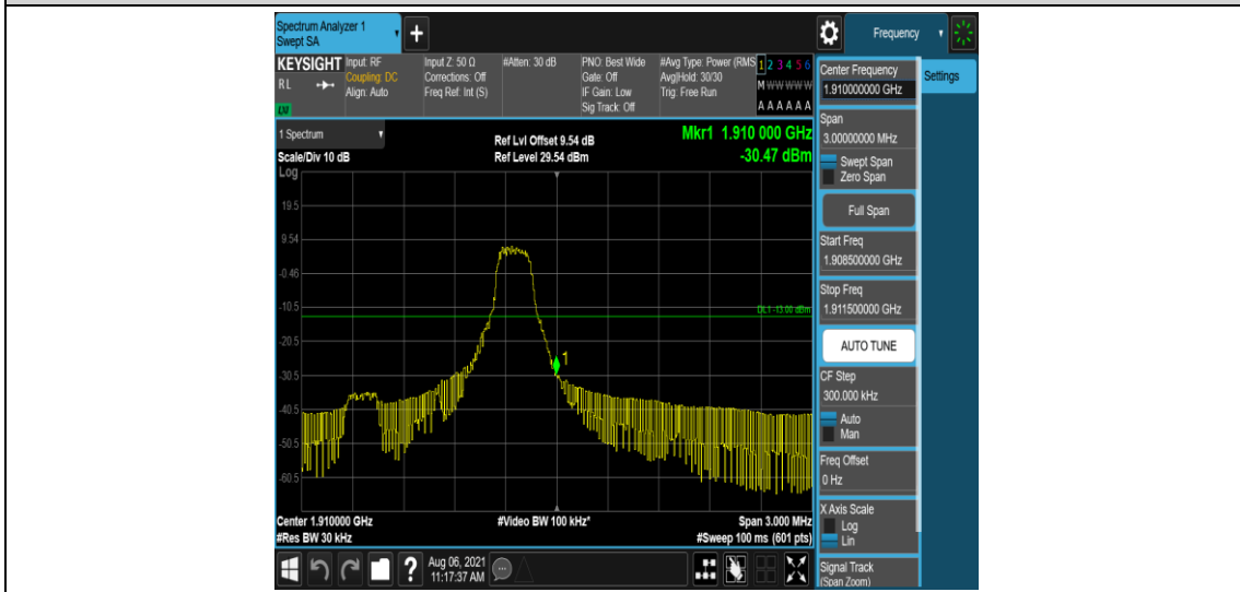
Band2-1.4MHz-16QAM-19193-1-5-High--30.47-PASS
