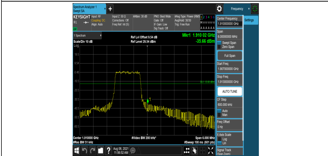
Band2-3MHz-16QAM-19185-6-0-High--35.66-PASS
