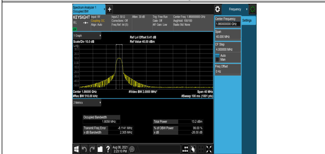
Band2-20MHz-QPSK-18700-6-0-Low-1.8058-2.305-PASS
