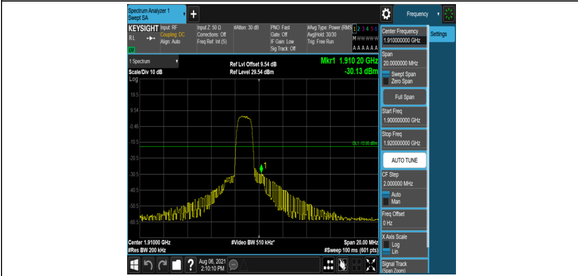
Band2-10MHz-16QAM-19150-6-0-High--30.13-PASS
