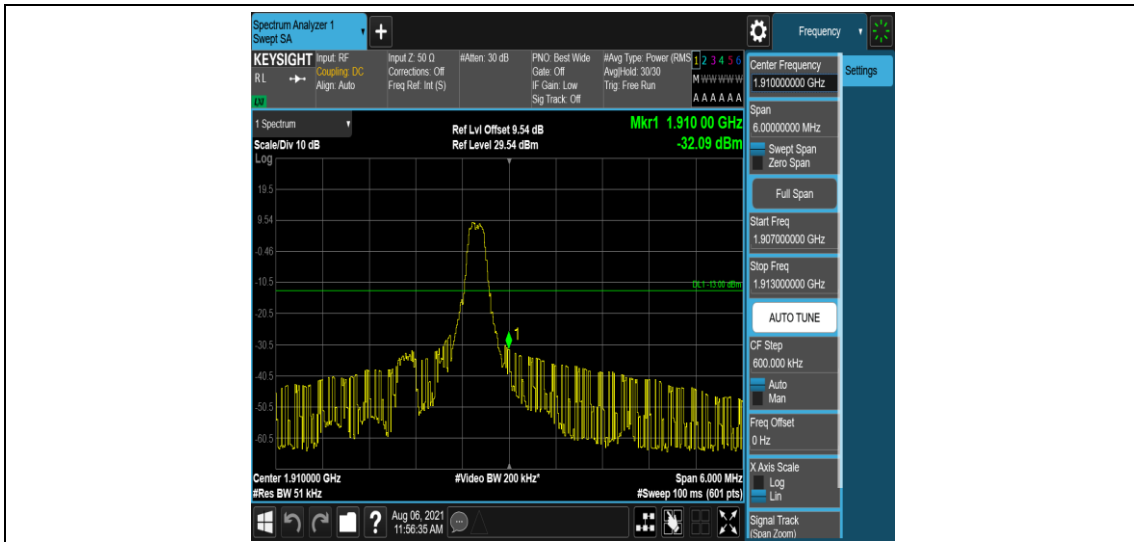
Band2-3MHz-16QAM-19185-1-5-High--32.09-PASS
