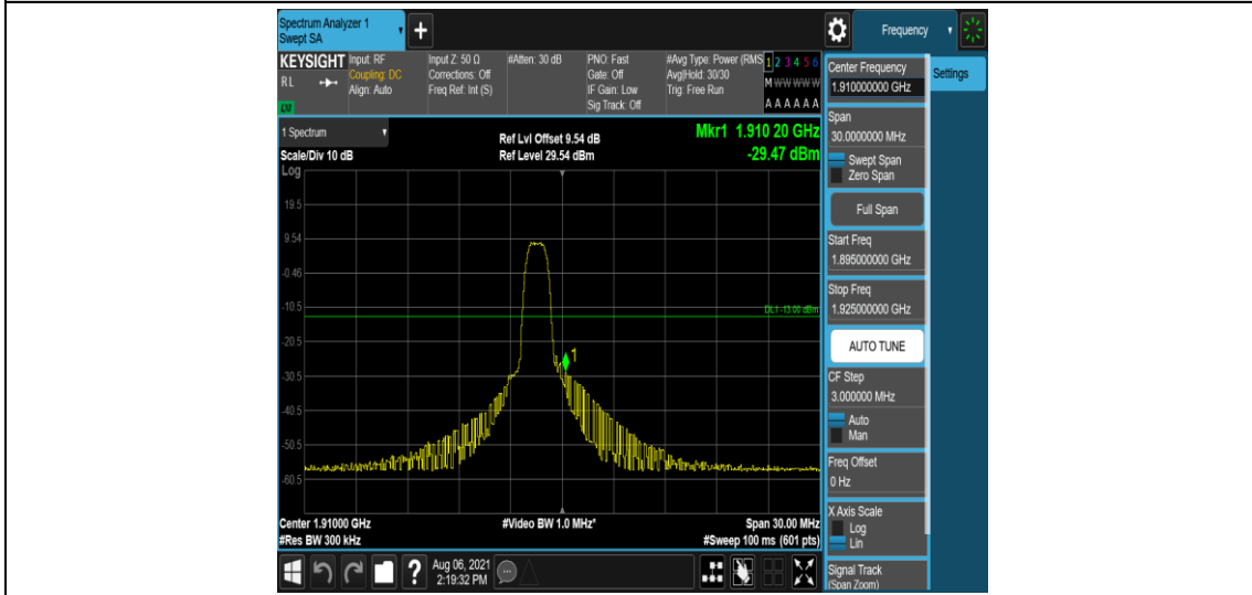
Band2-15MHz-16QAM-19125-6-0-High--29.47-PASS
