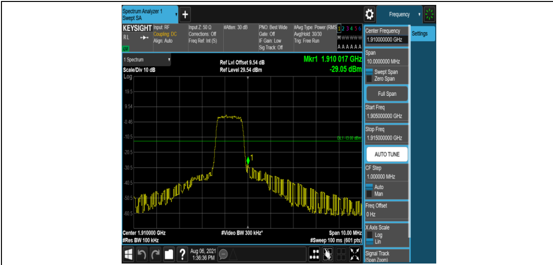
Band2-5MHz-16QAM-19175-6-0-High--29.05-PASS
