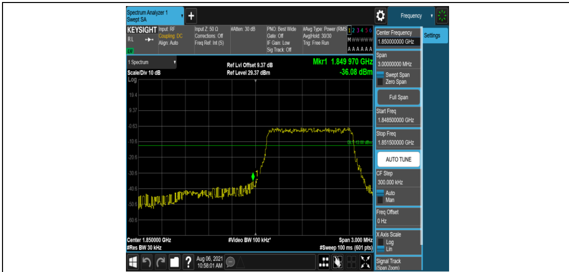
Band2-1.4MHz-16QAM-18607-6-0-Low--36.08-PASS
