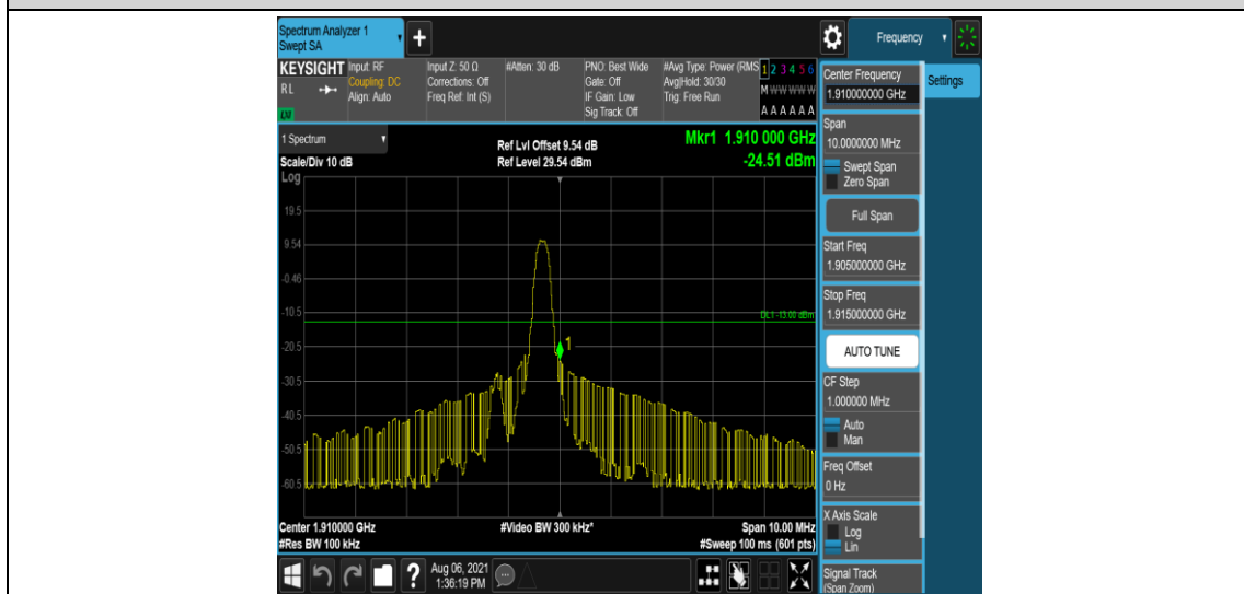
Band2-5MHz-16QAM-19175-1-5-High--24.51-PASS
