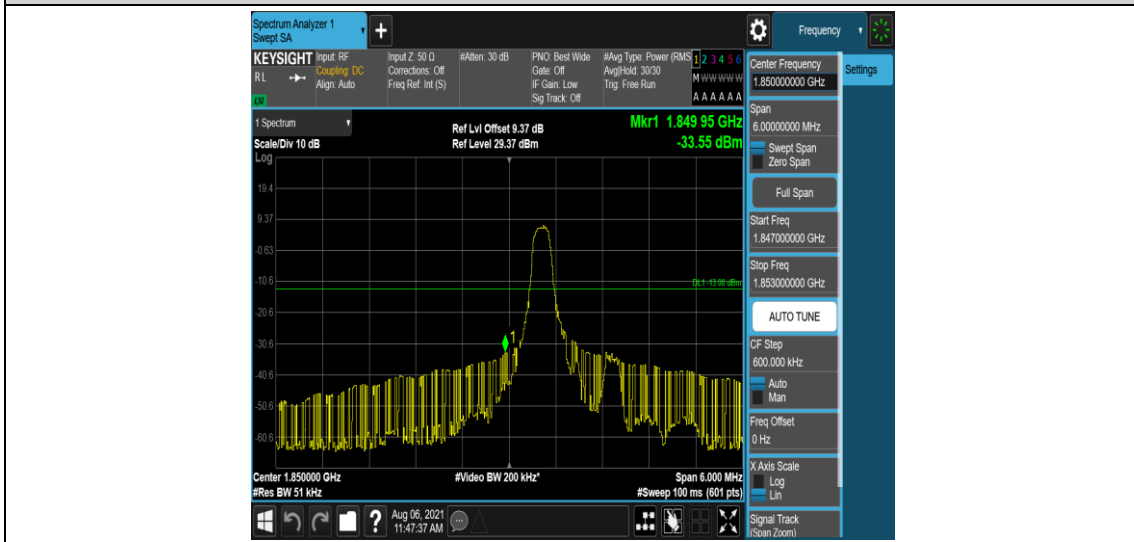
Band2-3MHz-16QAM-18615-1-0-Low--33.55-PASS
