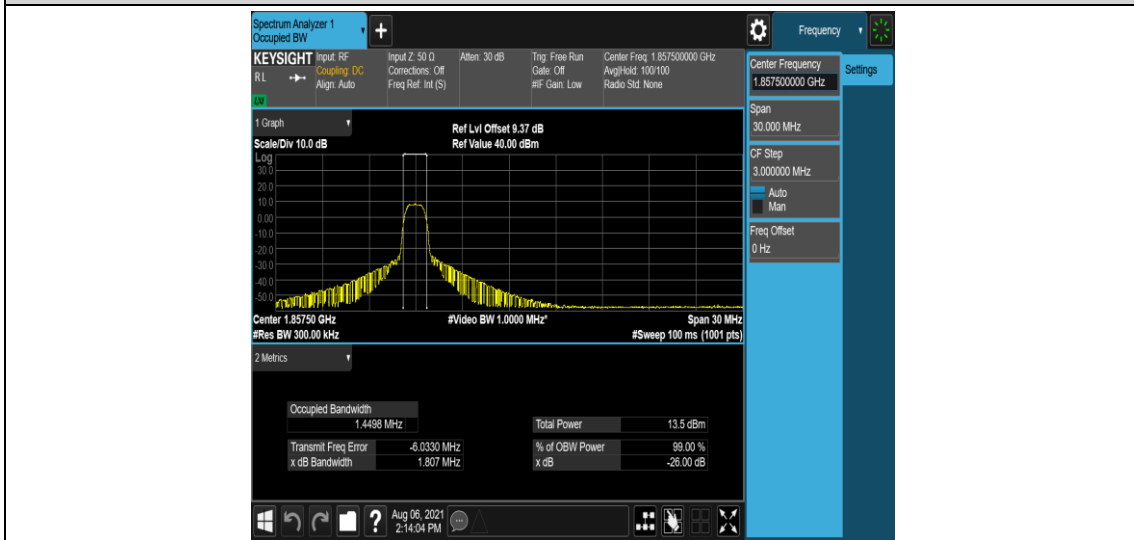
Band2-15MHz-16QAM-18675-6-0-Low-1.4498-1.807-PASS
