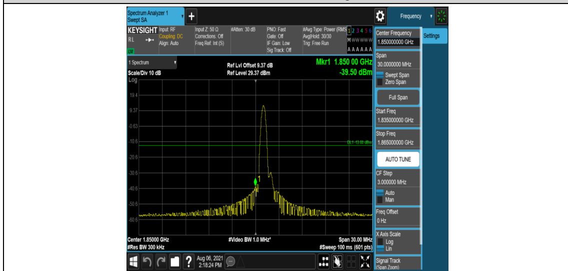
Band2-15MHz-16QAM-18675-1-0-Low--39.50-PASS
