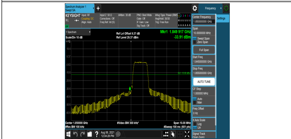
Band2-5MHz-16QAM-18625-6-0-Low--33.91-PASS
