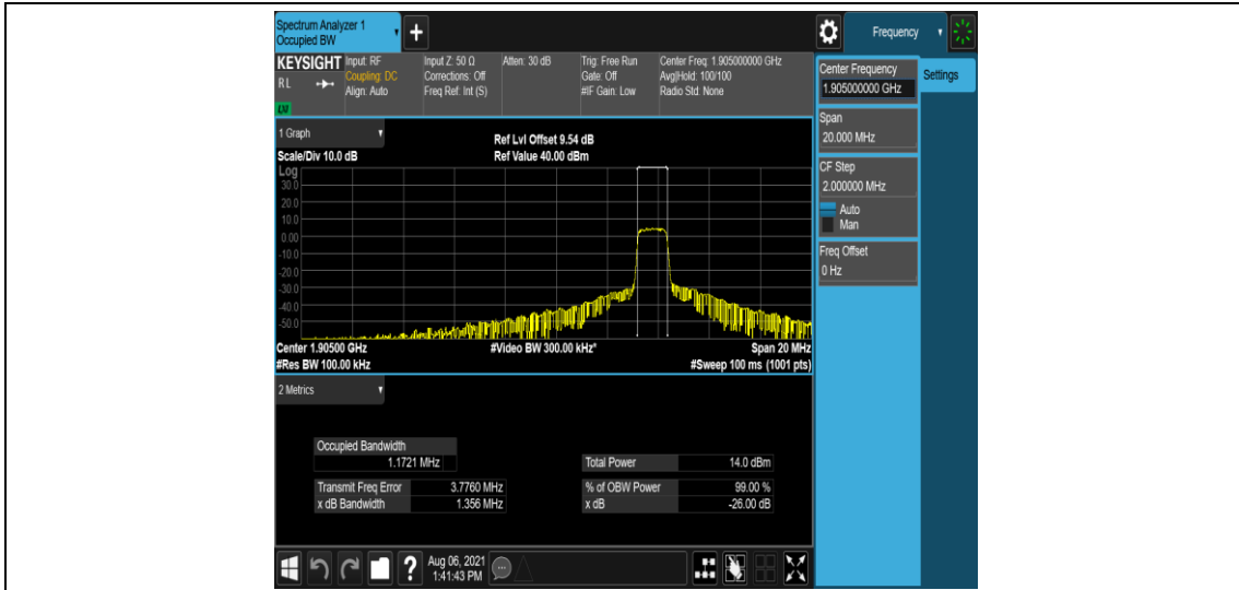
Band2-10MHz-16QAM-19150-6-0-High-1.1721-1.356-PASS
