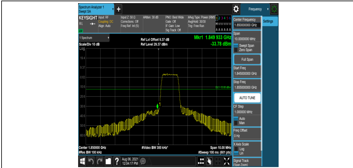
Band2-5MHz-QPSK-18625-6-0-Low--33.78-PASS
