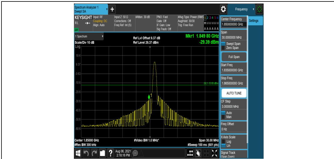
Band2-15MHz-QPSK-18675-1-0-Low--29.39-PASS
