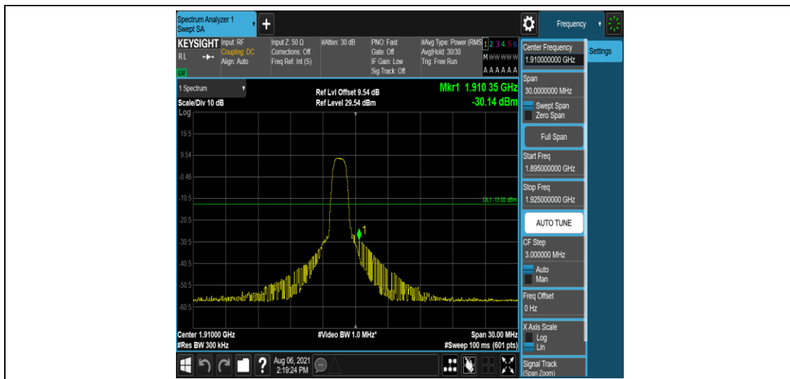
Band2-15MHz-QPSK-19125-6-0-High--30.14-PASS
