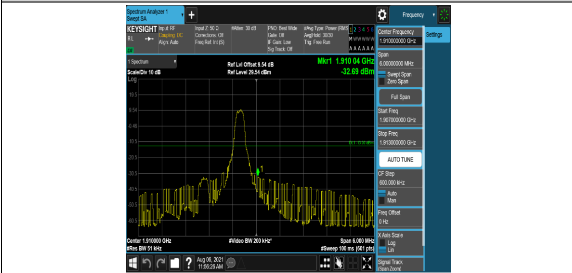
Band2-3MHz-QPSK-19185-1-5-High--32.69-PASS
