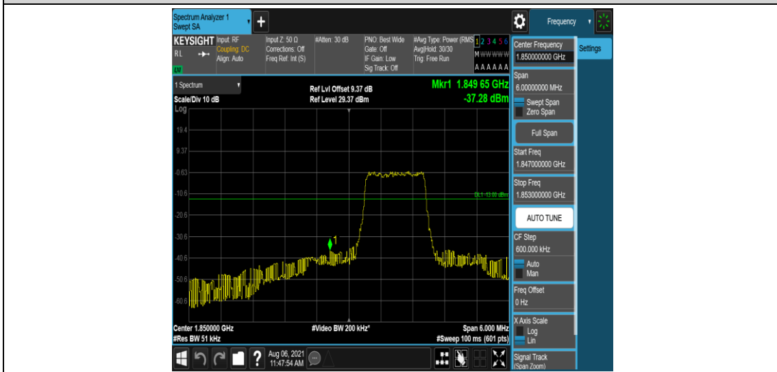
Band2-3MHz-16QAM-18615-6-0-Low--37.28-PASS
