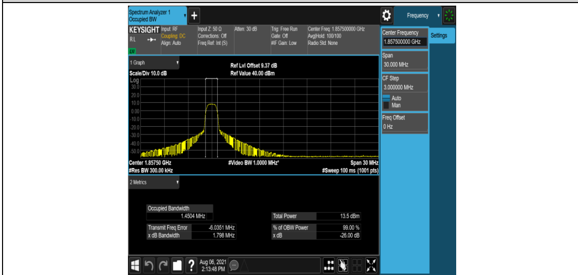
Band2-15MHz-QPSK-18675-6-0-Low-1.4504-1.798-PASS
