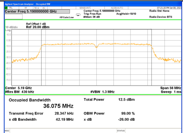
W52_11ac40_Lower_26BW and 99%
