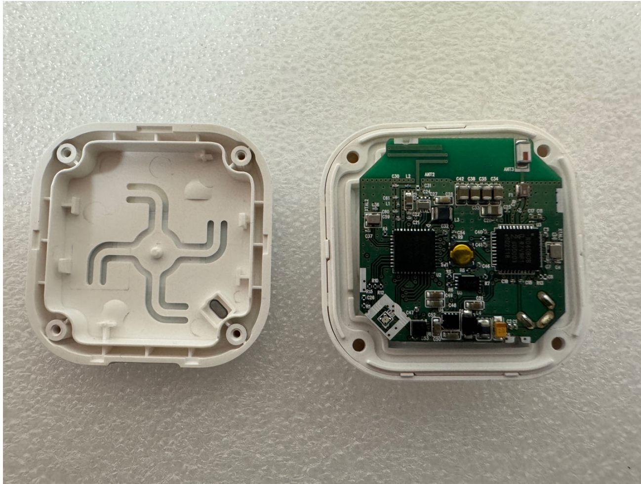
[ Inside View ]
