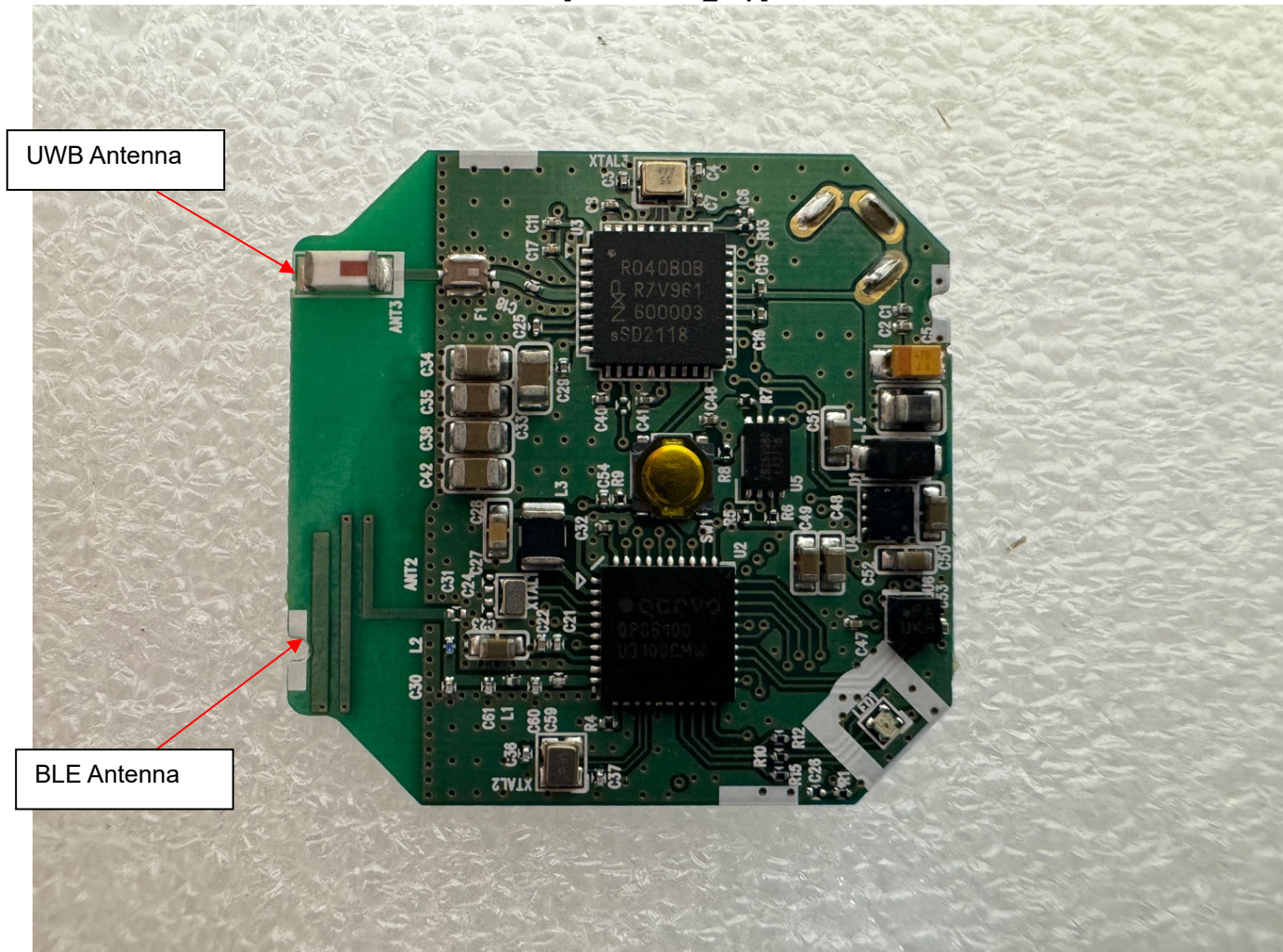
[Main board_Top]
