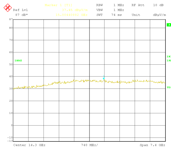
Vertical(Above 10 600 MHz)
