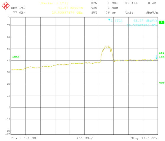
Horizontal(3 100-10 600 MHz)
