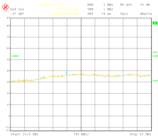
Horizontal(Above 10 600 MHz)
