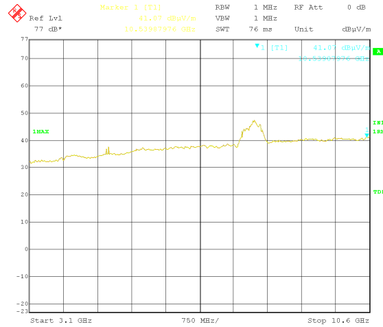
Vertical(3 100-10 600 MHz)
