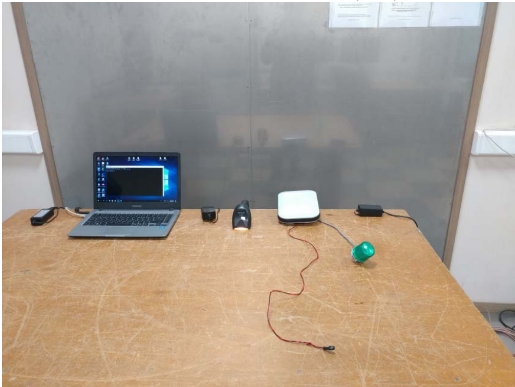
Conducted emission measurement (Front)
