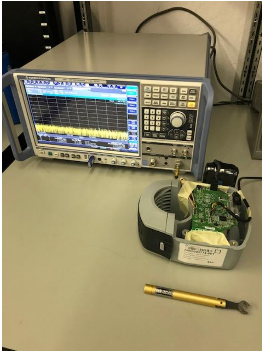
Figure 1: Test Setup for conducted measurements at internal u.fl connector
