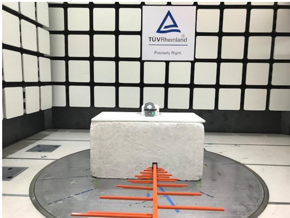
Figure 6: Test Setup for 30 MHz to 1 GHz (Front View)
