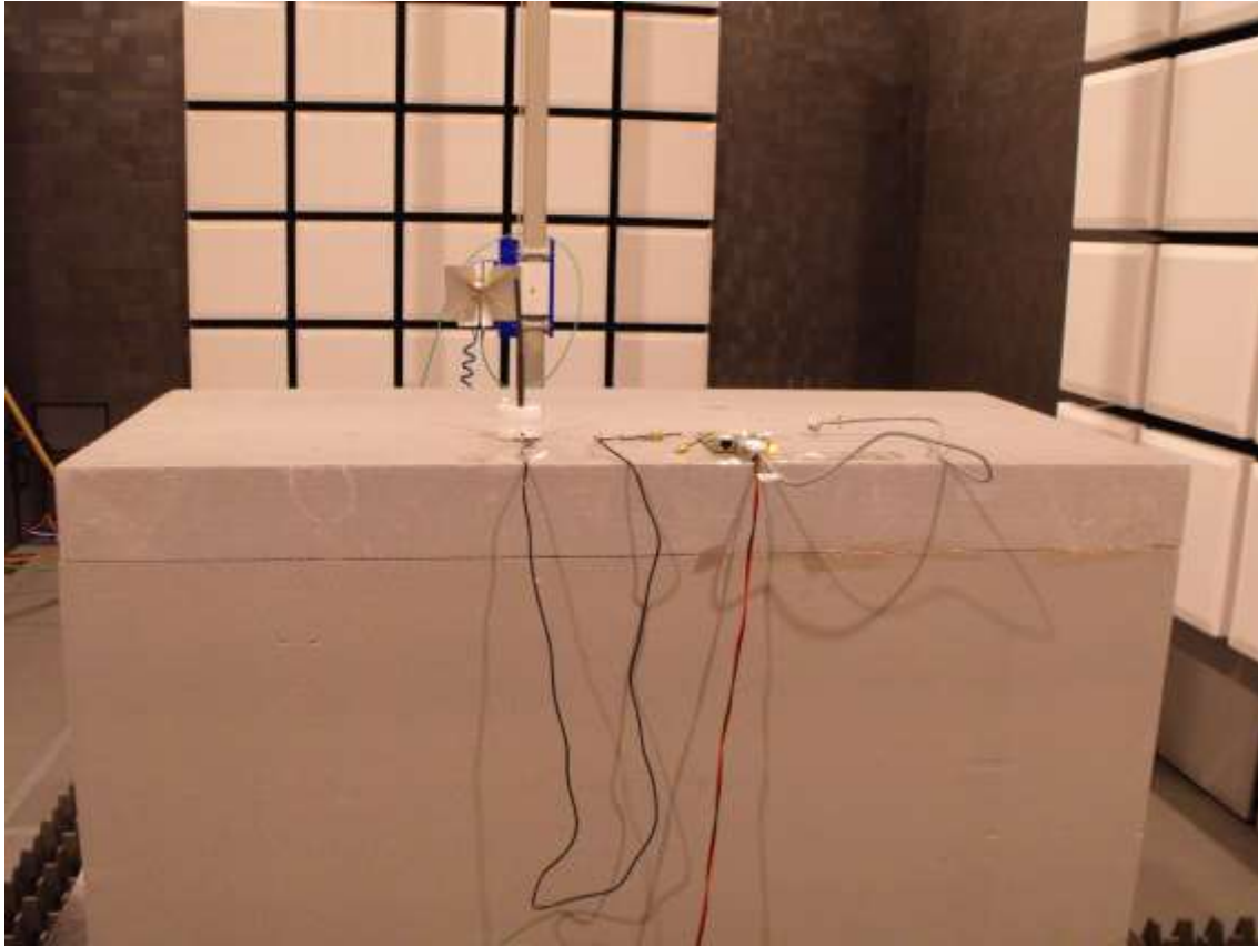
Figure 7: Radiated emission test, 1 GHz – 10 GHz
