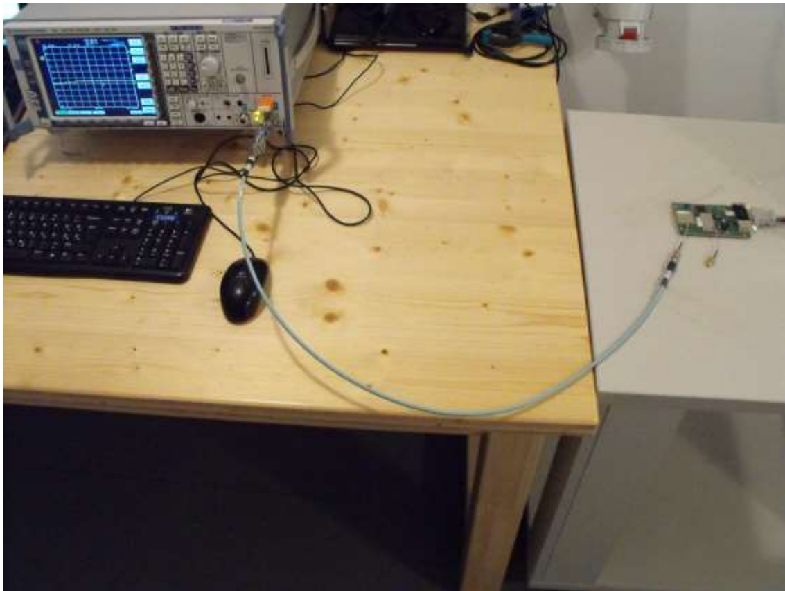
Figure 8: RF Conducted testing
