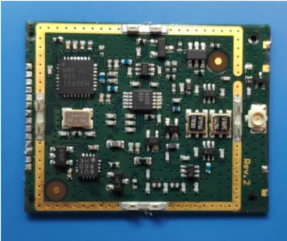
Figure 6: LXNAV Application module 2 - Diversity, top side, without RF shield
