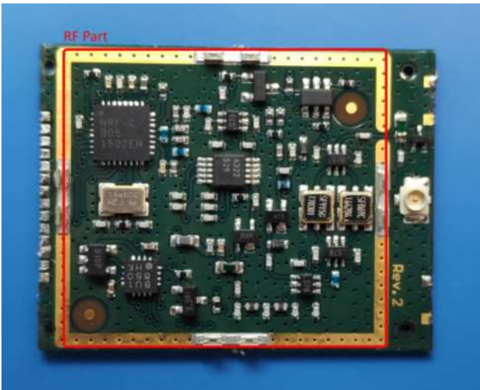
Figure 7: LXNAV Application module 2 - Diversity, top side, RF part
