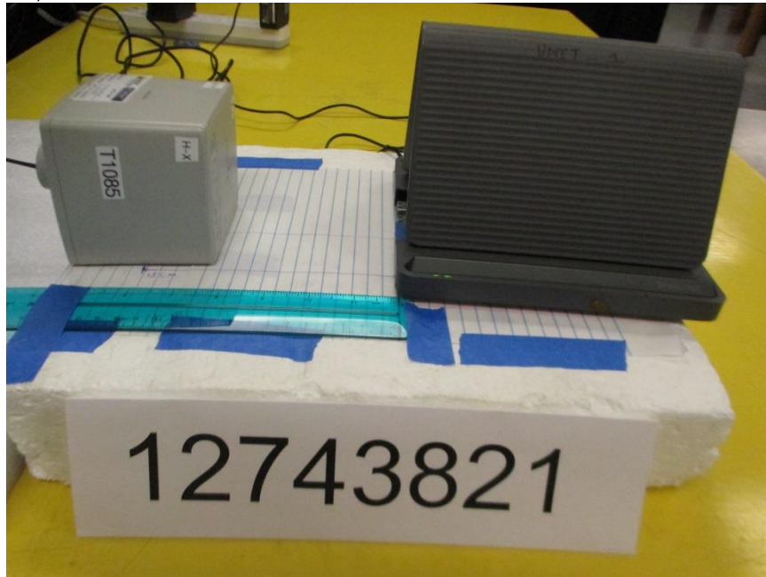
S2, RF EXPOSURE SETUP PHOTO
