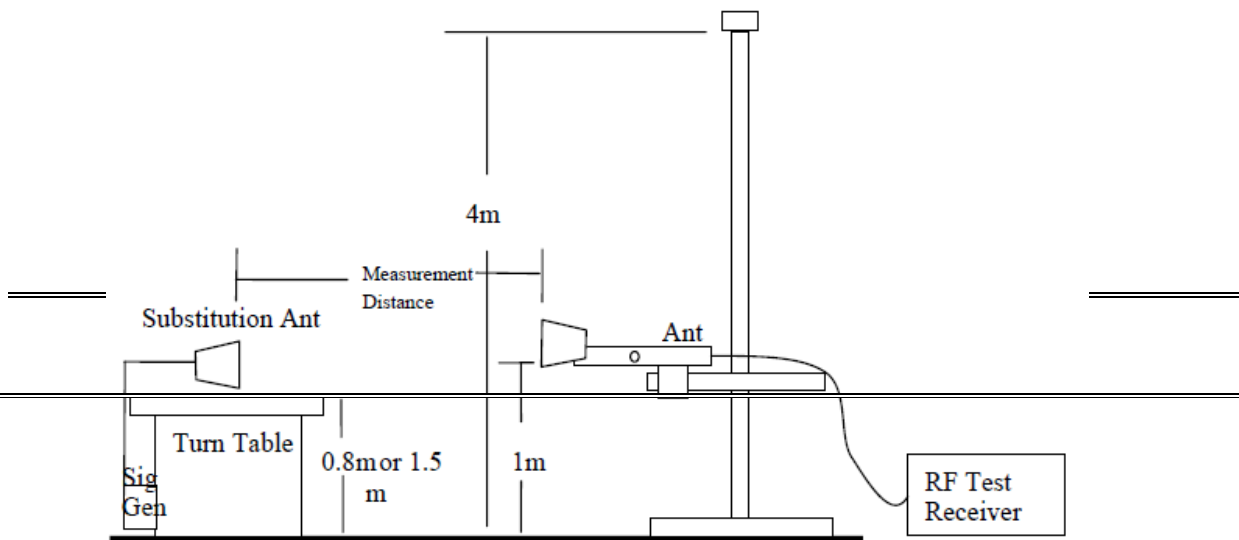
Figure 6—Test site-up for radiated ERP and/or EIRP measurements
