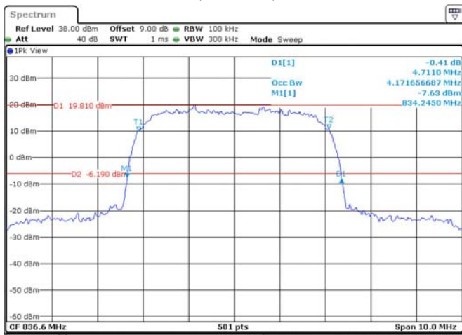
WCDMA Band V, HSDPA, Middle Channel
