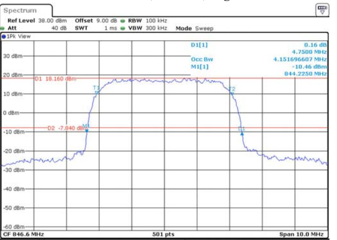
WCDMA Band V, HSDPA, High Channel
