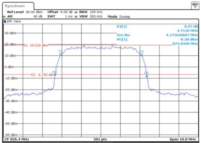
WCDMA Band V, HSDPA, Low Channel
