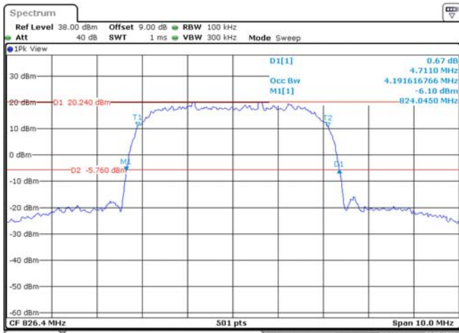
WCDMA Band V, Rel99, Low Channel
