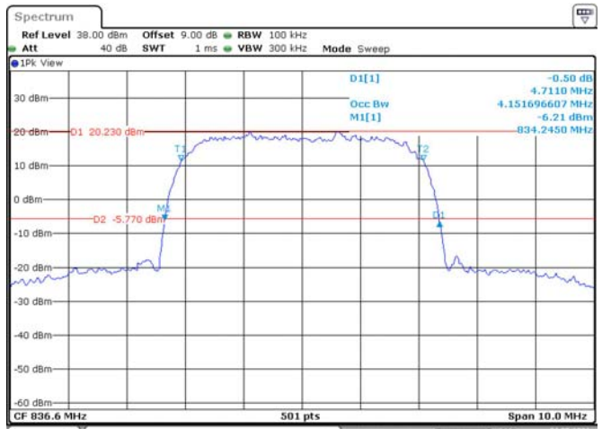
WCDMA Band V, Rel99, Middle Channel
