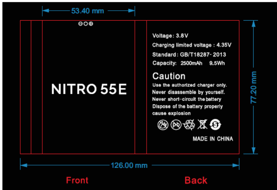
Battery label
