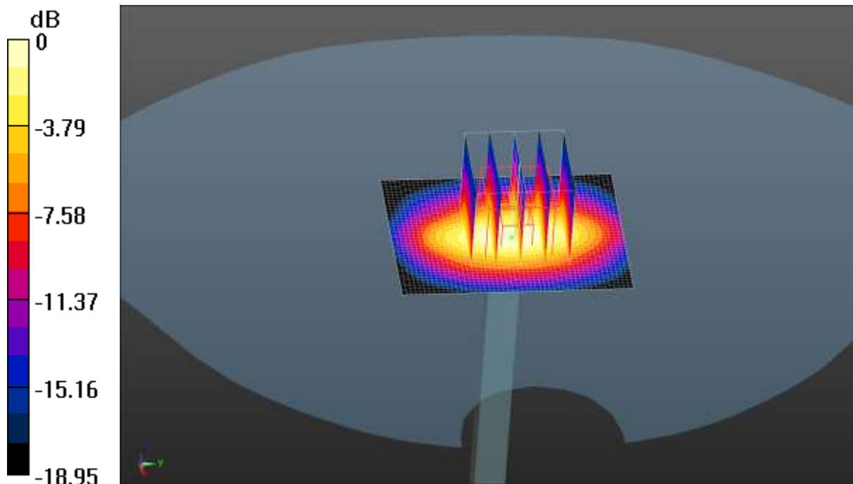
0 dB = 2.15 W/kg = 3.32 dBW/kg
