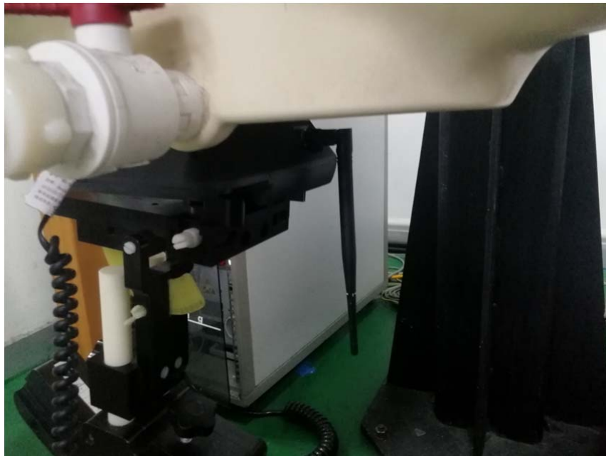
Body (Worn) Back With Antenna Vertical Setup Photo (0mm)
