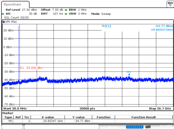
5MHz_Middle_QPSK_1@0(30MHz~26.7GHz)
