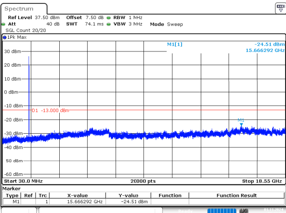
3MHz_High_QPSK_1@0(30MHz~18.55GHz)
