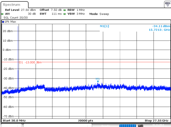
2_10MHz_High_QPSK_1@0(30MHz~27.55GHz)
