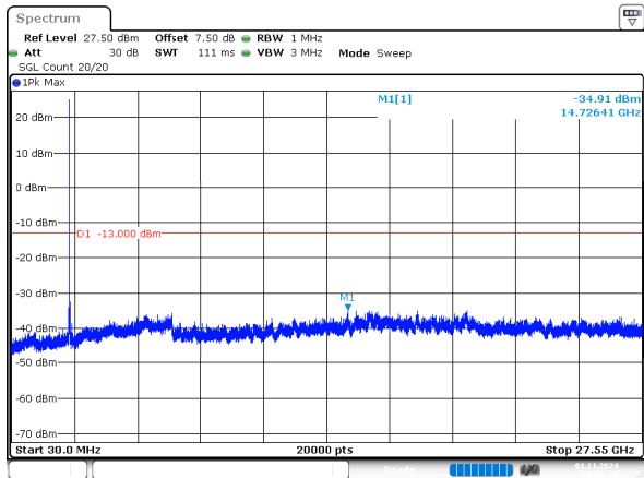
2_15MHz_Low_QPSK_1@0(30MHz~27.55GHz)
