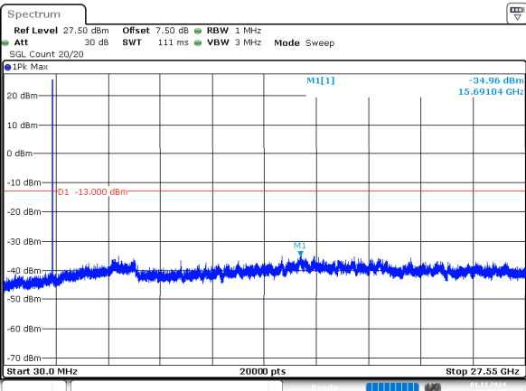
2_10MHz_Middle_QPSK_1@0(30MHz~27.55GHz)
