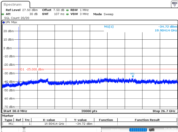
5MHz_Low_QPSK_1@0(30MHz~26.7GHz)
