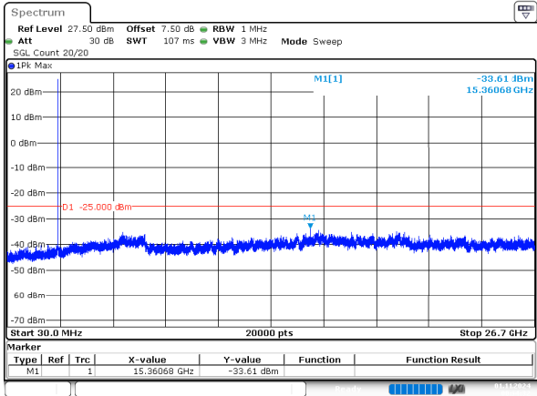
10MHz_High_QPSK_1@0(30MHz~26.7GHz)
