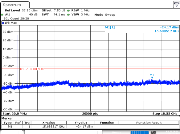
3MHz_Low_QPSK_1@0(30MHz~18.55GHz)
