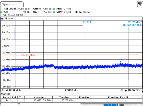
3MHz_Middle_QPSK_1@0(30MHz~18.55GHz)
