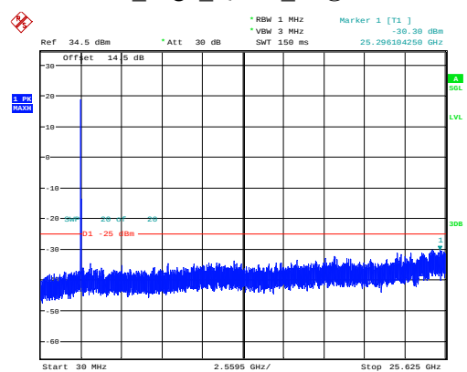
15MHz_High_QPSK_75@0 -30.30dBm
