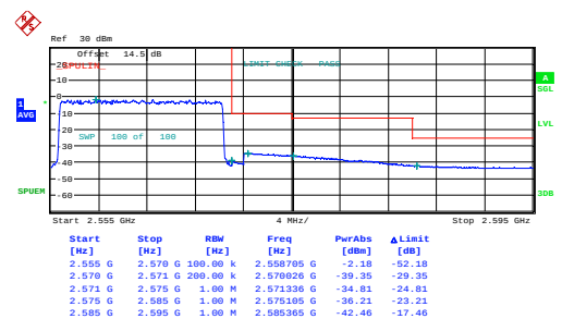
15MHz_High_16QAM_75@0
