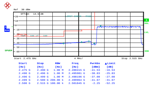
15MHz_Low_16QAM_75@0
