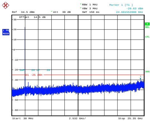
10MHz_Middle_QPSK_1@0 -29.63dBm
