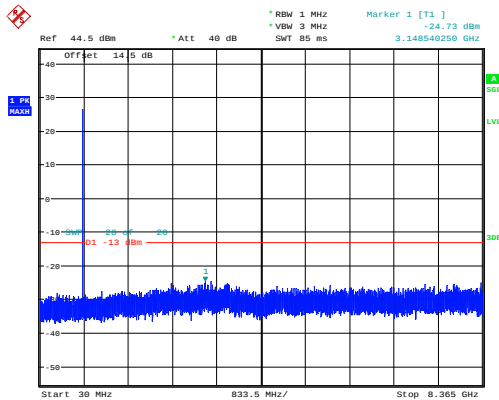
1.4MHz_Middle_QPSK_1@0 -24.73dBm
