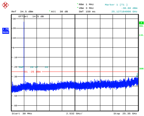
20MHz_Middle_QPSK_1@0 -30.60dBm
