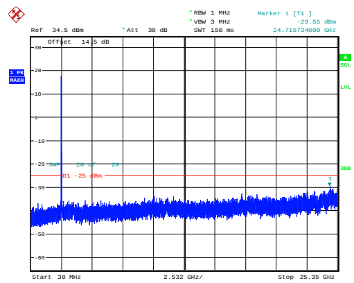
15MHz_Middle_QPSK_75@0 -29.55dBm
