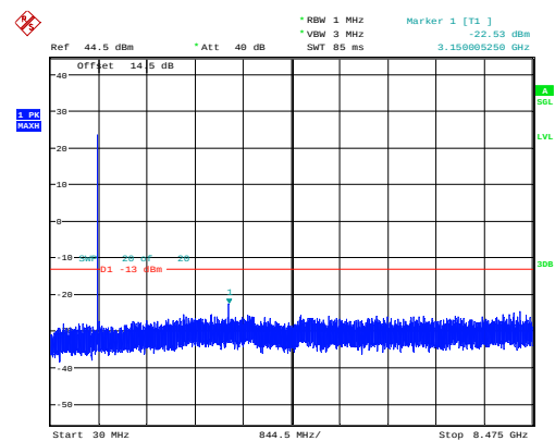
3MHz_High_QPSK_15@0 -22.53dBm
