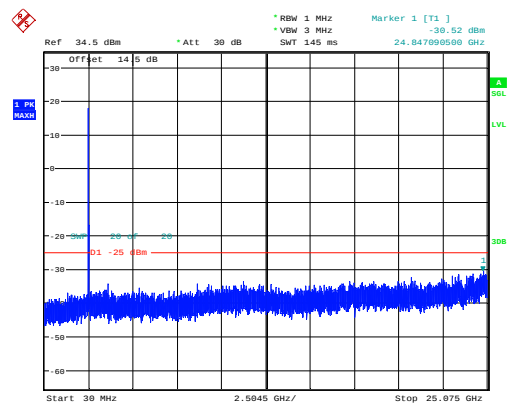
15MHz_Low_QPSK_75@0 -30.52dBm
