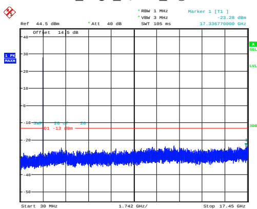
20MHz_High_QPSK_1@0 -23.28dBm
