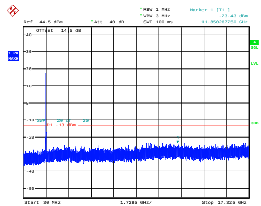
20MHz_Middle_QPSK_100@0 -23.43dBm
