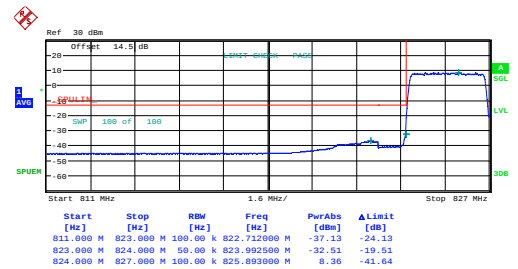
3MHz_Low_QPSK_15@0
