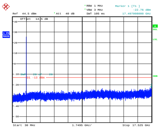
5MHz_High_QPSK_1@0 -22.76dBm
