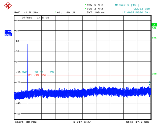
20MHz_Low_QPSK_100@0 -22.83dBm
