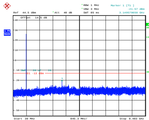
1.4MHz_High_QPSK_6@0 -21.57dBm
