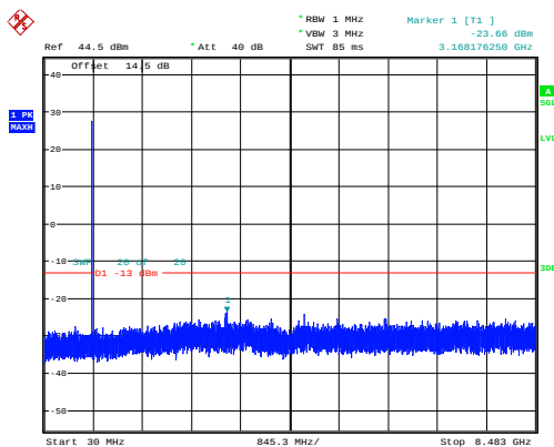
1.4MHz_High_QPSK_1@0 -23.66dBm
