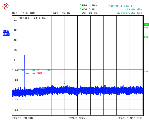
10MHz_Middle_QPSK_1@0 -24.64dBm
