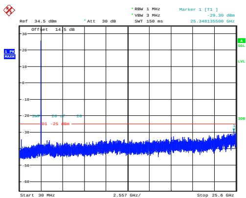
20MHz_High_QPSK_1@0 -29.30dBm
