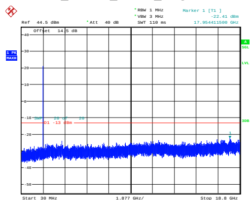
3MHz Middle QPSK 15@0 -22.41dBm
