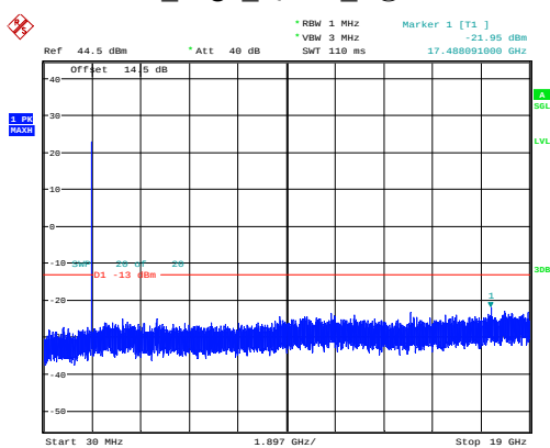
20MHz_High_QPSK_1@0 -21.95dBm
