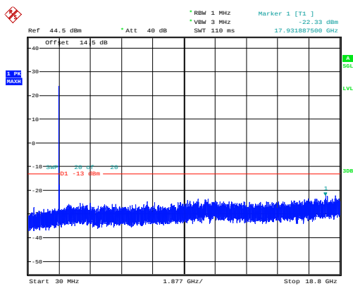
20MHz_Middle_QPSK_1@0 -22.33dBm
