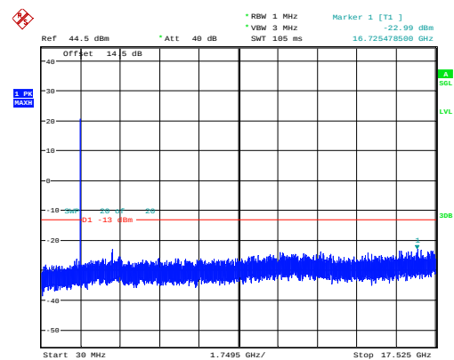
5MHz_High_QPSK_25@0 -22.99dBm
