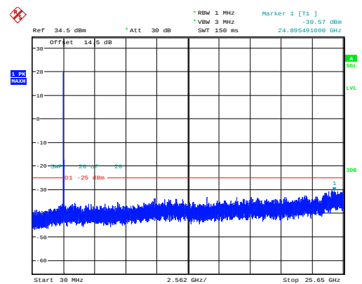
10MHz_High_QPSK_50@0 -30.57dBm
