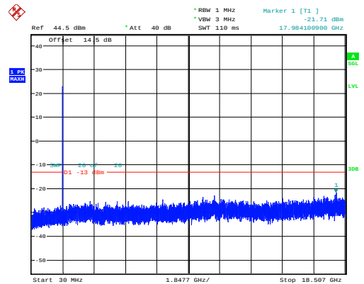
1.4MHz_Low_QPSK_6@0 -21.71dBm
