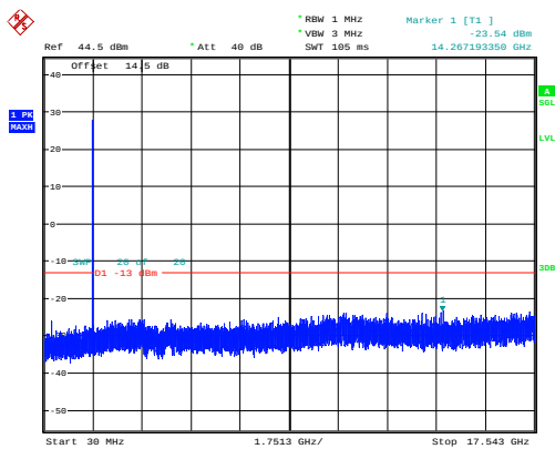
1.4MHz_High_QPSK_1@0 -23.54dBm
