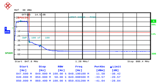
1.4MHz_High_16QAM_6@0
