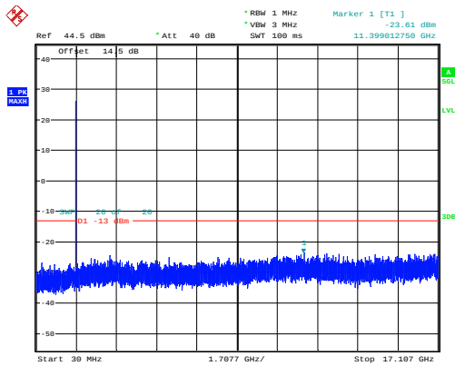
1.4MHz_Low_QPSK_1@0 -23.61dBm
