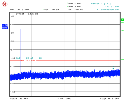
1.4MHz_Middle_QPSK_1@0 -23.37dBm
