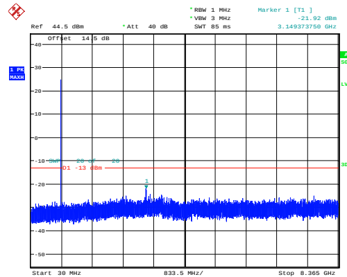
1.4MHz_Middle_QPSK_6@0 -21.92dBm
