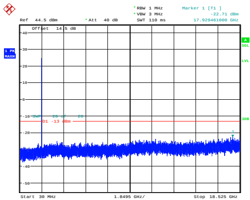
5MHz_Low_QPSK_1@0 -22.71dBm
