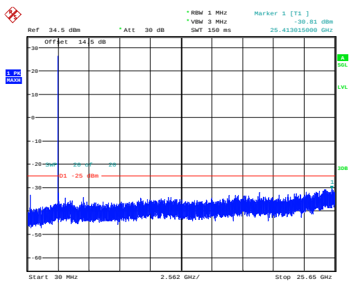
10MHz_High_QPSK_1@0 -30.81dBm
