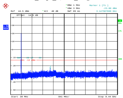
10MHz_High_QPSK_50@0 -23.80dBm
