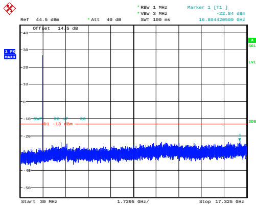
1.4MHz_Middle_QPSK_1@0 -22.84dBm
