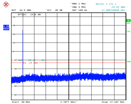
1.4MHz_Low_QPSK_6@0 -23.52dBm
