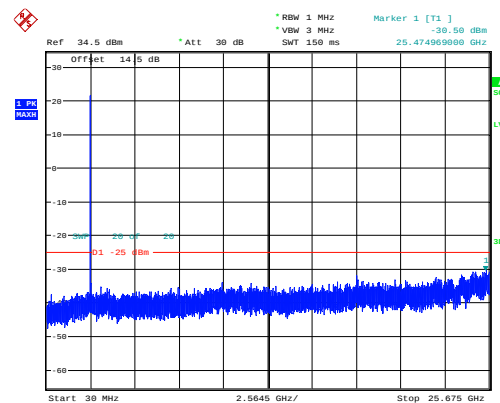
5MHz_High_QPSK_25@0 -30.50dBm
