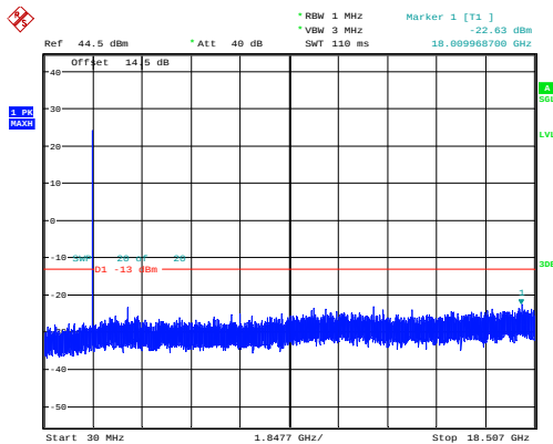
1.4MHz_Low_QPSK_1@0 -22.63dBm
