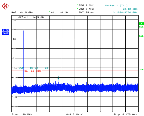
3MHz_High_QPSK_1@0 -22.12dBm
