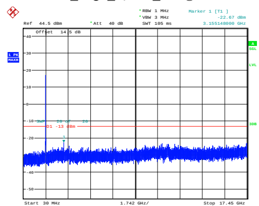
20MHz_High_QPSK_100@0 -22.67dBm
