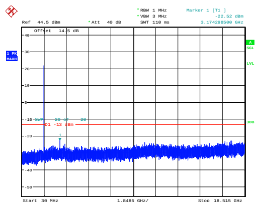
3MHz_Low_QPSK_15@0 -22.52dBm
