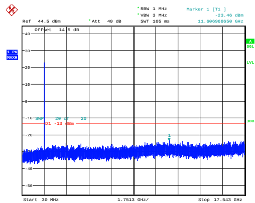
1.4MHz_High_QPSK_6@0 -23.46dBm
