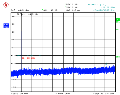
5MHz_High_QPSK_25@0 -22.78dBm
