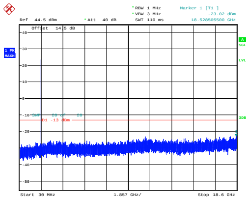
20MHz_Low_QPSK_1@0 -23.02dBm
