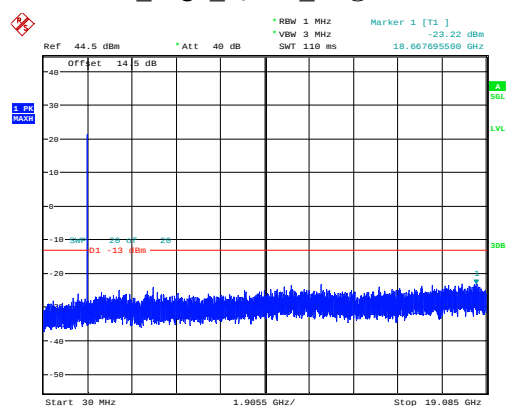
3MHz High QPSK 15@0 -23.22dBm
