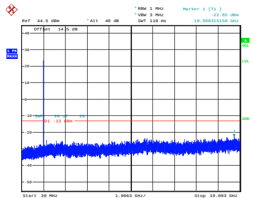
1.4MHz_High_QPSK_6@0 -22.65dBm
