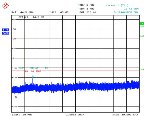
1.4MHz_High_QPSK_1@0 -21.42dBm
