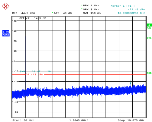
5MHz_High_QPSK_1@0 -22.45dBm
