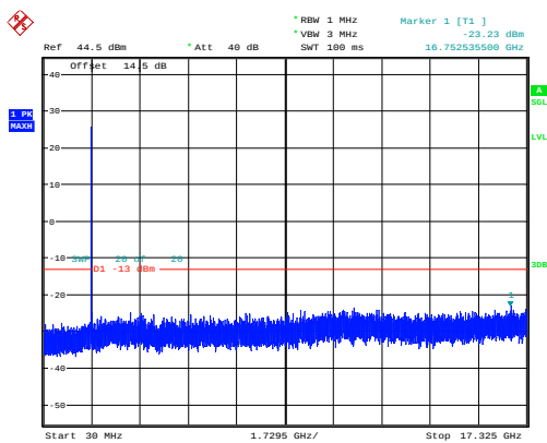
20MHz_Middle_QPSK_1@0 -23.23dBm
