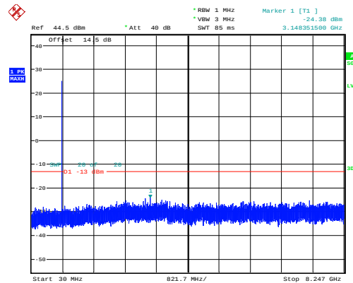
1.4MHz_Low_QPSK_6@0 -24.38dBm
