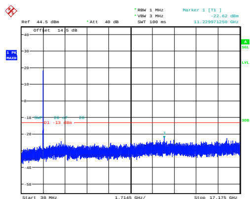
15MHz_Low_QPSK_75@0 -22.62dBm
