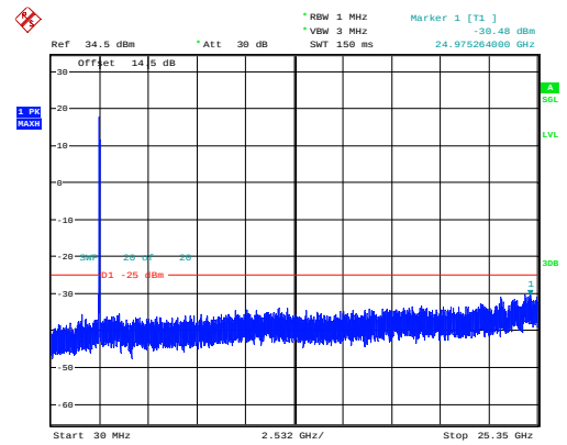
20MHz_Middle_QPSK_100@0 -30.48dBm
