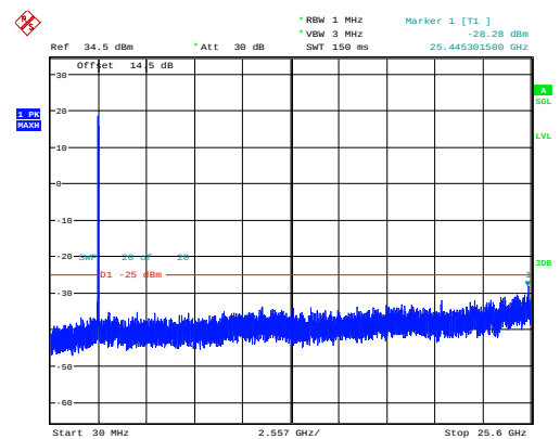
20MHz_High_QPSK_100@0 -28.28dBm
