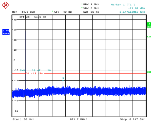
1.4MHz_Low_QPSK_1@0 -21.01dBm
