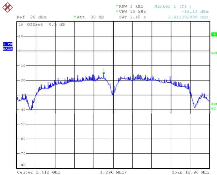
Power Spectral Density, 802.11b Low Channel
