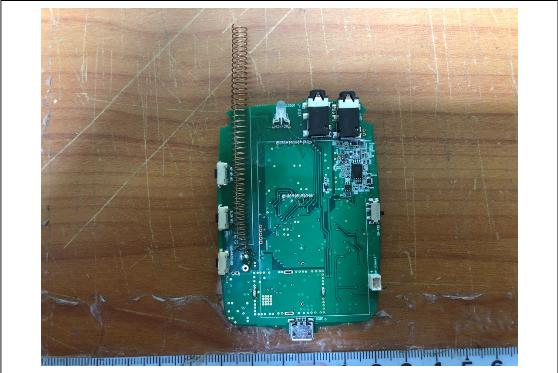
MainBoard-Rear
