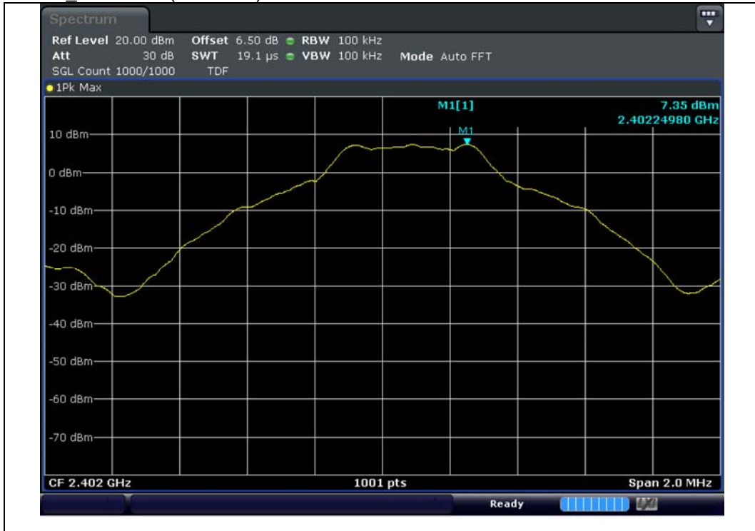
GFSK 2 402 MHz(reference)
