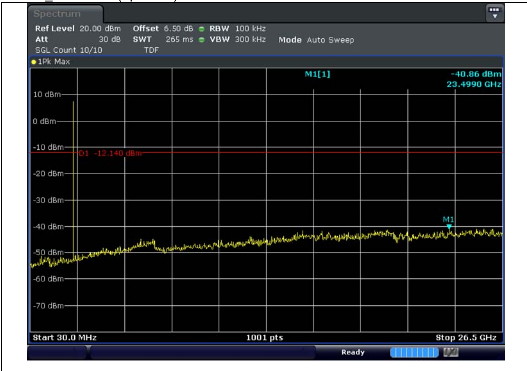
GFSK 2 441 MHz(Spurious)
