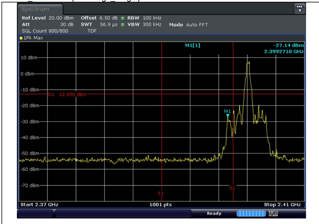
GFSK 2 402 MHz(Bandedge_Single)
