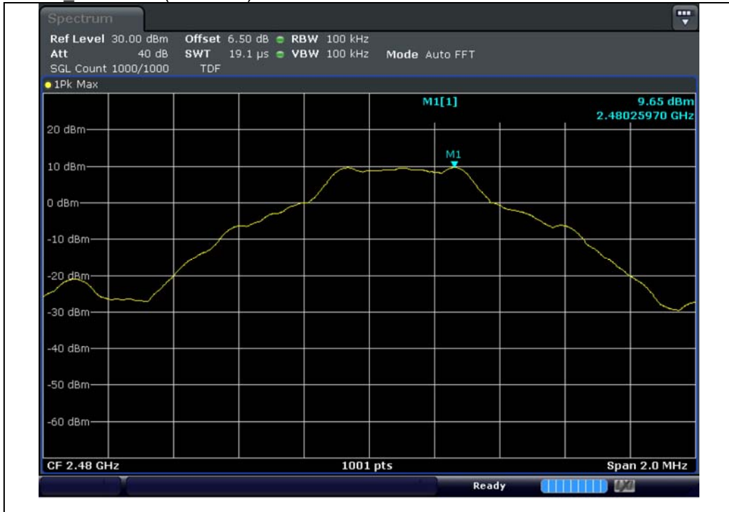
GFSK 2 480 MHz(reference)
