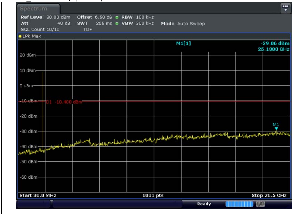
GFSK 2 441 MHz(Spurious)
