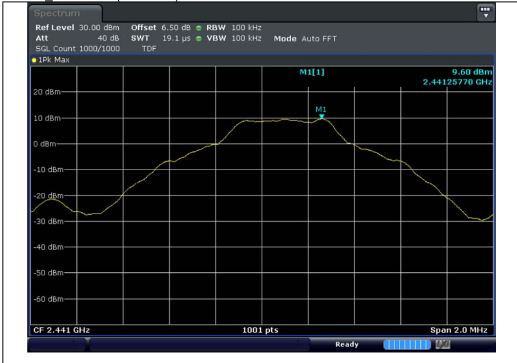
GFSK 2 441 MHz(reference)
