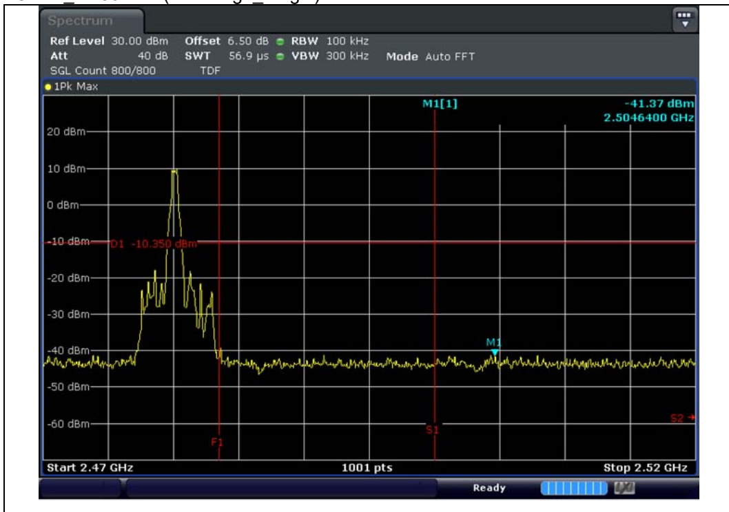
GFSK 2 480 MHz(Bandedge_Single)
