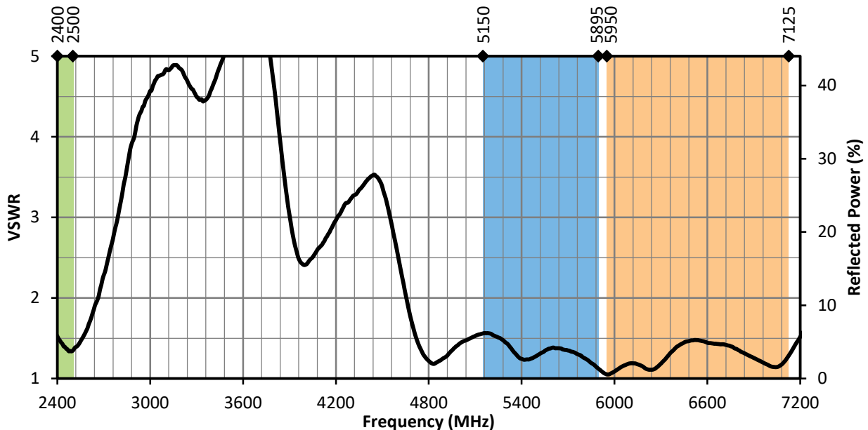
Figure 2. ANT-W63-FPC-LV Antenna VSWR with Frequency Band Highlights
