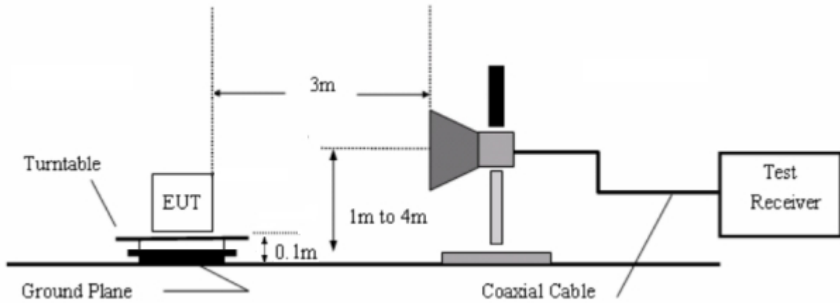
Figure 2. 30MHz to 1GHz
