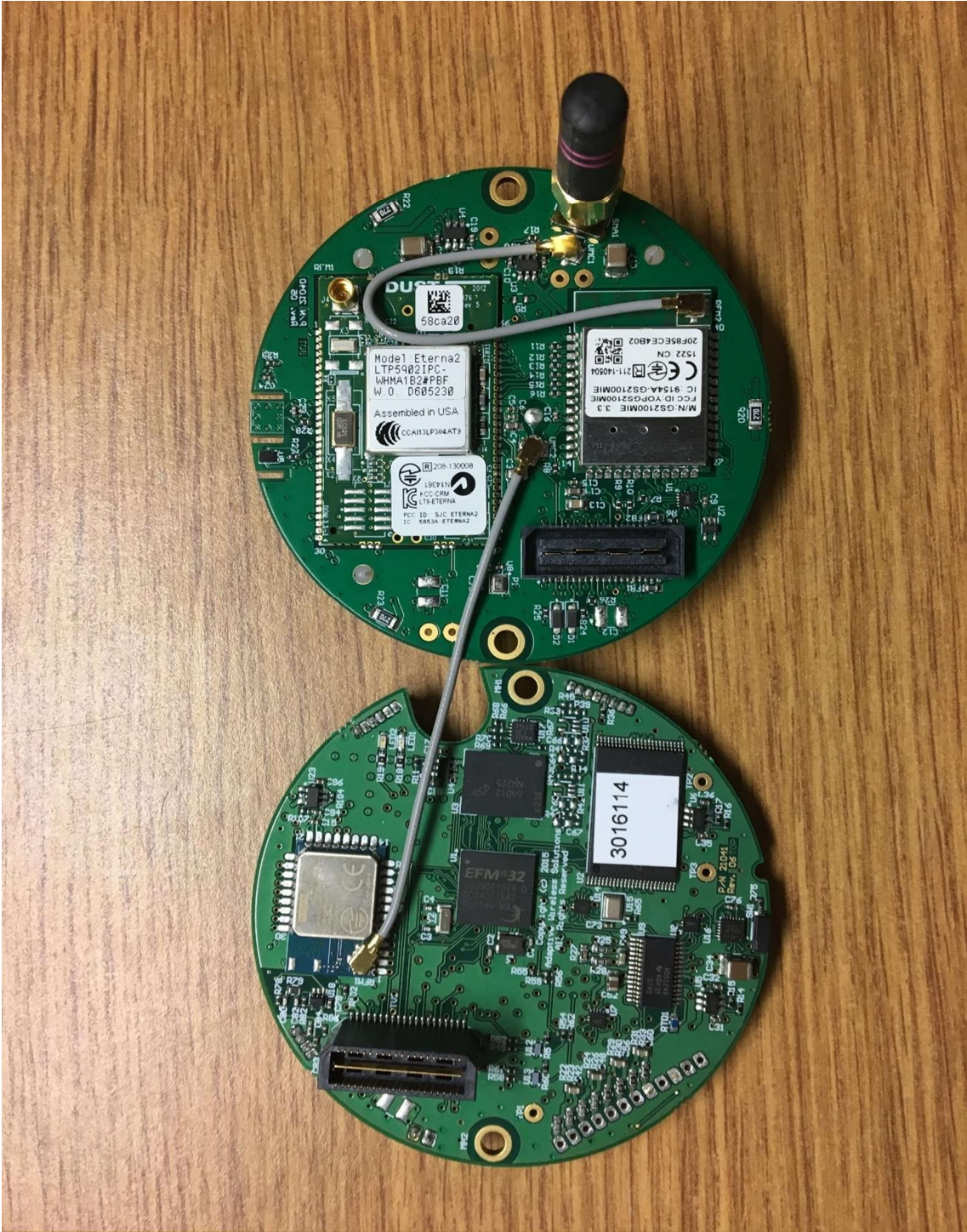
Top of Sensor PCB (lower) & Bottom of RF PCB (upper)
