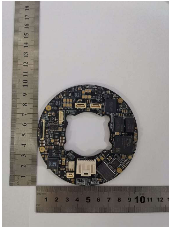
(39) EUT Photo (HSM5_BMB_V2.9)
