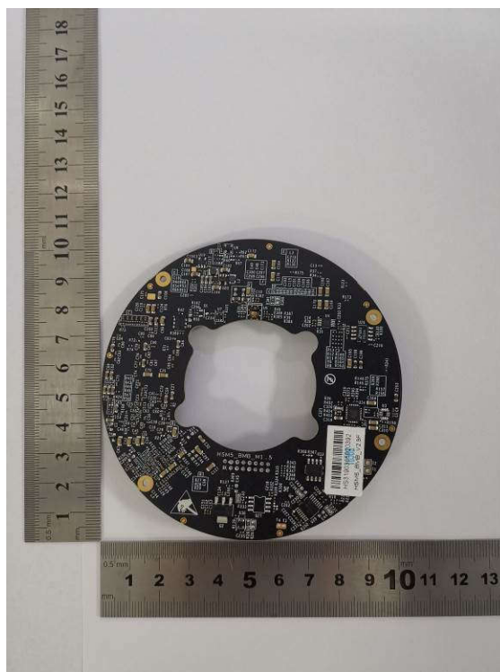
(40) EUT Photo (HSM5_BMB_V2.9)
