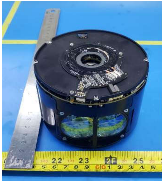
(21) EUT Photo (Pandar64)
