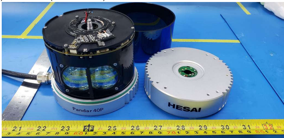
(22) EUT Photo (Pandar40 2.0)
