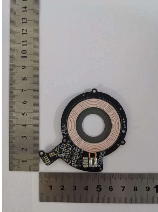
(33) EUT Photo (WLCHG_RX_V2.3)
