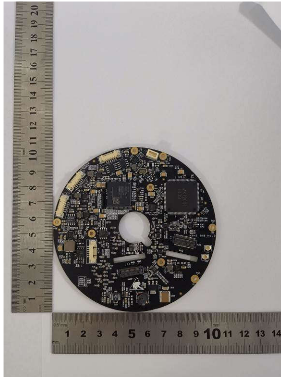
(35) EUT Photo (HSM5_TMB_V3.2)
