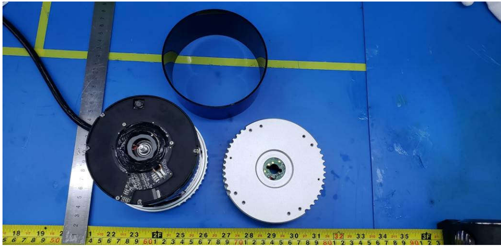
(23) EUT Photo (Pandar40 2.0)
