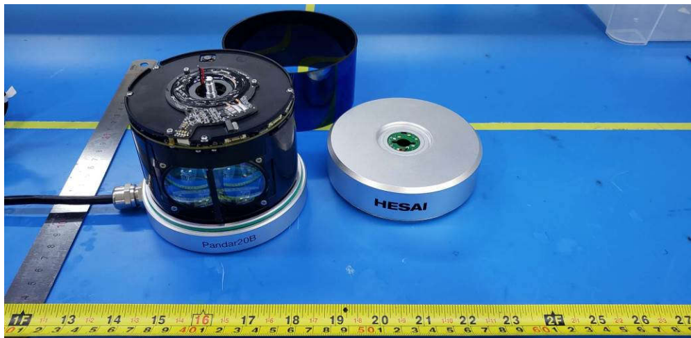
(28) EUT Photo (Pandar20B)
