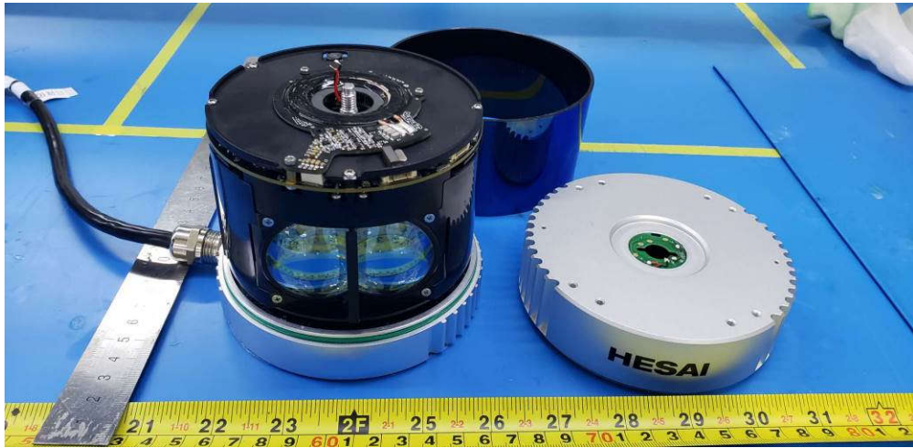
(19) EUT Photo (Pandar64)
