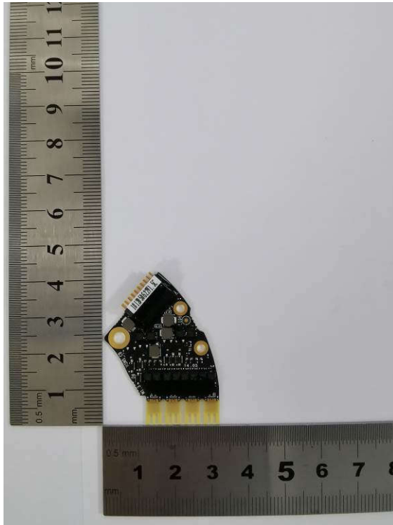
(37) EUT Photo (HSM5_CB_V1.5)
