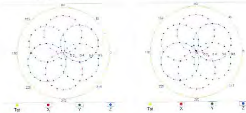
f=600 MHz,TEM
