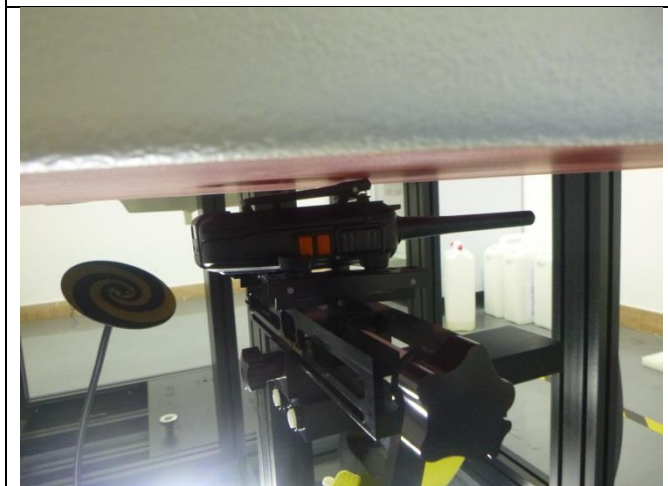
Body-worn(0mm)
