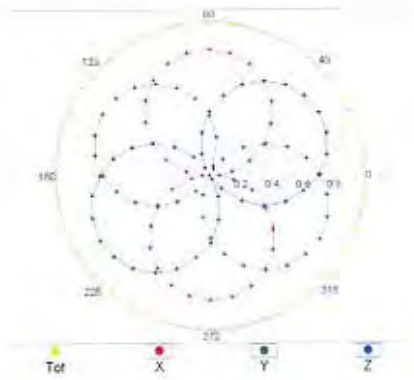
f=600 MHz,TEM
