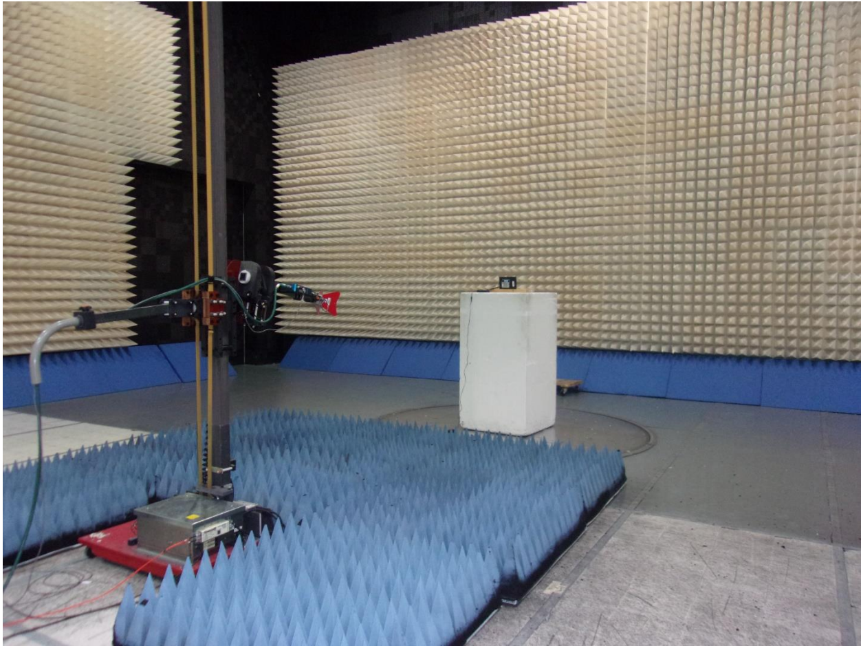
Figure 3: Radiated spurious emissions, 1 GHz – 18 GHz
