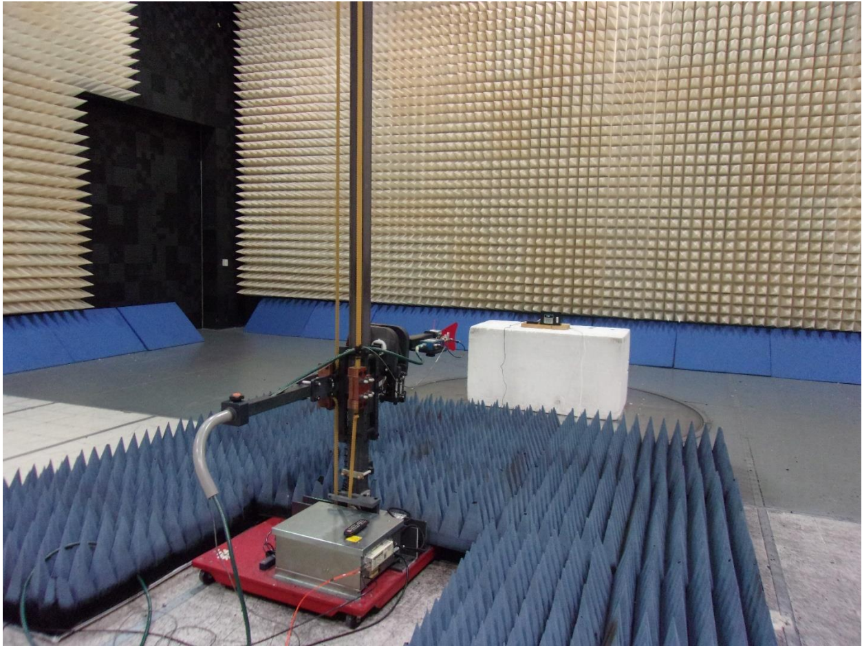
Figure 4: Unintentional emissions, 1 GHz – 18 GHz
