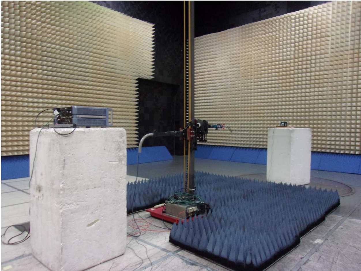
Figure 5: Radiated spurious emissions, 18 GHz – 40 GHz
