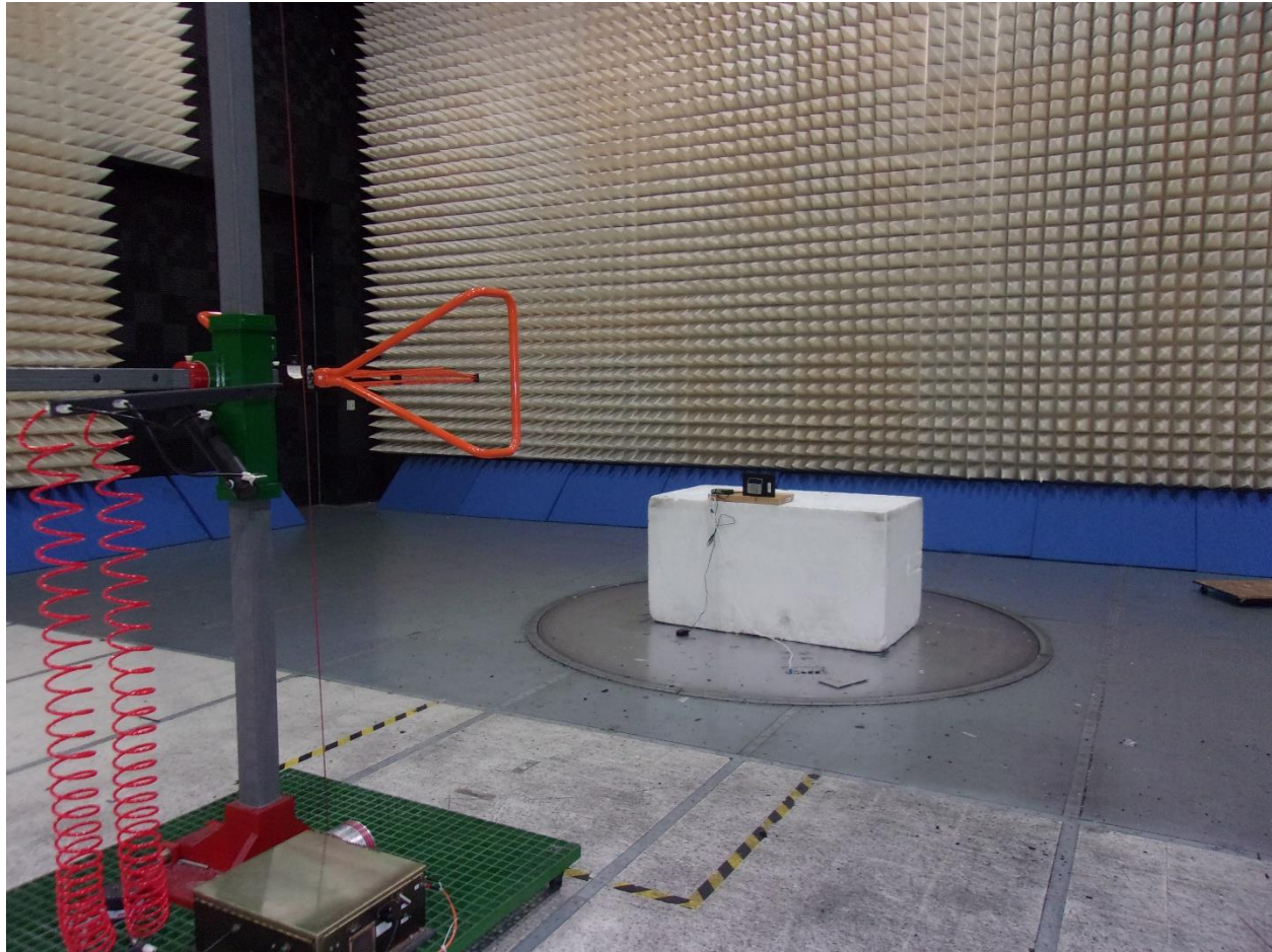
Figure 2: Unintentional and Radiated Spurious Emissions, 30MHz – 1 GHz
