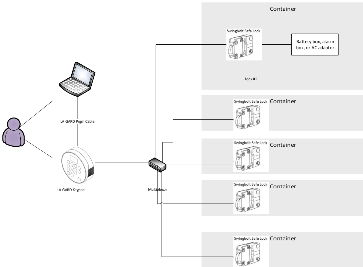
Figure 2 – Multi-Lock System
