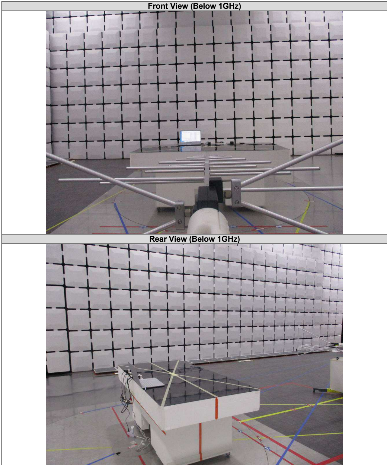
Figure 1. Radiated emission
