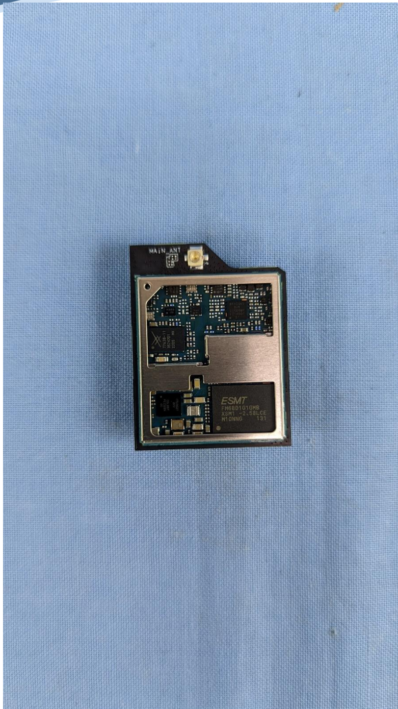
LTE Card Top View Shield Removed
