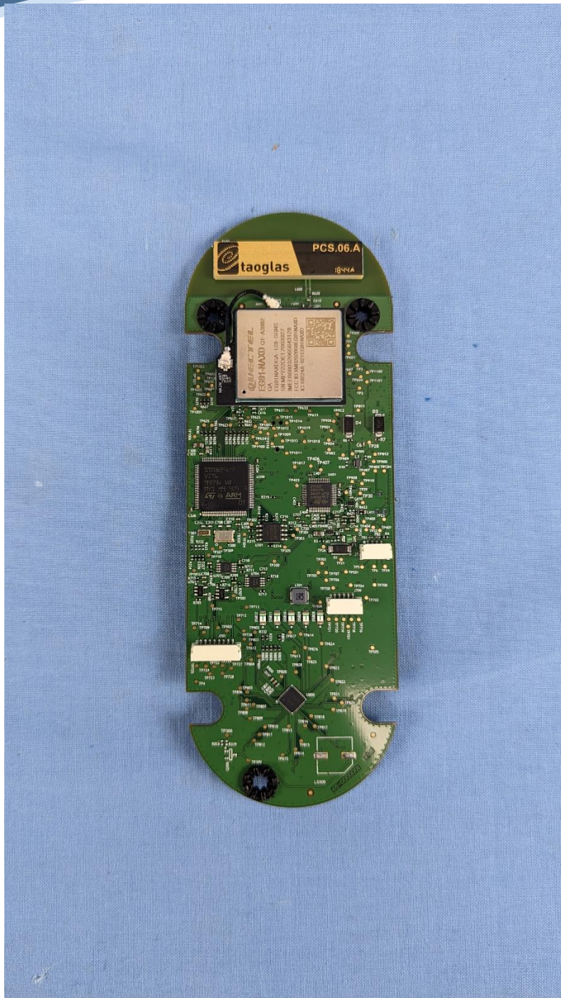
PCBA Top View LTE card Installed
