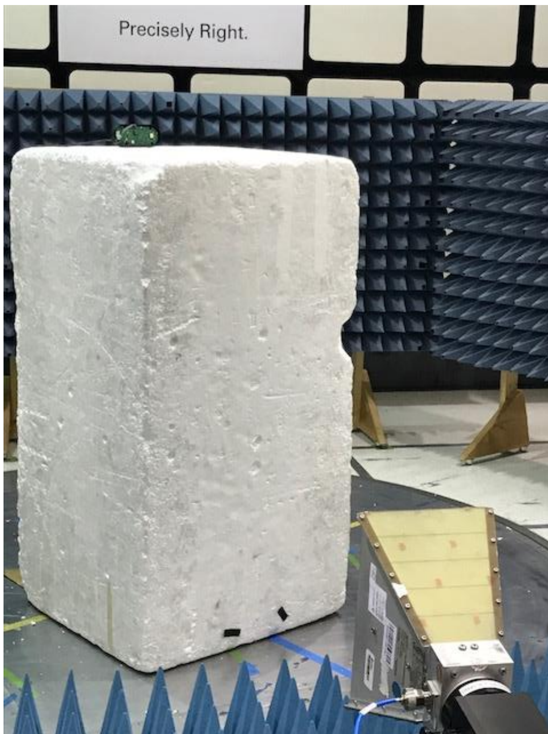
Test Setup 1-18G Front
