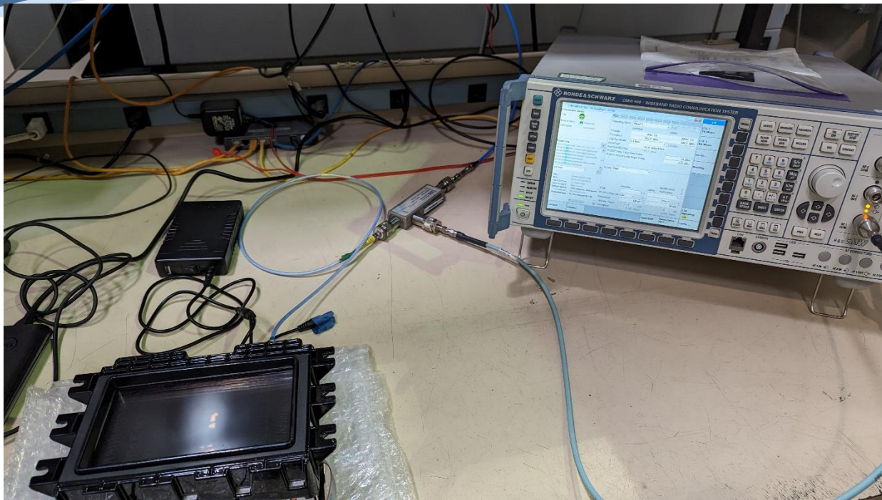
RF Conducted
