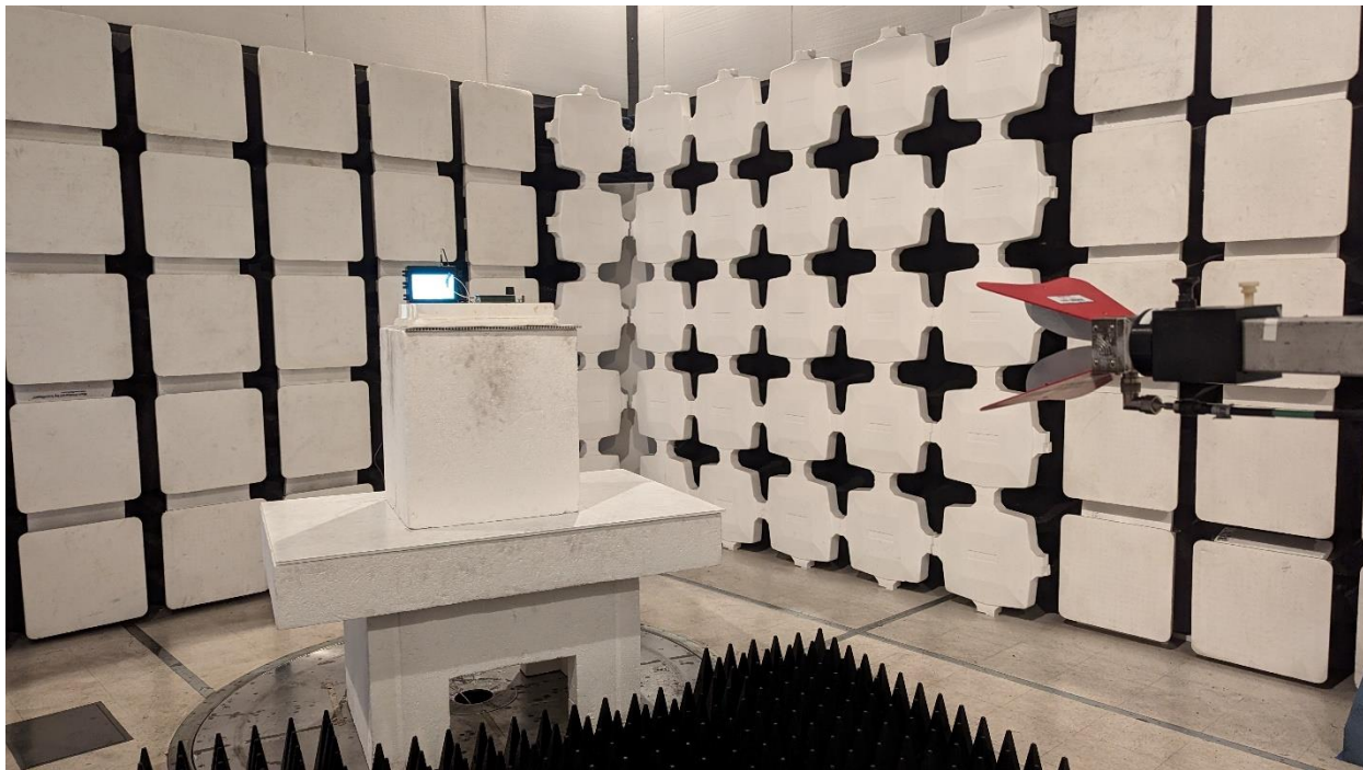
LTE Spurious
