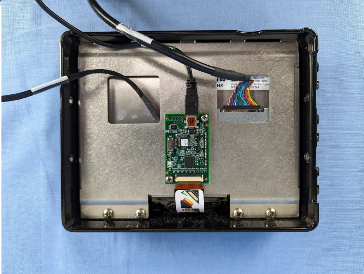
Display Back in Housing
