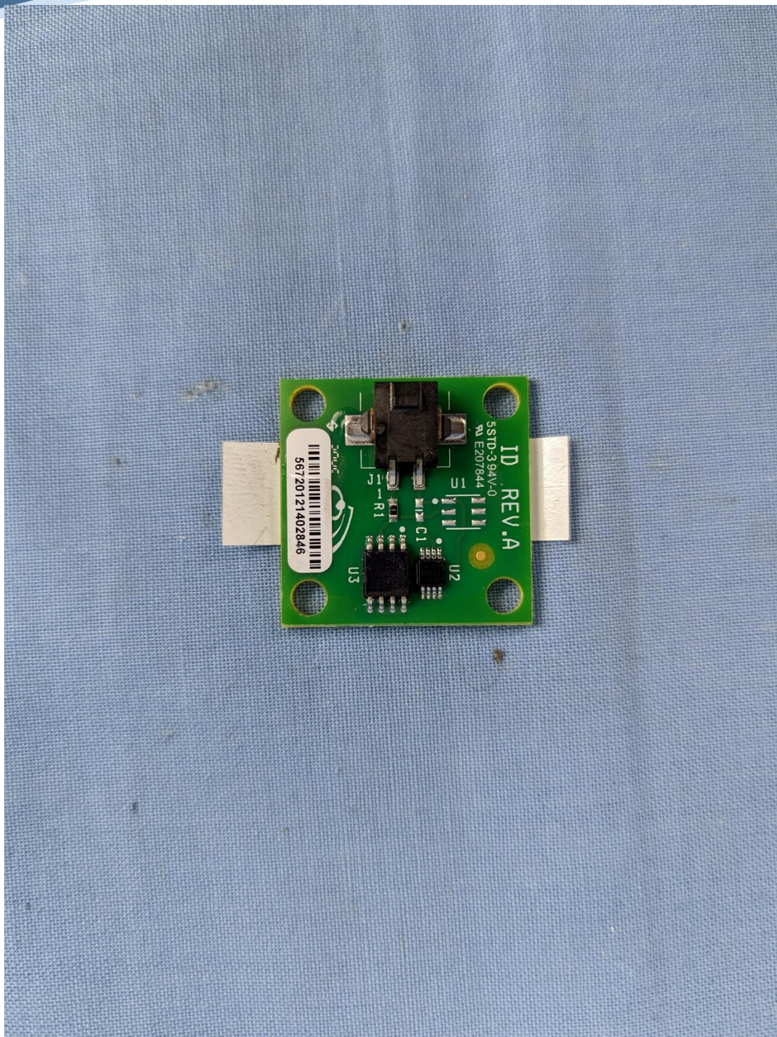
NFC Antenna Board
