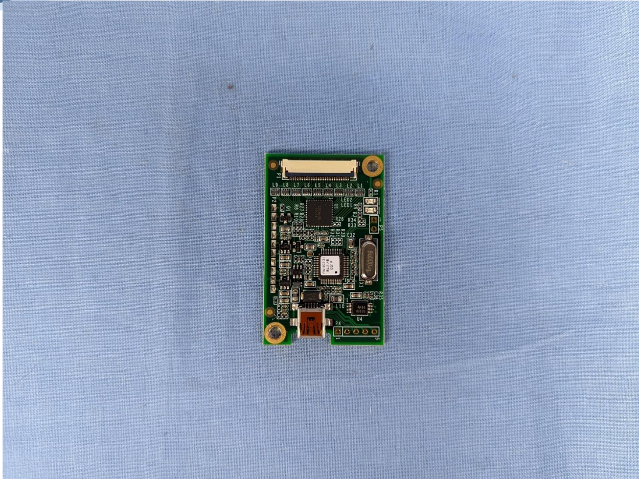
Display IO Board Top
