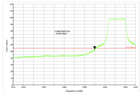
802.11g-Channel 1 Average
