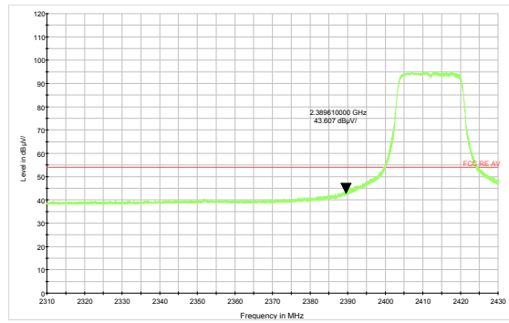
802.11g-Channel 1 Average
