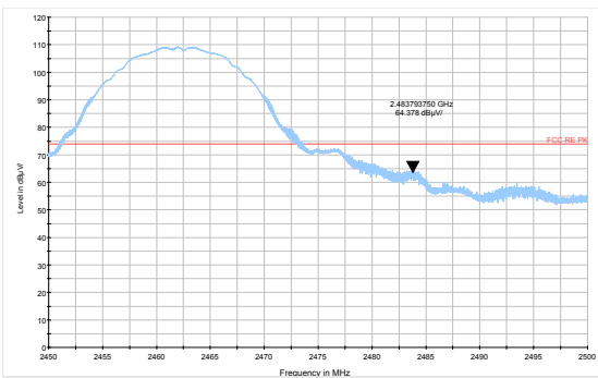
802.11b-Channel 11 Peak
