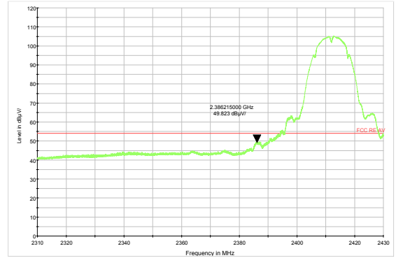
802.11b-Channel 1 Average
