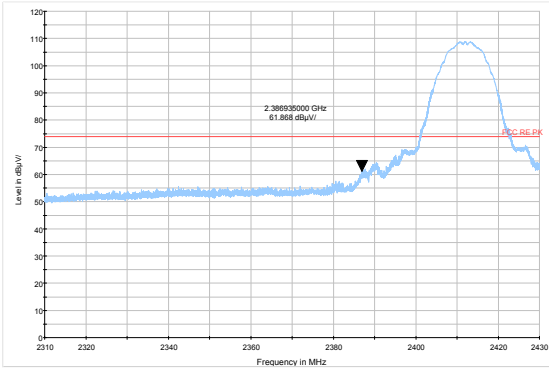
802.11b-Channel 1 Peak
