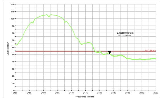
802.11b-Channel 11 Average
