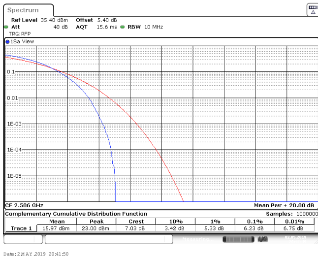
Band41_20MHz_16QAM_40620_27RB#0
