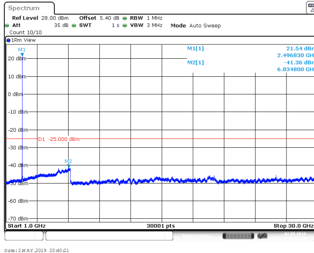
Band41_20MHz_16QAM_40620_1RB#0
