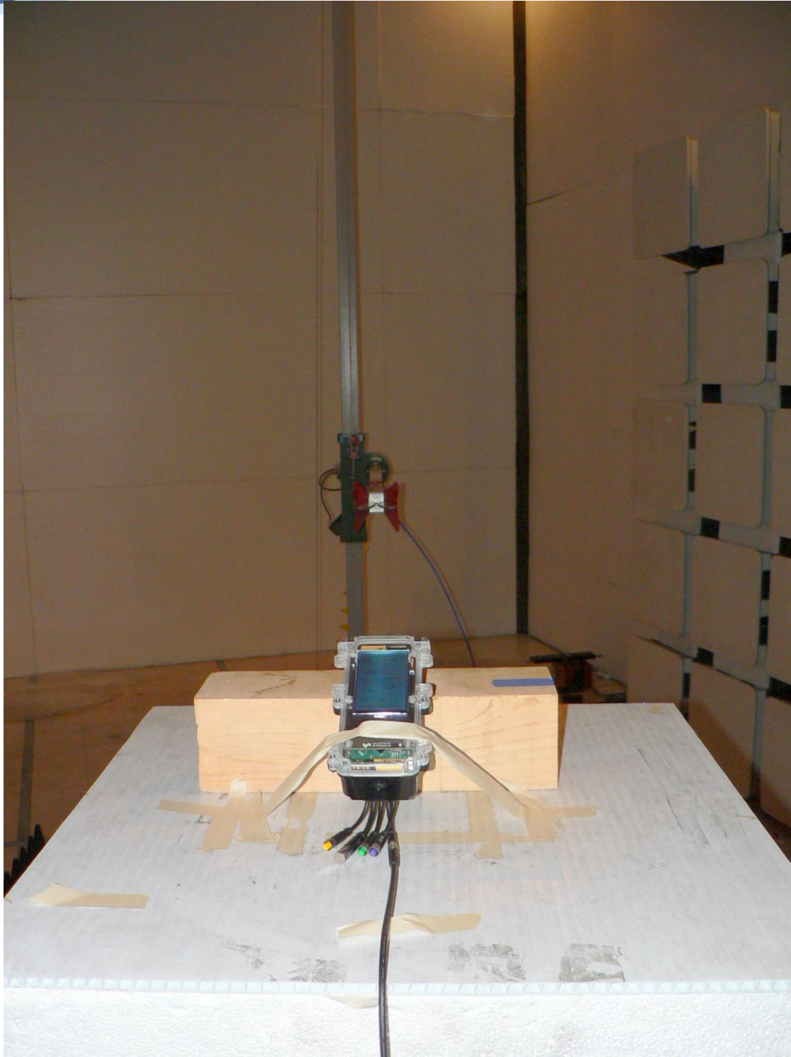
LYFT06 Tx Spurious Emissions 1-18GHz Back
