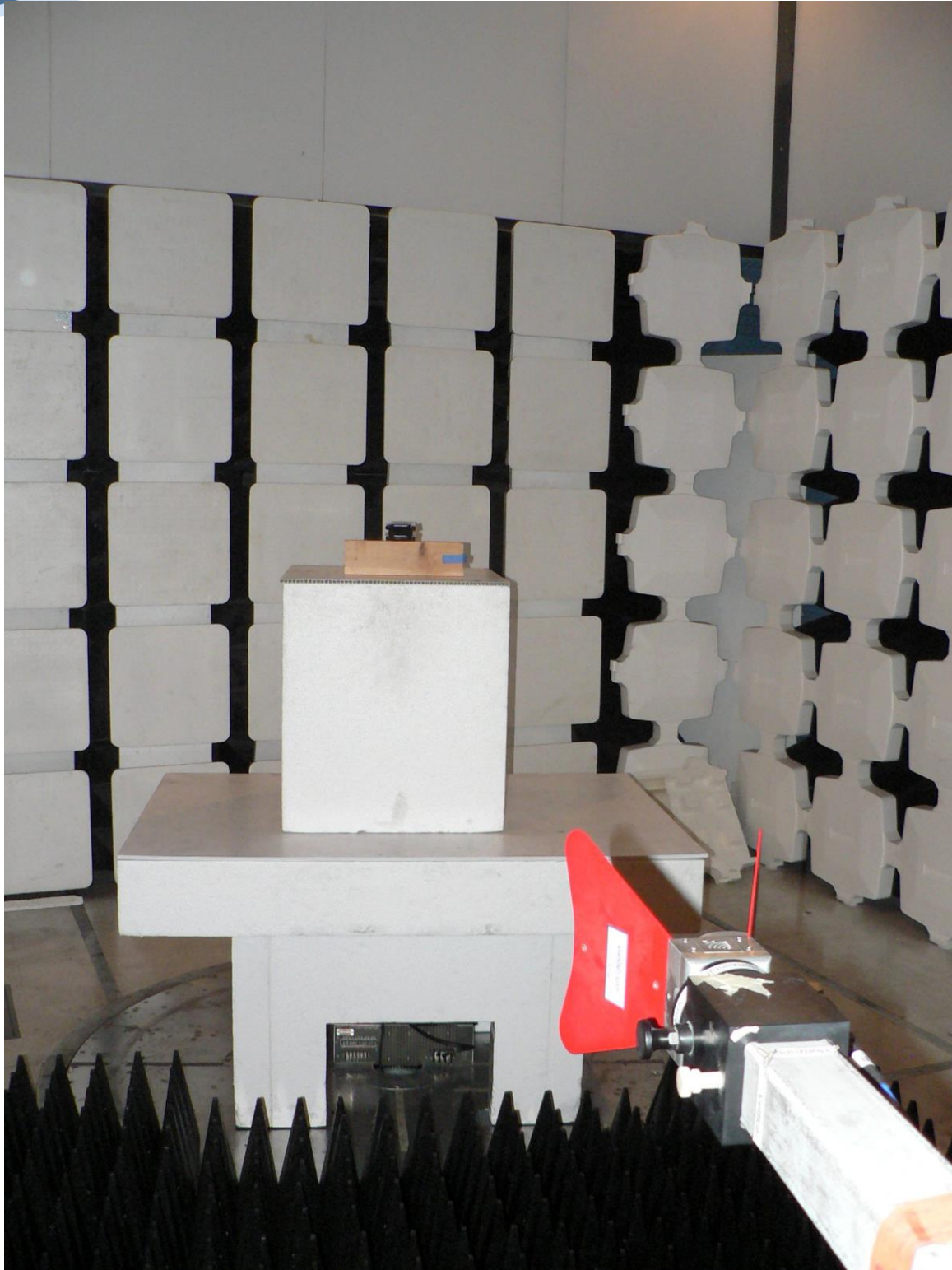
LYFT06 Tx Spurious Emissions 1-18GHz Front
