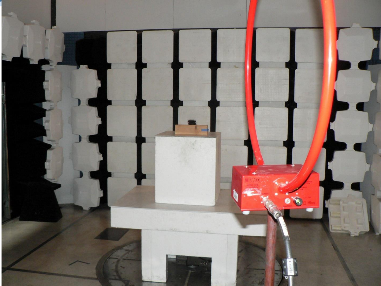
LYFT06 9k-30M Y Plane Emissions
