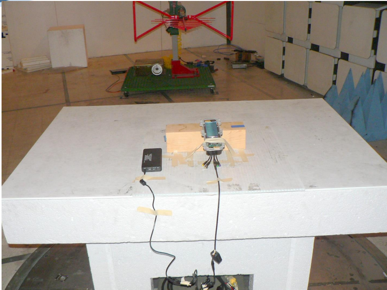
LYFT06 Digital Emissions 30-1000 MHz Back
