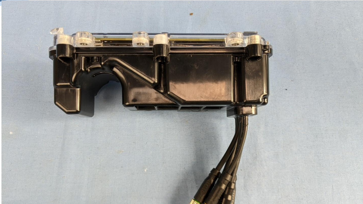
Left View
