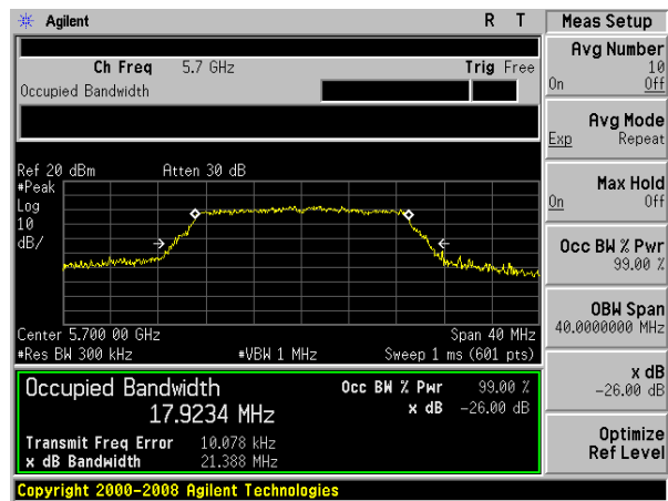
(802.11 ac20) -26dB&99%Bandwidth plot on channel 140
