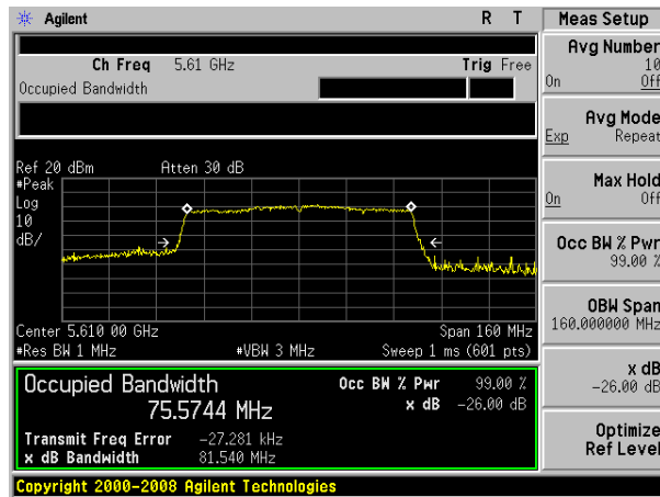
(802.11 ac80) -26dB&99%Bandwidth plot on channel 122
