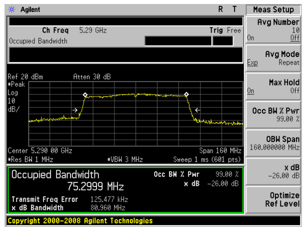
(802.11 ac80) -26dB&99%Bandwidth plot on channel 58
