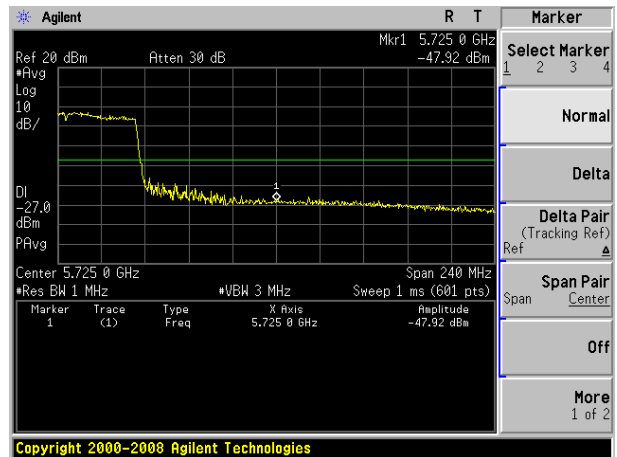
(802.11n80) Band Edge, Right Side
