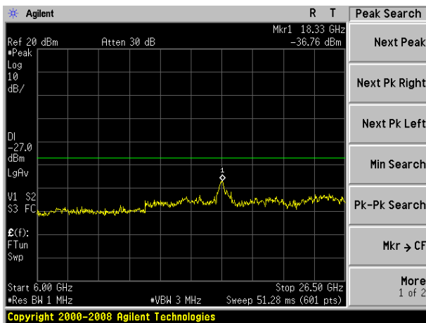
802.11ac80 on channel 122
