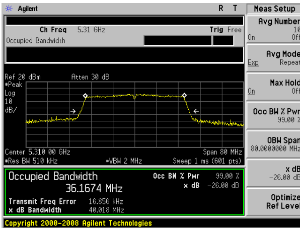
(802.11 n40) -26dB&99%Bandwidth plot on channel 62
