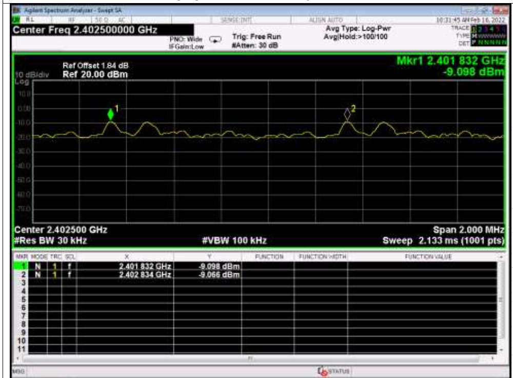
CFS NVNT 2-DH1 2402MHz
