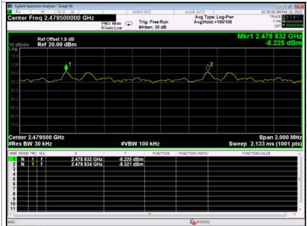
CFS NVNT 2-DH1 2480MHz
