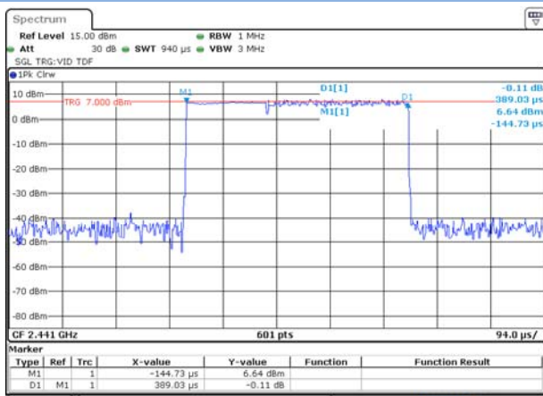
8-DPSK DH1
