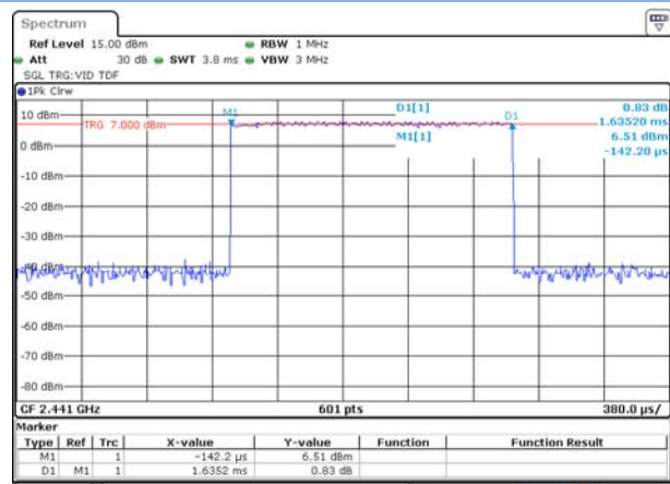
8-DPSK DH3
