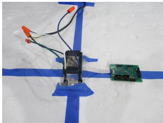
X-Axis Orientation
