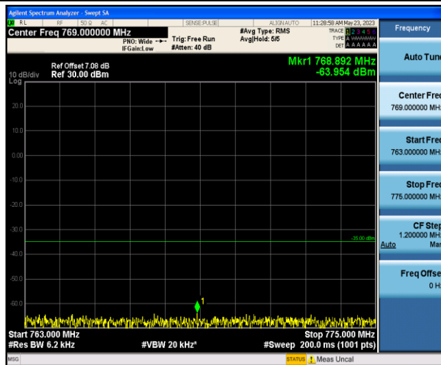
Band13-Stand-Alone-NaN-QPSK-23230-1 @0-15kHz-763-775--63.95--35-PASS
