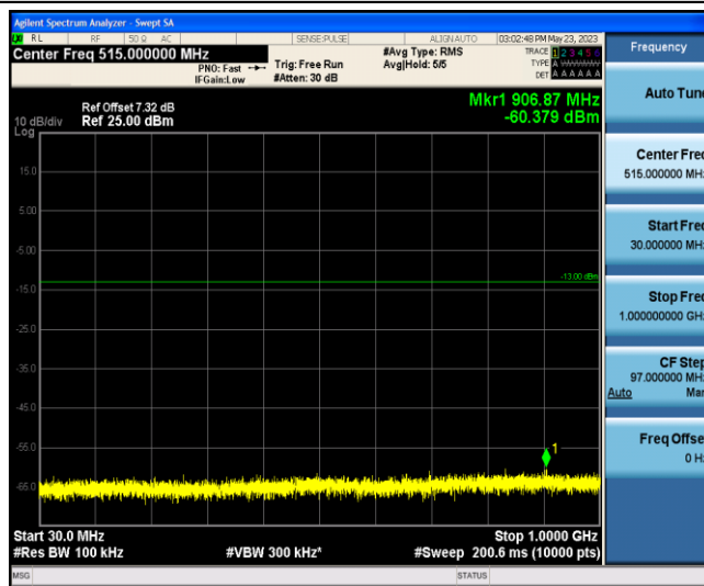
Band2-Stand-Alone-NaN-BPSK-19199-1 @0-15kHz-30-1000--60.38--13-PASS
