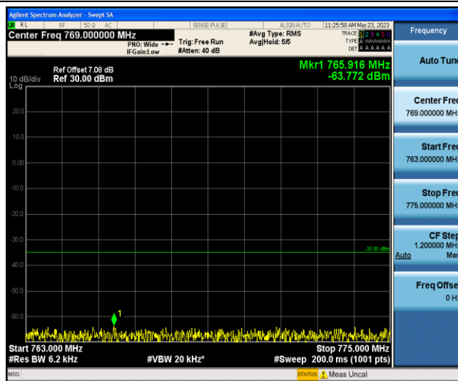
Band13-Stand-Alone-NaN-BPSK-23181-1 @0-15kHz-763-775--63.77--35-PASS
