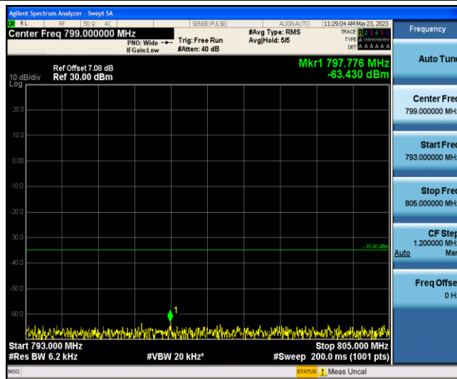
Band13-Stand-Alone-NaN-QPSK-23230-1 @0-15kHz-793-805--63.43--35-PASS
