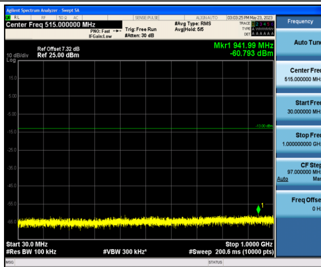
Band2-Stand-Alone-NaN-QPSK-19199-1 @0-15kHz-30-1000--60.79--13-PASS
