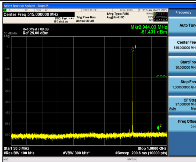
Band13-Stand-Alone-NaN-QPSK-23279-1 @0-15kHz-30-1000--61.4--13-PASS
