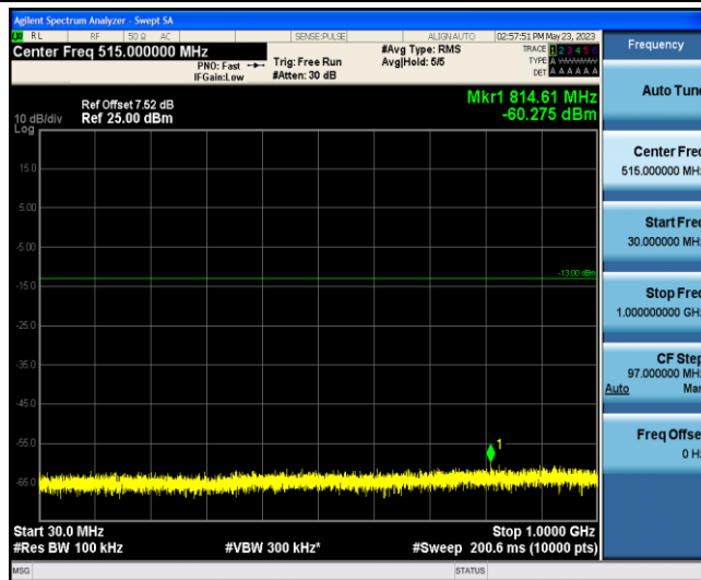
Band2-Stand-Alone-NaN-BPSK-18900-1 @0-3.75kHz-30-1000--60.28--13-PASS
