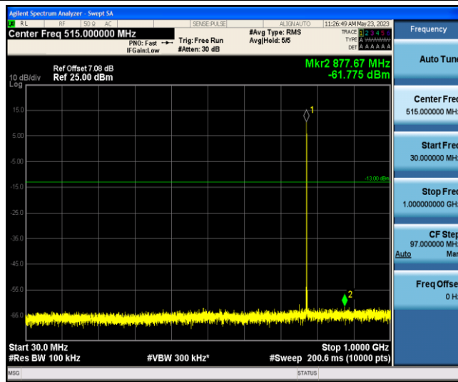
Band13-Stand-Alone-NaN-QPSK-23181-1 @0-15kHz-30-1000--61.78--13-PASS
