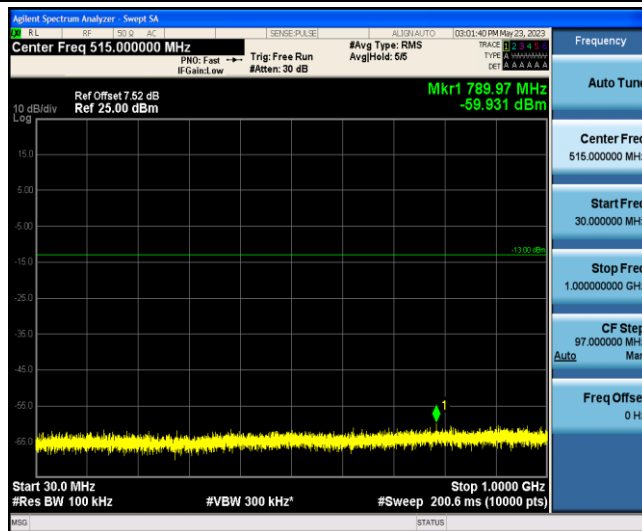
Band2-Stand-Alone-NaN-BPSK-18900-1 @0-15kHz-30-1000--59.93--13-PASS
