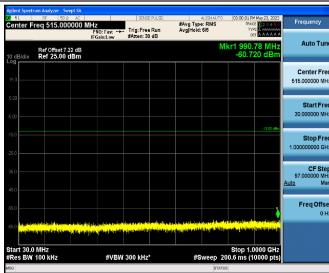
Band2-Stand-Alone-NaN-QPSK-19199-1 @0-3.75kHz-30-1000--60.72--13-PASS
