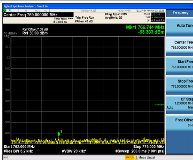
Band13-Stand-Alone-NaN-BPSK-23230-1 @0-15kHz-763-775--63.38--35-PASS
