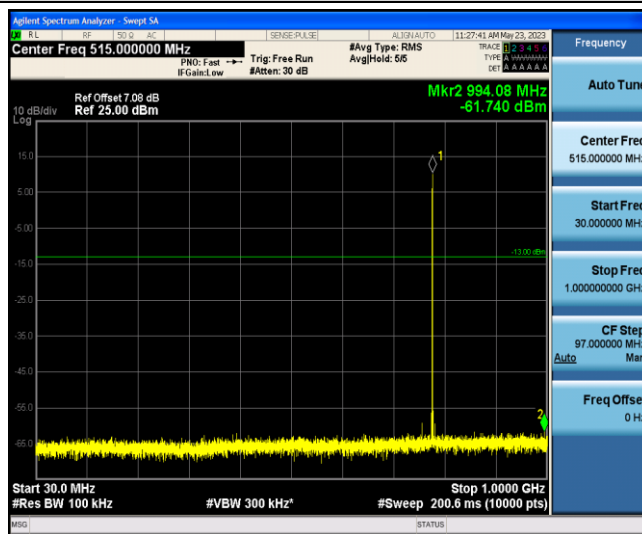
Band13-Stand-Alone-NaN-BPSK-23230-1 @0-15kHz-30-1000--61.74--13-PASS
