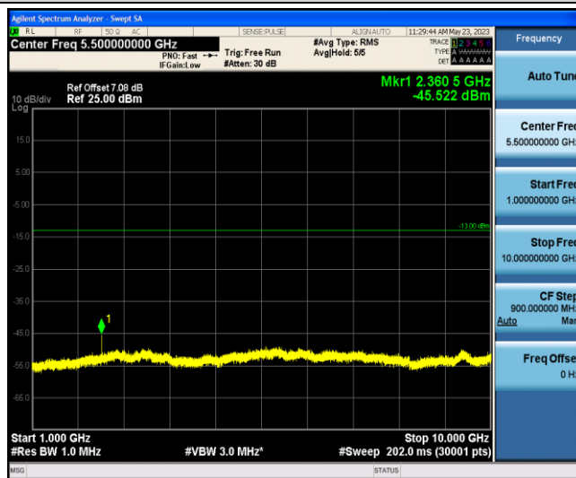
Band13-Stand-Alone-NaN-BPSK-23279-1 @0-15kHz-1000-10000--45.52--13-PASS
