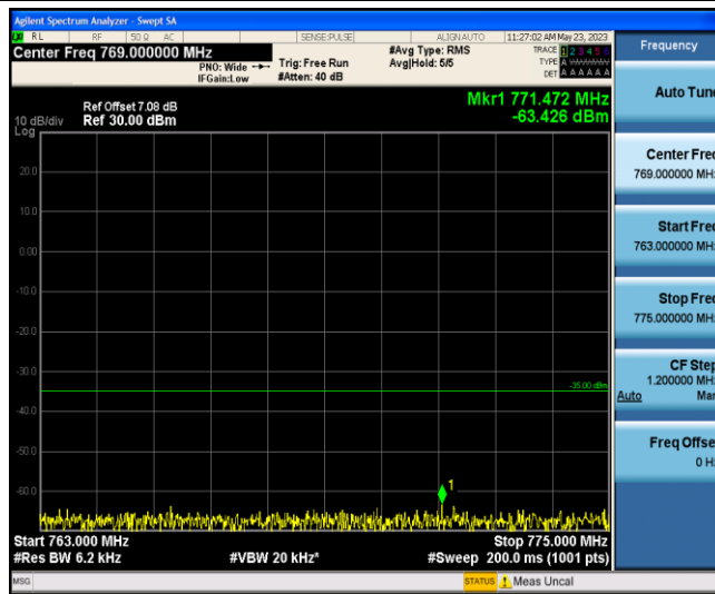
Band13-Stand-Alone-NaN-QPSK-23181-1 @0-15kHz-763-775--63.43--35-PASS
