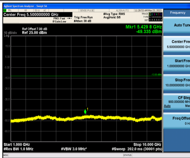
Band13-Stand-Alone-NaN-QPSK-23230-1 @0-15kHz-1000-10000--49.34--13-PASS
