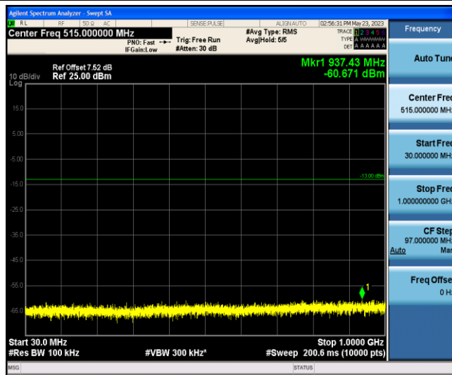
Band2-Stand-Alone-NaN-BPSK-18601-1 @0-3.75kHz-30-1000--60.67--13-PASS
