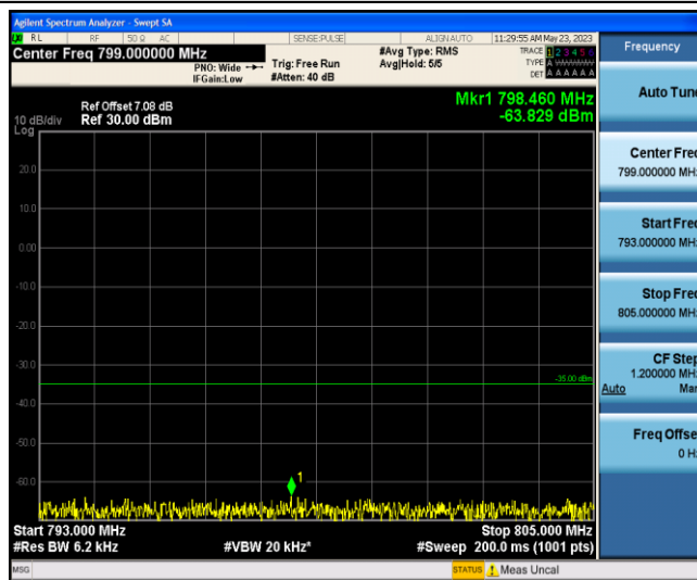
Band13-Stand-Alone-NaN-BPSK-23279-1 @0-15kHz-793-805--63.83--35-PASS
