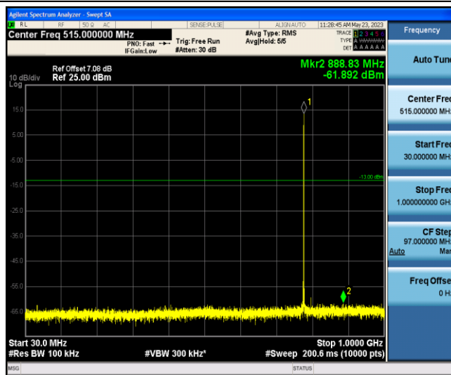
Band13-Stand-Alone-NaN-QPSK-23230-1 @0-15kHz-30-1000--61.89--13-PASS
