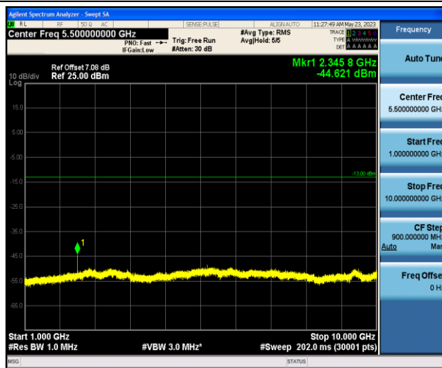
Band13-Stand-Alone-NaN-BPSK-23230-1 @0-15kHz-1000-10000--44.62--13-PASS
