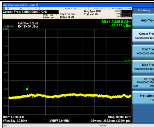
Band13-Stand-Alone-NaN-QPSK-23230-1 @0-3.75kHz-1000-1000--47.78--13-PASS
