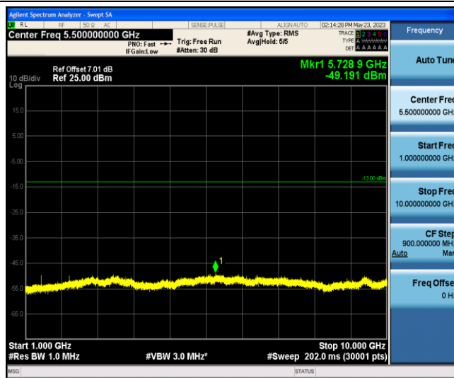
Band12-Stand-Alone-NaN-QPSK-23011-1 @0-15kHz-1000-10000--49.19--13-PASS
