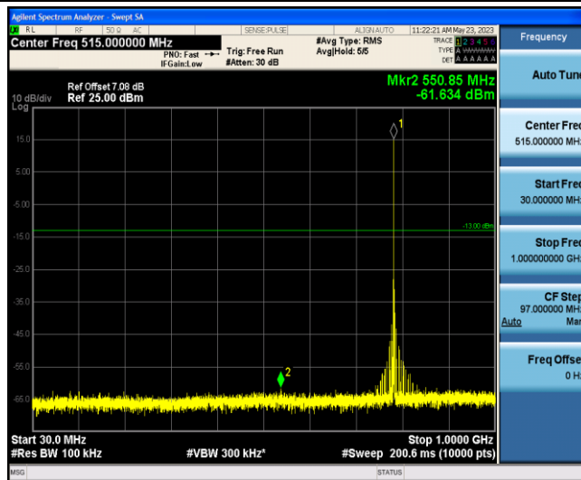
Band13-Stand-Alone-NaN-BPSK-23279-1 @0-3.75kHz-30-1000--61.63--13-PASS
