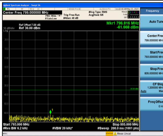
Band13-Stand-Alone-NaN-BPSK-23279-1 @0-3.75kHz-793-805--61.67--35-PASS
