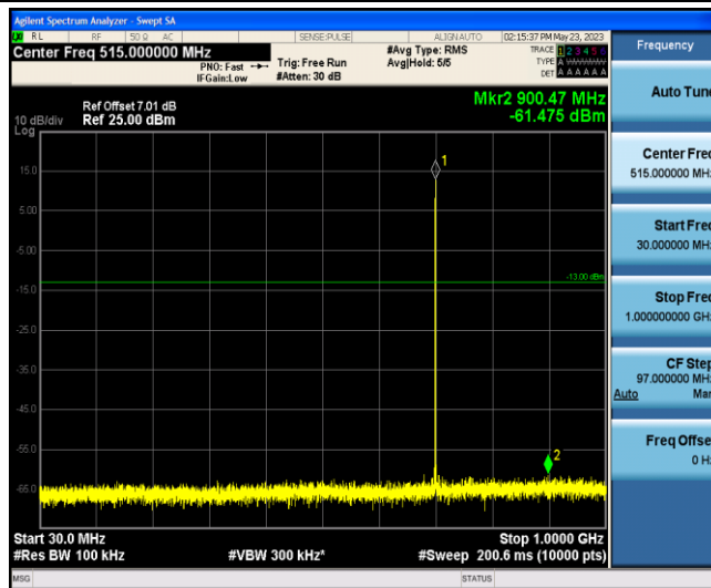
Band12-Stand-Alone-NaN-QPSK-23095-1 @0-15kHz-30-1000--61.48--13-PASS
