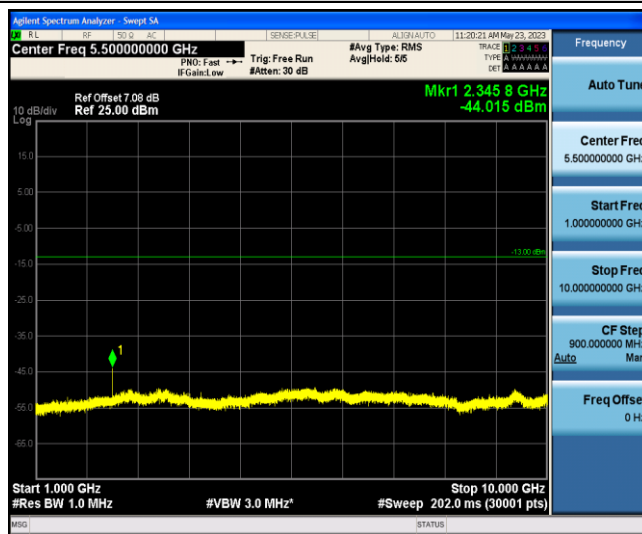
Band13-Stand-Alone-NaN-BPSK-23230-1 @0-3.75kHz-1000-1000--44.02--13-PASS
