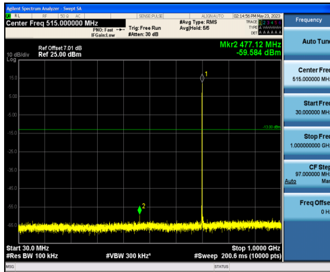
Band12-Stand-Alone-NaN-BPSK-23095-1 @0-15kHz-30-1000--59.58--13-PASS
