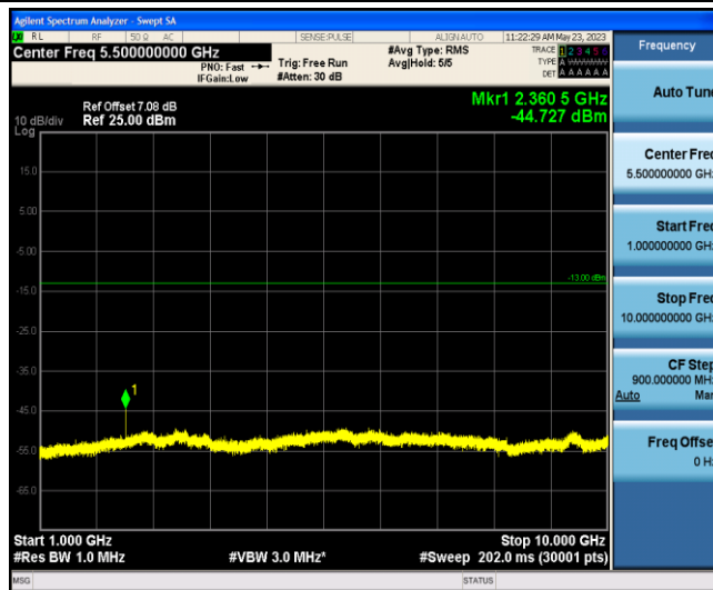
Band13-Stand-Alone-NaN-BPSK-23279-1 @0-3.75kHz-1000-10000--44.73--13-PASS
