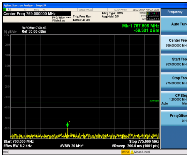
Band13-Stand-Alone-NaN-BPSK-23279-1 @0-3.75kHz-763-775--59.3--35-PASS
