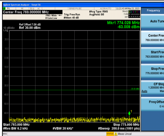
Band13-Stand-Alone-NaN-QPSK-23230-1 @0-3.75kHz-763-775--63.01--35-PASS
