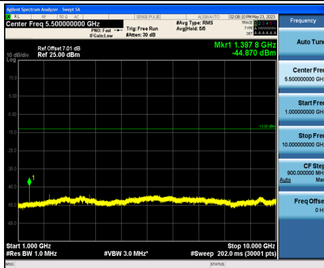
Band12-Stand-Alone-NaN-BPSK-23011-1 @0-3.75kHz-1000-10000--44.87--13-PASS
