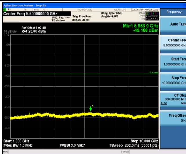
Band12-Stand-Alone-NaN-QPSK-23179-1 @0-3.75kHz-1000-10000--49.19--13-PASS
