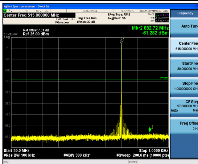
Band12-Stand-Alone-NaN-BPSK-23095-1 @0-3.75kHz-30-1000--61.28--13-PASS
