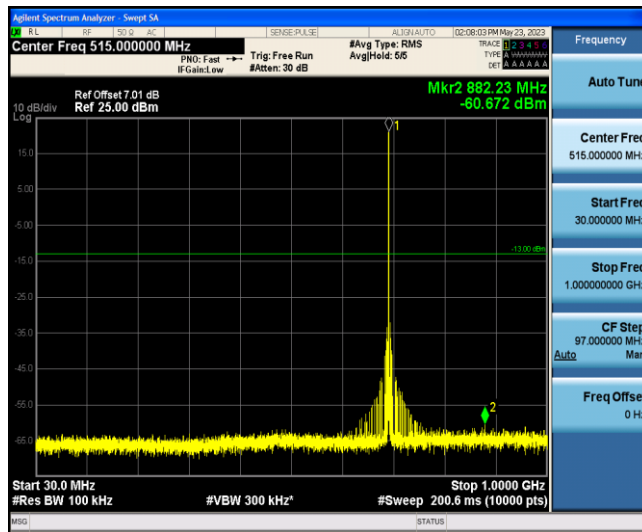
Band12-Stand-Alone-NaN-BPSK-23011-1 @0-3.75kHz-30-1000--60.67--13-PASS
