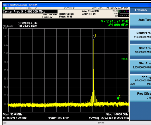
Band12-Stand-Alone-NaN-QPSK-23179-1 @0-3.75kHz-30-1000--61.1--13-PASS
