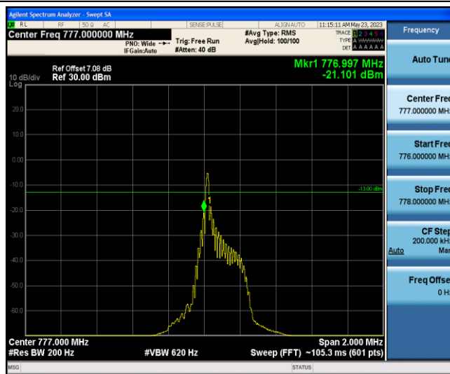
Band13-Stand-Alone-NaN-QPSK-23181-1 @0-15kHz--20.95-PASS
