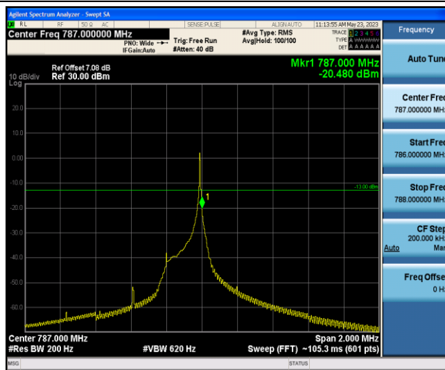
Band13-Stand-Alone-NaN-QPSK-23279-1 @47-3.75kHz--20.42-PASS
