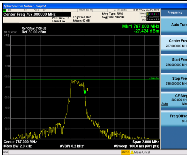
Band13-Stand-Alone-NaN-QPSK-23279-12 @ 0-15kHz--27.42-PASS
