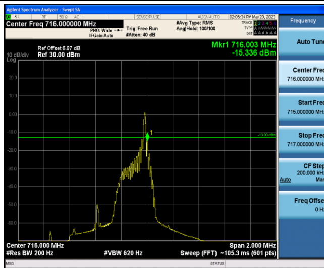
Band12-Stand-Alone-NaN-QPSK-23179-1 @11-15kHz--15.33-PASS
