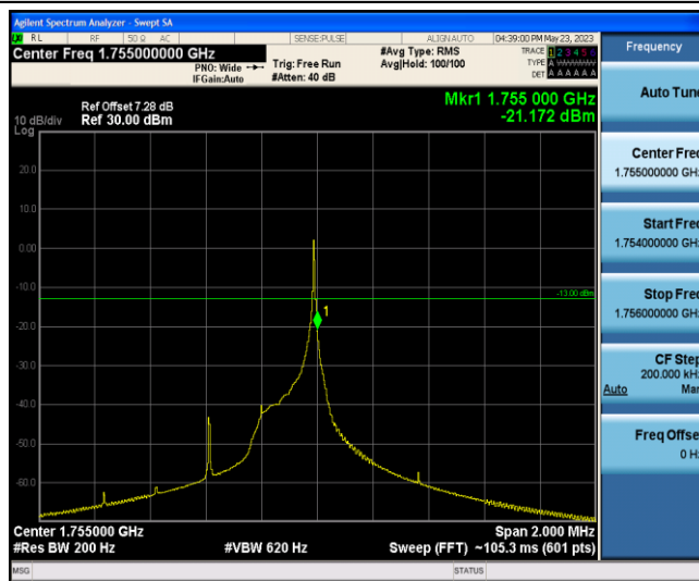
Band4-Stand-Alone-NaN-BPSK-20399-1 @47-3.75kHz--21.17-PASS
