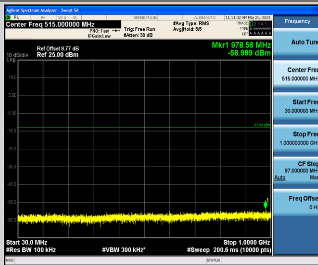
Band66-1.4MHz-16QAM-131979-1-0-Low-30-1000--58.99-PASS
