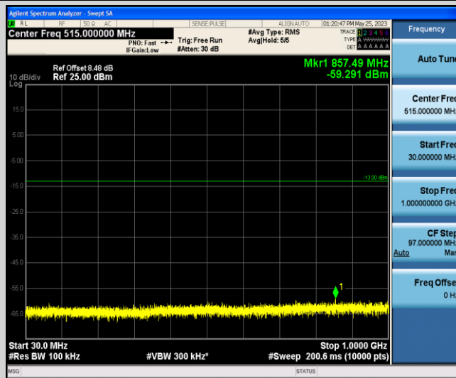
Band4-20MHz-16QAM-20175-1-0-Low-30-1000--59.29-PASS
