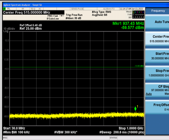
Band66-3MHz-16QAM-132657-1-0-Low-30-1000--59.58-PASS
