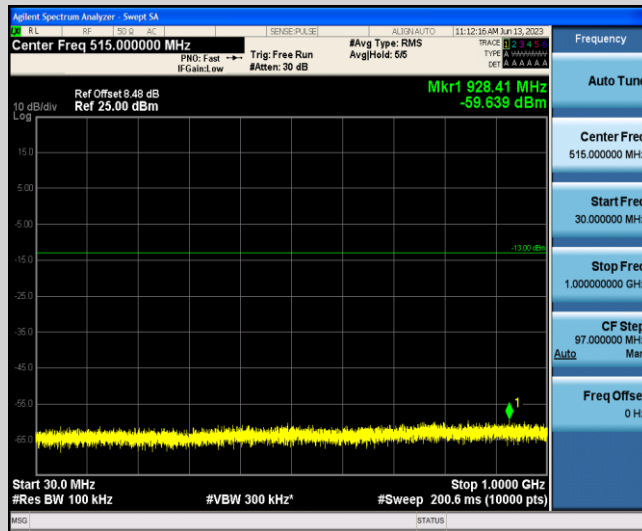
Band66-1.4MHz-16QAM-132665-1-0-Low-30-1000--59.64-PASS
