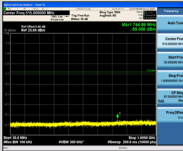
Band4-20MHz-16QAM-20300-1-0-High-30-1000--59.06-PASS
