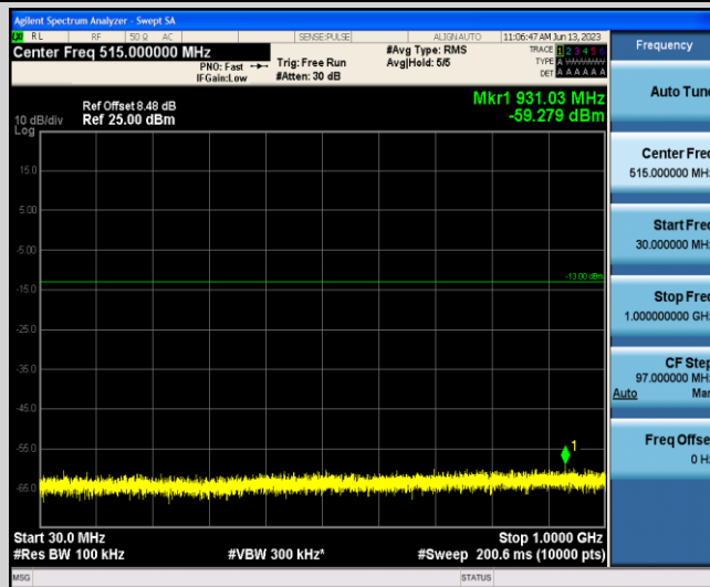
Band4-20MHz-1RB#0@Low-20300-1-0-High-30-1000--59.28-PASS
